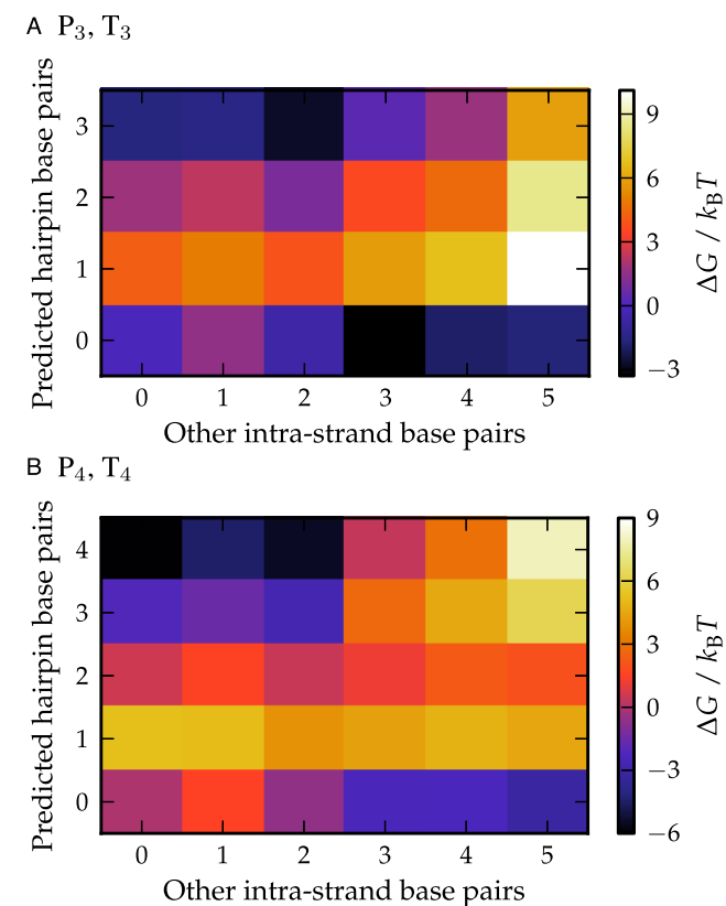
Figure 3. The free-energy profiles of the P_3 and P_4 strands are shown in panels (A) and (B), respectively. The free energy of a particular state relative to the unbound (0,0) state is indicated by the color of the square. The results for complementary T strands are essentially identical.
