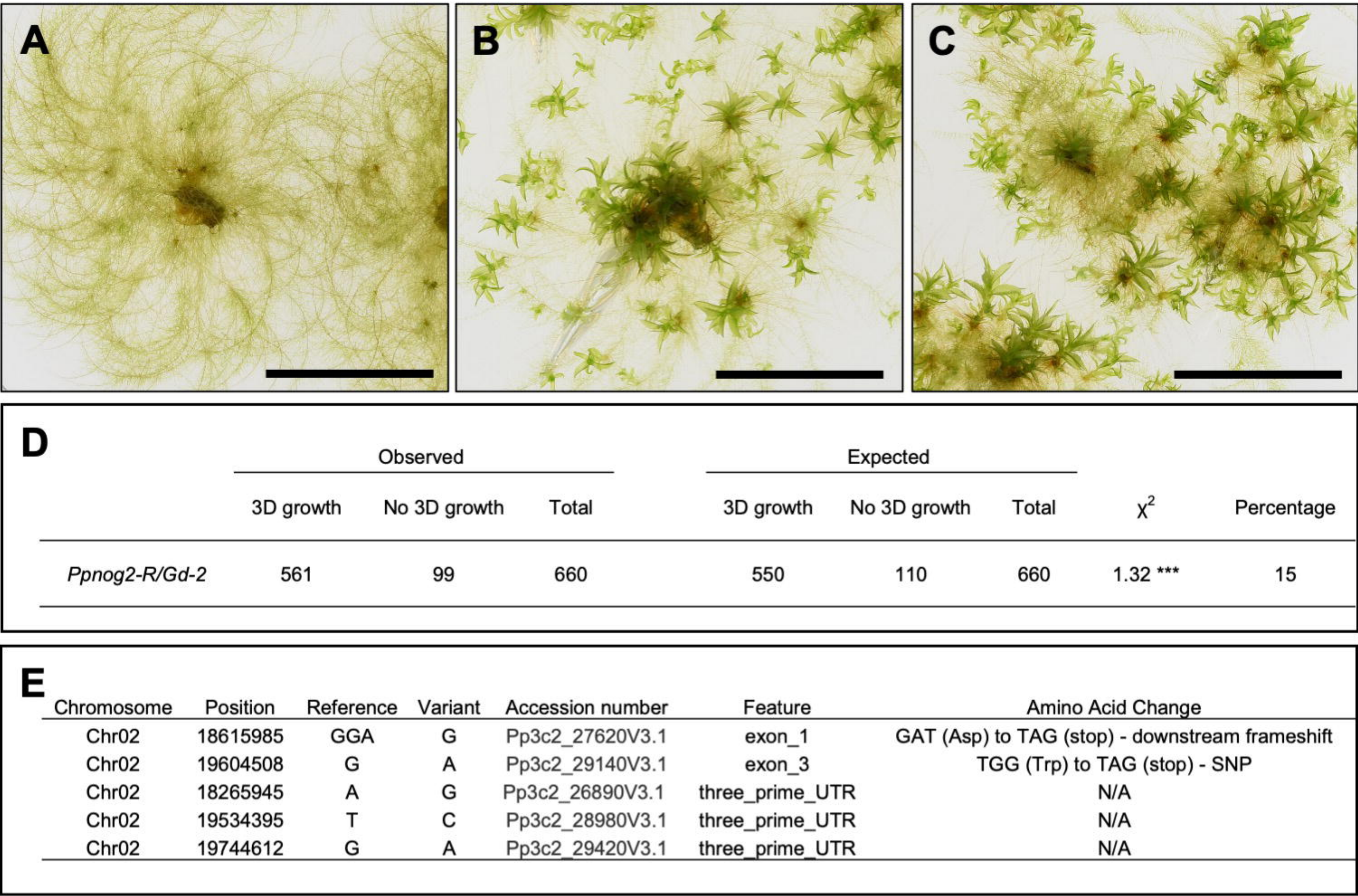
Figure 3. Identification of the PpNOG2 locus by somatic hybridization combined with bulk segregant analysis
