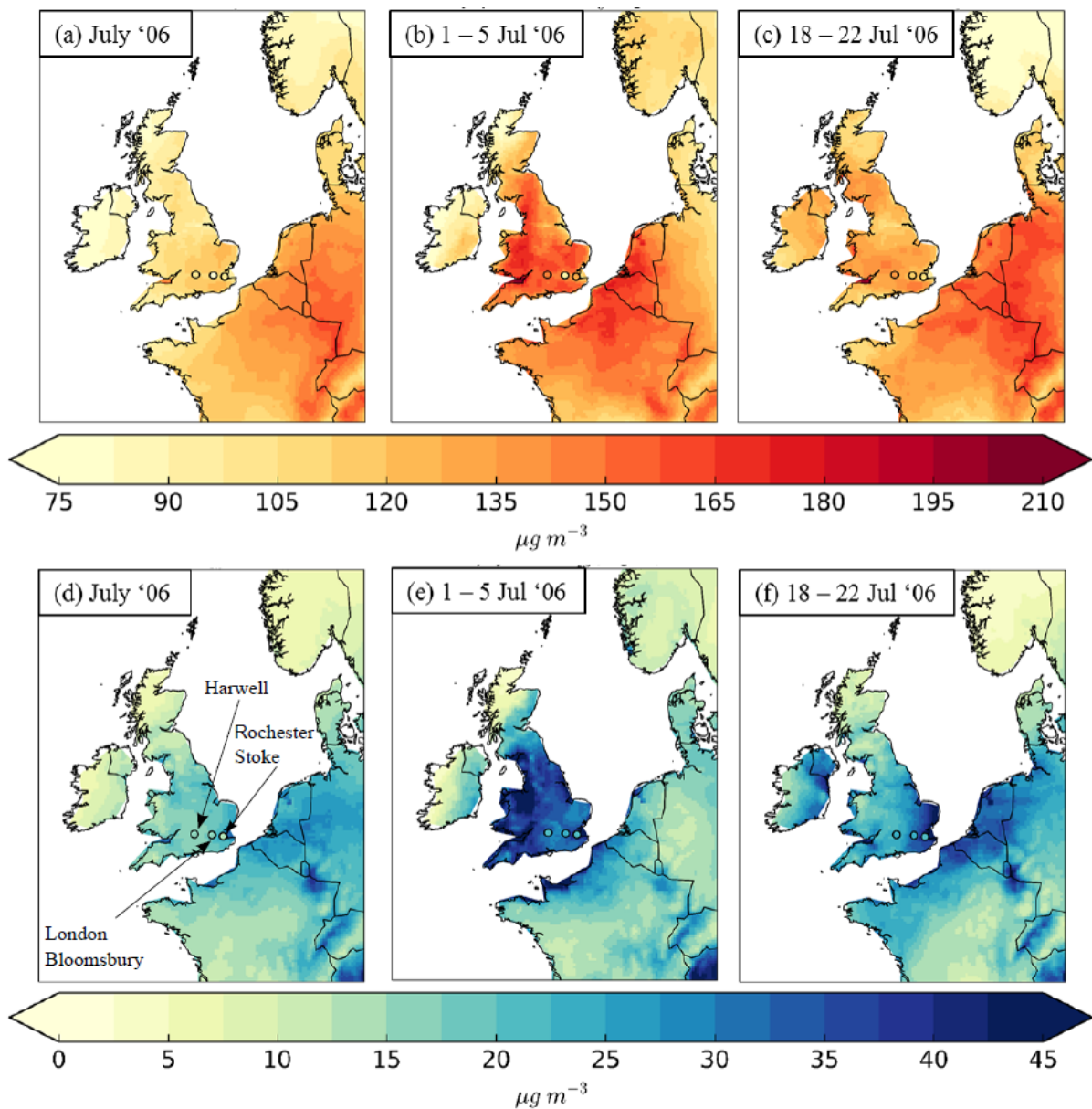
Figure 4: Simulated daily maximum 8-hr running mean O 3 concentrations for (a) July mean, (b) 1-5 July mean and (c) 18-22 July 2006 mean and simulated daily mean PM 2.5 concentrations for the same time periods (d, e and f) (NB concentrations shown here are not bias corrected to enable comparison with meteorology; however spatial patterns are similar (refer to Supplement)). The circles in each plot are coloured with measured data of the respective pollutant at 3 AURN sites - Rochester Stoke, Harwell and London Bloomsbury.
