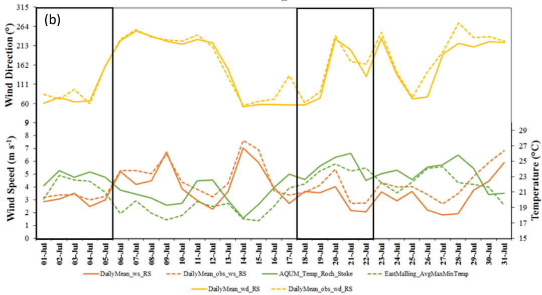
Figure 3: Daily time series during July 2006 of modelled (solid lines) and observed (dashed lines) a) PM_{2.5} (blue) and MDA8 O_3 (red) b) wind direction (degrees are taken clockwise starting from the north - yellow), wind speed (orange) and temperature (green) at the rural background AURN station in Rochester Stoke (observed temperatures were obtained from the nearest MIDAS station to Rochester Stoke which is at East Malling.) Black boxes represent the two 5-day air pollution episodes in July 2006 (1 st -5 th July and 18 th -22 nd July). Solid lines with dots indicated the original simulated concentrations while the solid lines with no dots show the bias-corrected concentrations using the SPPO technique.
