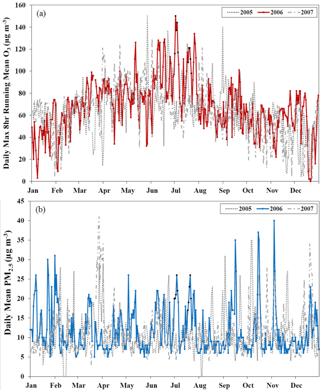
Figure 2: (a) Daily maximum 8-hr running mean (MDA8) O_3 and (b) daily mean PM_{2.5} at the Rochester Stoke AURN rural background station from 2005 (dotted), 2006 (red for O_3 and blue for PM_{2.5} ), and 2007 (dot-dashed). Black points mark the two 5-day air pollution episode days for July 2006 (1 st -5 th July and 18 th -22 nd July 2006).
