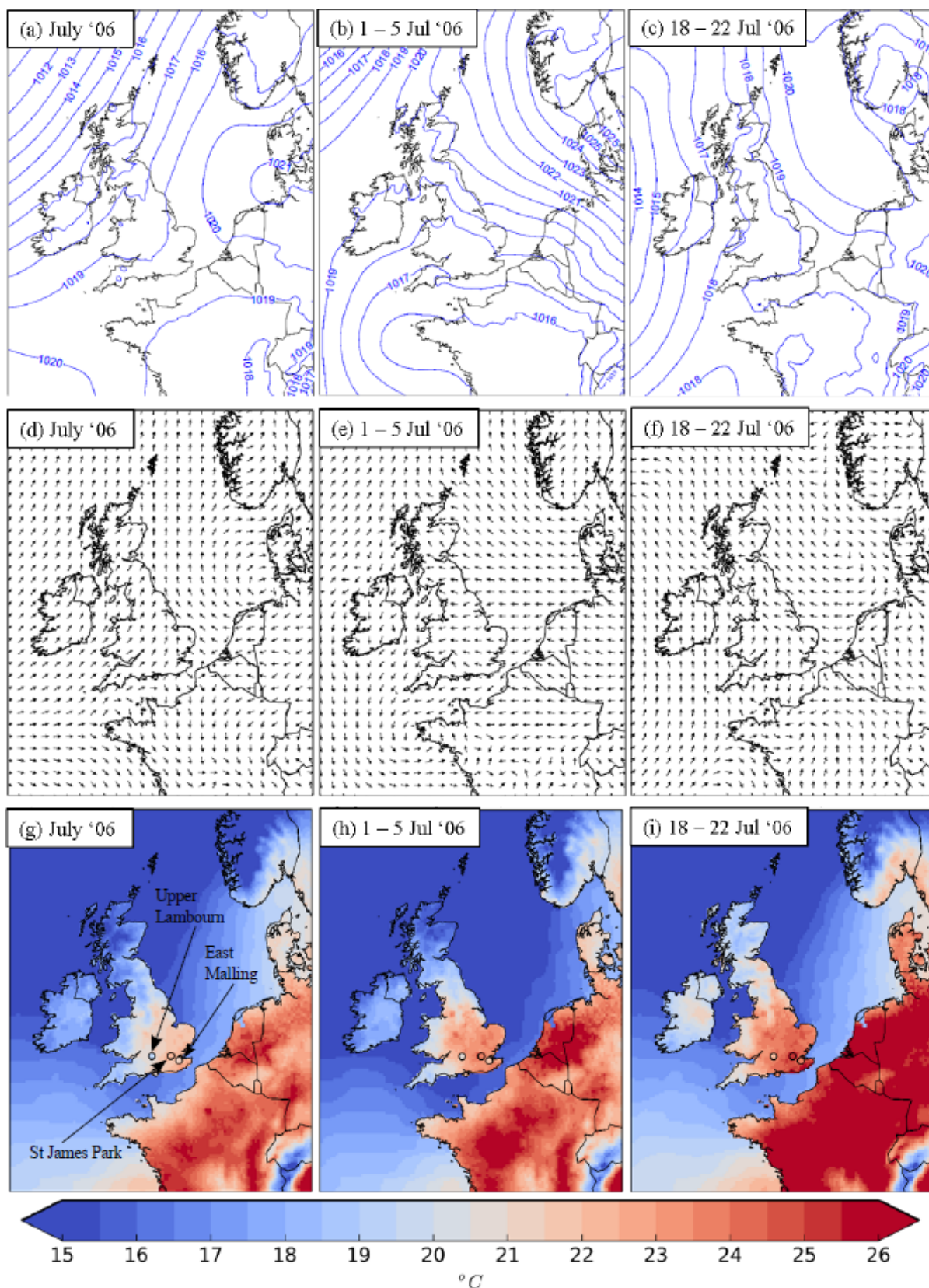
Figure 6: Daily mean air pressure at mean sea level (top panel), wind vectors (middle panel) and surface temperature (bottom panel) averaged for all of July (left column), 1 st to 5 th July (middle column) and 18 th to 22 nd July (right column). Measured levels of daily mean temperature averaged for the same time periods from three MIDAS stations (St James Park, East Malling and Upper Lambourn) are shown in coloured circles (bottom panel)
