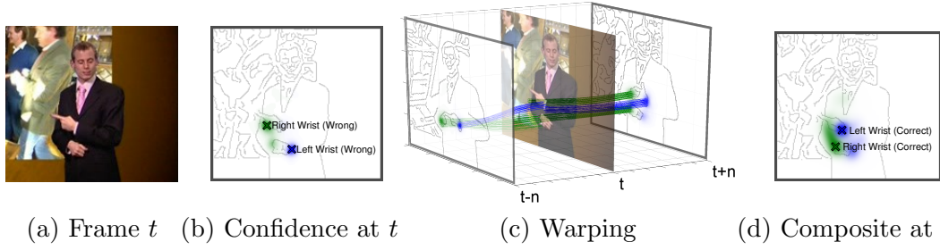
Figure 5.10: Warping neighbouring confidence maps for improving pose estimates. (a) RGB input at frame t . (b) Confidence map at frame t for left (blue) and right (green) hands (crosses show incorrect modes of confidence). (c) Confidence maps from frames (t - n) and (t + n) warped to frame t using tracks from optical flow (green & blue lines). (d) Composite map with corrected modes.
