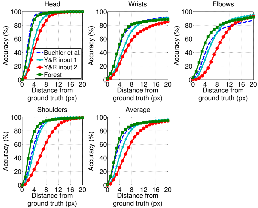
Figure 4.14: Comparison of joint tracking accuracy of random forest against [Buehler et al., 2011] and [Yang and Ramanan, 2011]. Plots show accuracy per joint type (averaged over left and right body parts) as allowed distance from manual ground truth is increased.
