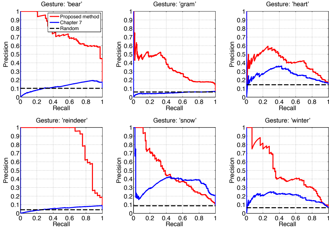
Figure 8.6: Gesture spotting accuracy on the gesture reservoir for BSL-TV , with a comparison to Chapter 7. PR curves are for six gestures with ground truth.
