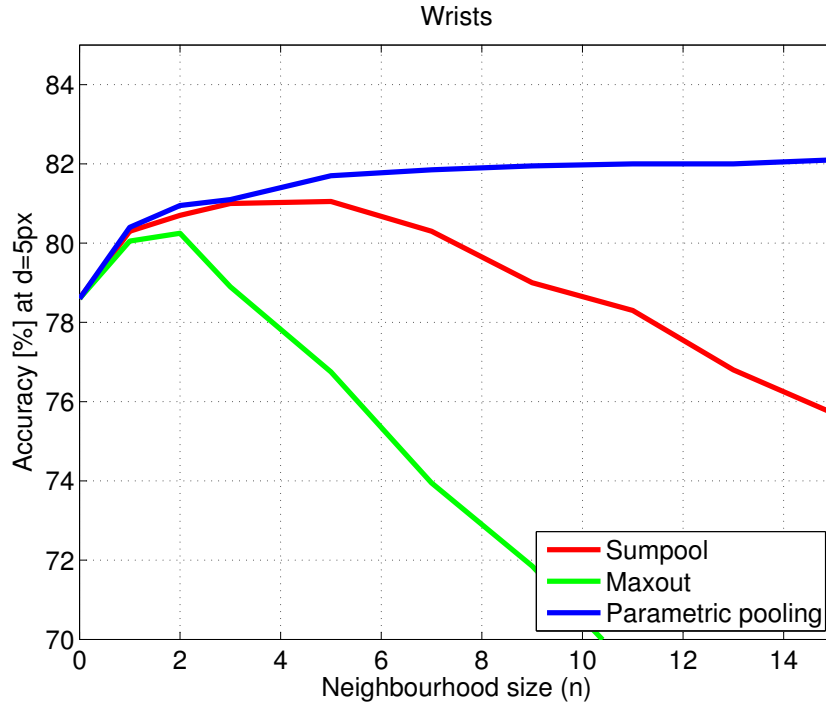
Figure 6.11: Comparison of pooling types. Results are shown for wrists in BBC Pose at threshold d = 5 px. Parametric pooling (learnt cross-channel pooling weights) performs best.
