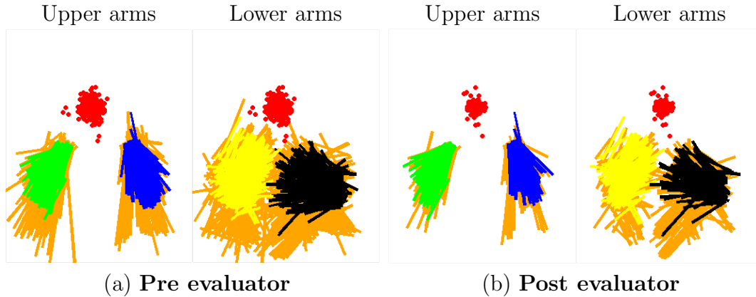
Figure 4.18: Pose visualisation with/without evaluator. (a) shows scatter plots of stickmen for pose estimates from forest on all training data. (b) shows scatter plot of pose estimates from forest on training data marked as containing good poses by the evaluator. Elbow and wrist joints greater than 5px from ground truth are indicated by orange sticks.
