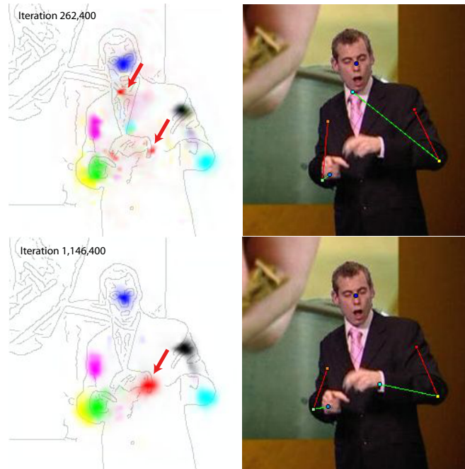
Figure 6.6: Multiple peaks are possible with the Spatial Heatmap ConvNet. Early on in training (top), multiple locations may fire for a given joint. These are then suppressed as training proceeds (bottom). The arrows identify two modes for the wrist; one correct, one erroneous. As the training proceeds the erroneous one is diminished.
