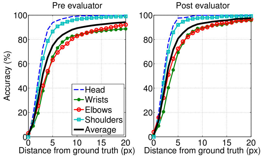
Figure 4.17: Pose estimation with/without evaluator. Average accuracy of per-joint estimates are shown without (left) and with (right) evaluator when the operating point of the pose evaluator is set to the optimum in Figure 4.16a.
