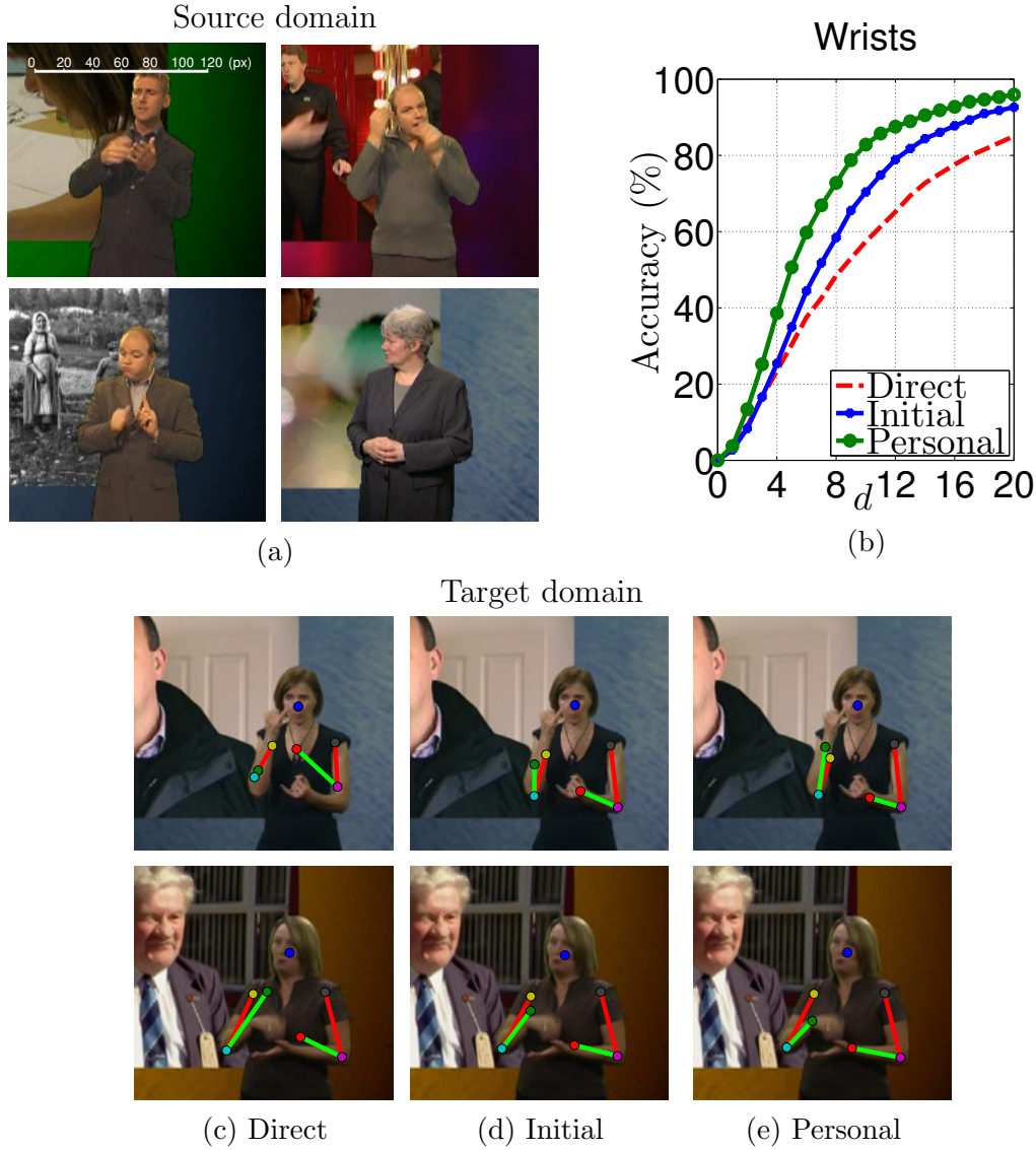
Figure 5.1: Training an upper body pose estimator using knowledge from the source domain. In this example, the transfer is from a source domain (a) where signers wear long sleeves, to a target domain (c)–(e) where signers wear short sleeves. The red and green lines on the signer show the output pose. The target domain results show: (c) the detector trained directly from the source domain; (d) trained from initial semi-synthetic images constructed using the source domain; and (e) from personal semi-synthetic images constructed from both source and target domain. (b) shows accuracy of (c)–(e) in detecting the wrist joint in the target domain. Accuracy is percentage of predicted joints within a distance d pixels from ground truth (scale bar shown in top left of (a)). The accuracy almost doubles at 8 pixels.
