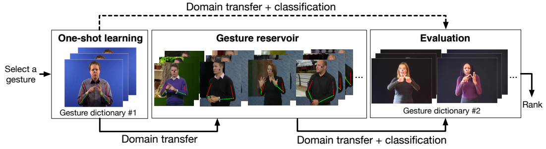
Figure 8.1: Learning gestures from strong and weak supervision. A single strongly supervised training example from a dictionary is used to train a one-shot learner . This one-shot learner is used to obtain additional training data from a large weakly supervised gesture repository of another domain. These new samples are used to ‘boost’ the one-shot learner with additional discriminative power. Evaluations are carried out under further domain adaptation on another strongly supervised dictionary dataset. Dashed line shows the baseline and the solid lines show the proposed method .
