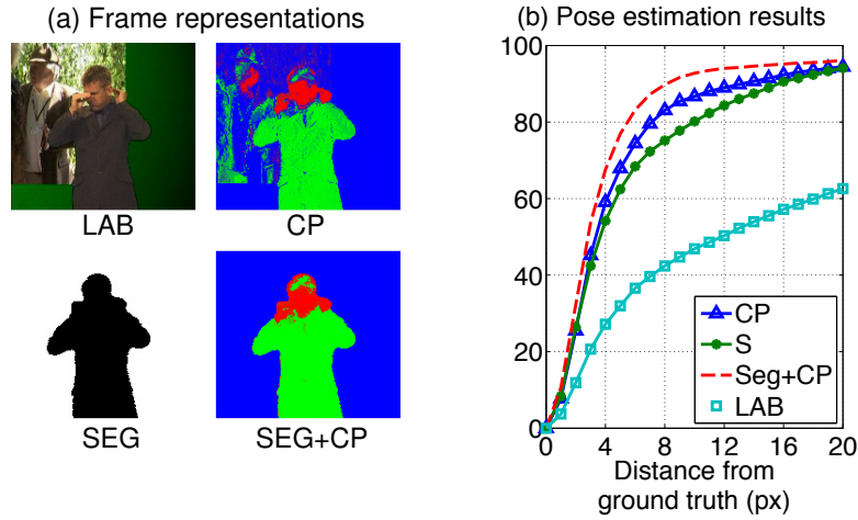
Figure 4.12: Comparison of different input frame representations. (a) Example frames showing different methods for representing a frame. (b) Average accuracy of forests as allowed distance from ground truth is increased. Using SEG+CP proves best.
