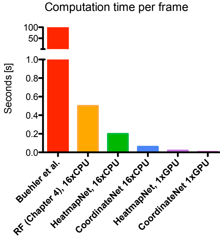
Figure 6.16: Computation time. Comparison of computation times versus the method in Chapter 4 and [Buehler et al., 2011]. Note that the reliable semi-automatic method of Buehler et al. is off the scale as computing a pose for a single frame takes around 100s. Our method outperforms previous methods by over an order of magnitude using the same hardware. Using a single GPU instead of CPUs increases speed by another order of magnitude.
