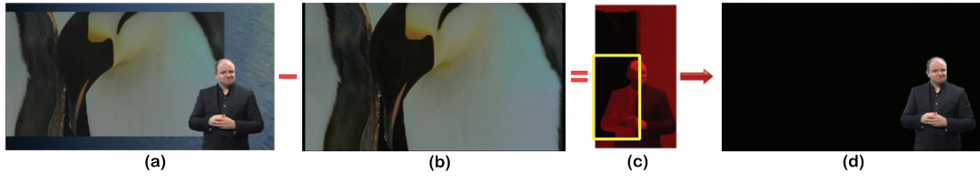
Figure 4.19: Co-segmentation using two complementary data sources. The signer-overlaid frame (a) and original frame (b) are subtracted after alignment, resulting in a difference image (c) that is used as a foreground clamp (in yellow) and to generate GrabCut constraints. (d) shows the segmentation output.
