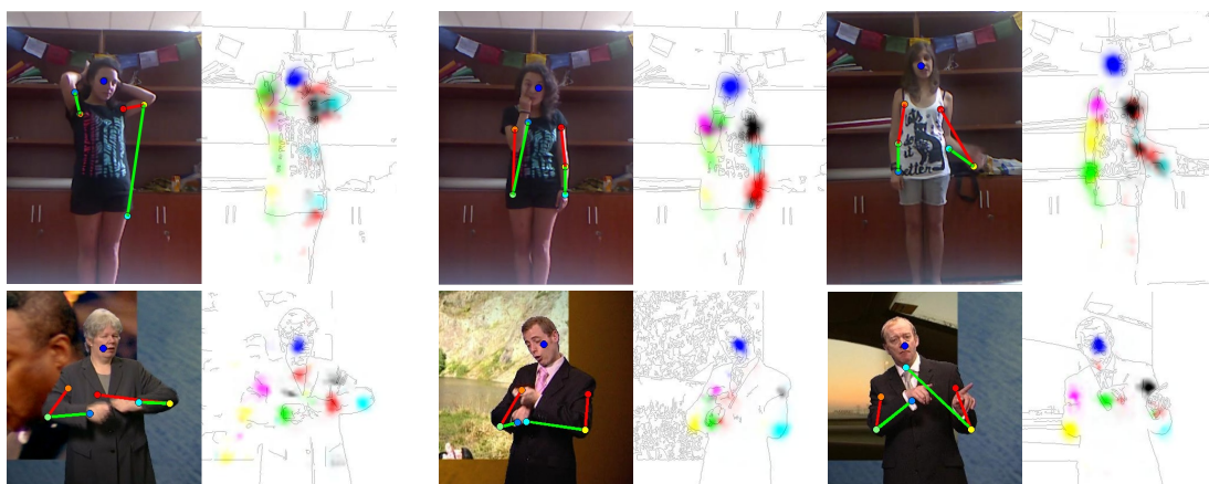
Figure 6.19: Failure cases. As shown, failure cases contain multiple modes for the same joint in the heatmap (and the wrong mode has been selected). This could be addressed with spatial model.
