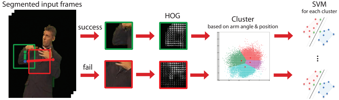
Figure 4.8: Training the detector for mixed hand predictions. The evaluator is trained on HOG feature vectors placed in the middle of the correct and incorrect positions of the lower arm. Feature vectors are clustered into separate SVMs based on the hand-elbow angle and hand position.
