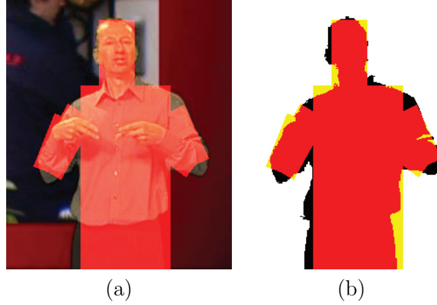
Figure 4.6: Segmentation score for evaluator. (a) the silhouette (red boxes) rendered based on estimated joint positions. (b) the segmentation (black), rendered silhouette (yellow) and their overlap (red) which is used as a segmentation score.
