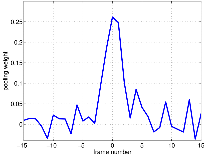
Figure 6.10: Learnt pooling weights for BBC Pose with n = 15 . Weights shown for the right wrist. The centre frame receives highest weight.
