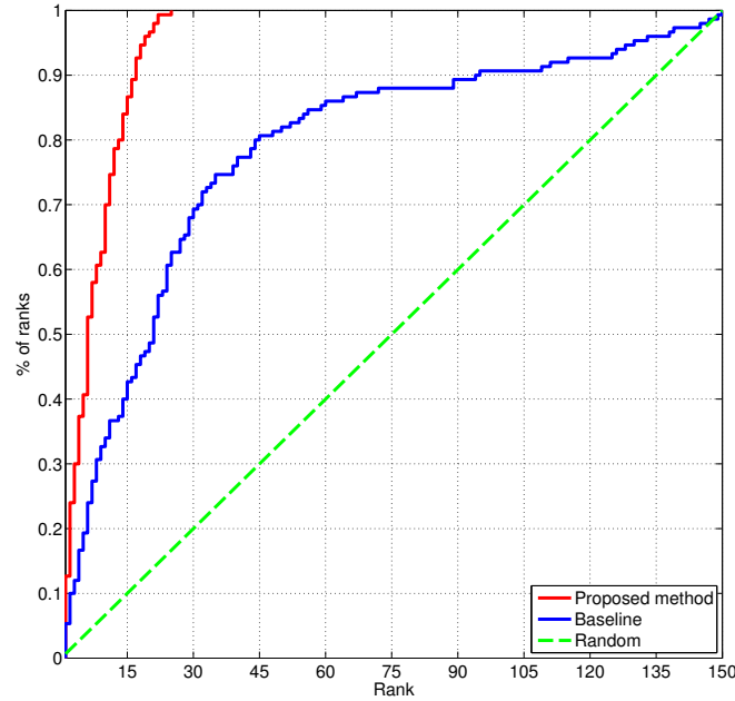
Figure 8.7: Gesture classifier accuracy evaluated on gesture dictionary ‘BSL dictionary 2’. The graph shows the recall at rank k for the baseline and our proposed method. For example, 87% of gestures are ranked within the top 15.
