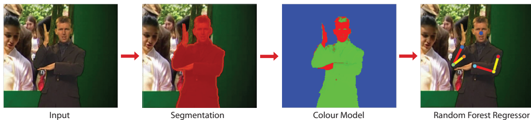
Figure 4.1: Random forest pose estimator overview. Arm and hand joint positions are predicted by first segmenting the signer using a layered foreground/background model, and then feeding the segmentation together with a colour model into a random forest regressor.
