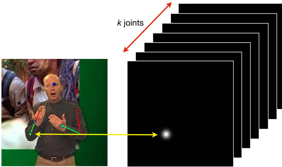
Figure 6.5: Regression target for learning the Heatmap ConvNet. The learning target for the convolutional network is (for each k joints) a heatmap with a synthesised Gaussian with a fixed variance centred at the ground truth joint position. The loss is the l_2 loss between this target and the output of the last convolutional layer.
