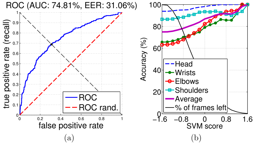
Figure 4.16: Pose evaluator classification performance. (a) ROC curve of the evaluator. (b) Change in accuracy as a function of the percentage of frames left after discarding frames that the evaluator detects as failures. For (b) the accuracy threshold is set as 5 pixels from manual ground truth.
