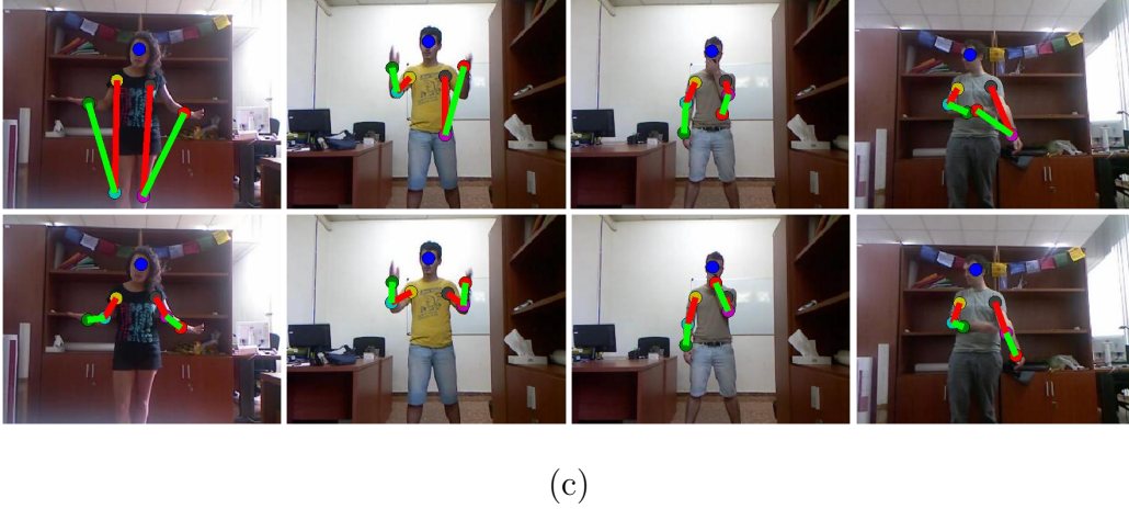
Figure 5.8: Sequential forest performance on the ChaLearn dataset. (a) & (b) show average accuracy for wrists and elbows (against allowed distance from ground truth (Kinect provided skeleton) in pixels). Sequential forests (SF) show a significant improvement for wrist detections over Chapter 4, and nearly double the accuracy for the elbows at 5 pixels from ground truth. (c) Example pose estimates on ChaLearn for the forest in Chapter 4 (top row) and SF (bottom row).
