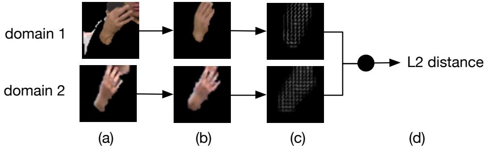
Figure 8.5: Hand shape descriptor. (a) Badly segmented hands (due to overlap with skin) in two domains, (b) hands assigned to their hand cluster exemplars, (c) HOG of size-normalised exemplars, and (d) hands are compared across domains in terms of l_2 distance between the HOGs of the hand exemplars.
