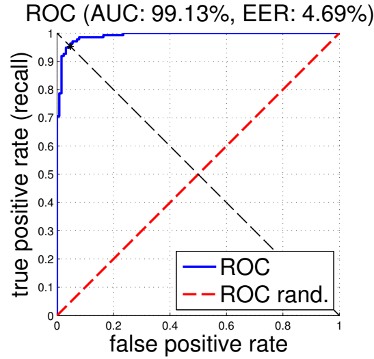
Figure 7.3: ROC curve of the person-independent mouthing classifier.
