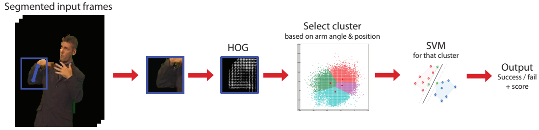
Figure 4.9: Testing the hand mixup detector. The SVM trained on a cluster whose centroid best represents the predicted joints is chosen to evaluate the HOG feature vector placed in the middle of the hand and elbow positions. This SVM outputs a failure score which the evaluator exploits as a feature for predicting whether the pose estimate is successful or failed.
