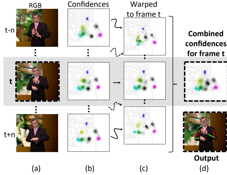
Figure 5.9: Process diagram of temporal upper body pose estimation on RGB input frame t . Detection reinforcement with optical flow for a person's right arm is shown running from left to right. (a) Given the head position, joints are detected using the sequential forest from Section 5.2. (b) Joint detections produce a body joint confidence map (different colour per joint) shown superimposed on an edge image. (c) Confidences at frame t are reinforced by combining warped confidences (using optical flow) from n frames either side of t . (d) Body joint estimates are chosen as points of maximum confidence from the combined confidence map, with final pose output illustrated with a skeleton on RGB frame t .
