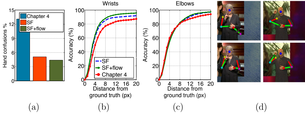
Figure 5.12: Performance of sequential forests + optical flow on BBC TV dataset. (a) Bar chart showing percentage of hand confusions (lower is better) – SF+flow does best; (b) & (c) accuracy of average wrist and elbows joints respectively (averaged of left and right arms) against allowed pixel distance from ground truth (higher is better) – SF+flow increases accuracy by 15% for wrists compared to Chapter 4 (at 5 pixels); (d) shows SF+flow (bottom row) correcting incorrect pose estimates from Chapter 4 (top row).
