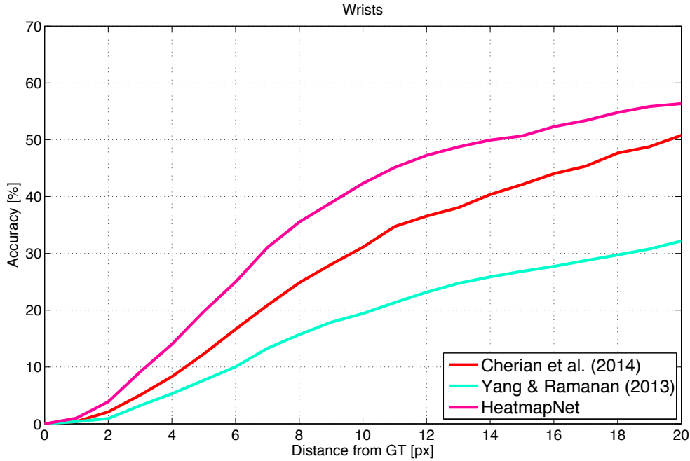
Figure 6.14: Comparison to state of the art on Poses in the Wild. Plot shows accuracy for wrists as the allowed distance from manual ground truth is increased. We note that our method outperform state of the art by a large margin (12% at d = 10 ).
