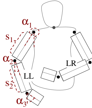
Figure 2.4: Upper body model in [Buehler et al., 2011]. The pose is specified by 11 parameters – 5 for each arm and an additional binary parameter b indicating which arm is closer to the camera and hence visible in the case that the arms overlap.
