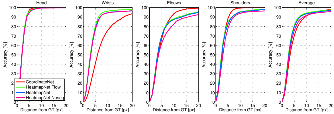
Figure 6.12: Net performance comparison for CoordinateNet , HeatmapNet , HeatmapNet without foreground segmentation ( HeatmapNet Noseg ), and HeatmapNet with optical flow ( HeatmapNet Flow ). For wrists, HeatmapNet with and without foreground segmentations perform equally well (the lines in the graph cover each other). Results are shown for Extended BBC Pose. Plots show accuracy per joint type (average over left and right body parts) as the allowed distance from manual ground truth is increased.
