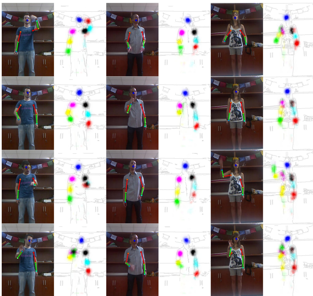
Figure 6.20: Example predictions on ChaLearn (HeatmapNet Flow).
