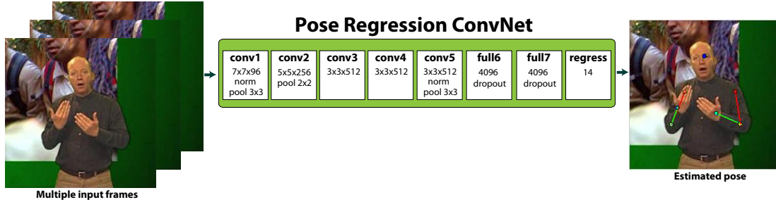
Figure 6.1: Coordinate Network (CoordinateNet) . Given a set of input frames, the convolutional network regresses the positions of the head, shoulder, elbows and wrists.
