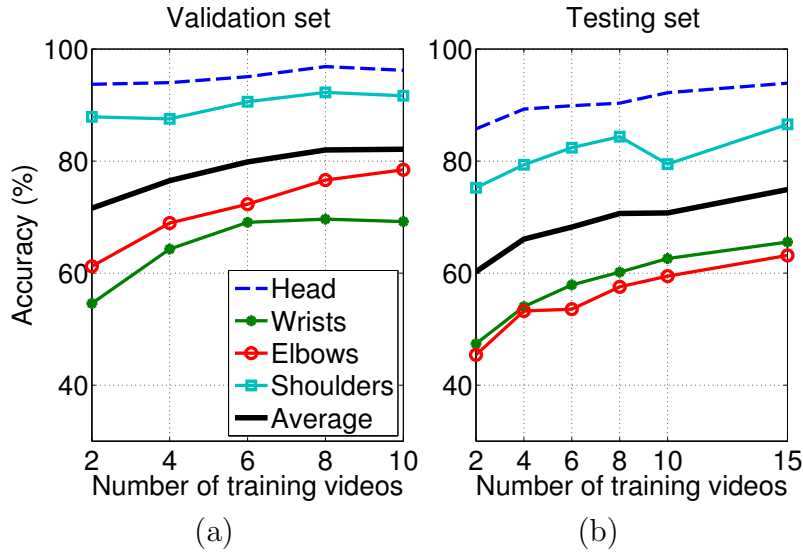
Figure 4.13: Forest performance with increasing amount of training data. Results on validation and testing sets are shown.
