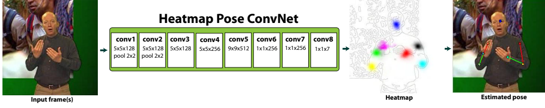
Figure 6.4: Heatmap ConvNet architecture.
