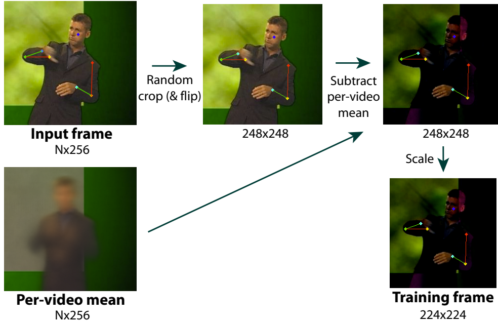
Figure 6.3: Per-video mean and training augmentation. At training time, the training data is augmented with random crops and flips. A per-video mean is computed from a subset of frames to provide some invariance to different background colours. The per-video mean is obtained once per video, and can be computed on-the-fly in online pose estimation scenarios.
