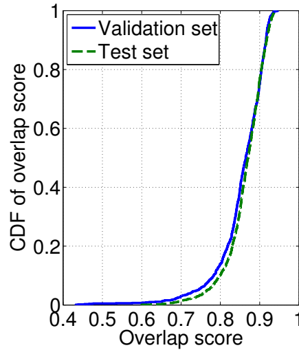
Figure 4.11: Cumulative distribution function of segmentation overlap scores. The majority of scores are in the range 0.85 – 0.95 (high overlap).
