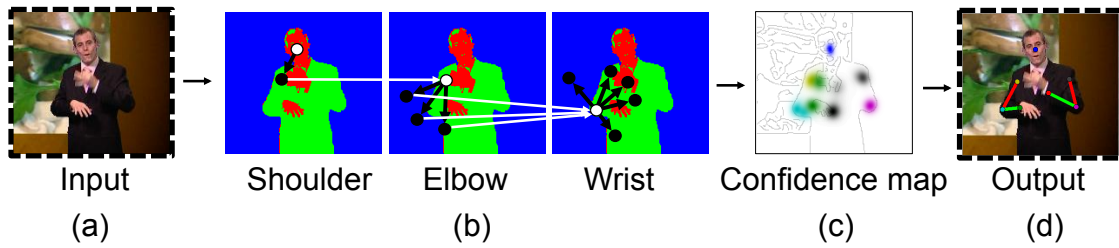
Figure 5.6: Process diagram of sequential upper body pose estimation. (a) Input RGB image. (b) Given the head position, joints are detected using a separate mixture of experts per joint, in order of shoulder, elbow then wrists. Knowledge of previous experts' output joint prediction (white arrows) is passed on when estimating the next joint in sequence. Each expert is responsible for a region of the image relative to the previous joint in sequence. Experts are positioned with fixed learnt offset vectors (positions shown as black dots with black arrows indicating offsets). (c) Joint detections produce a body joint confidence map (different colour per joint) shown superimposed on an edge image, and (d) the points of maximum confidence are selected (final pose output illustrated with a skeleton).
