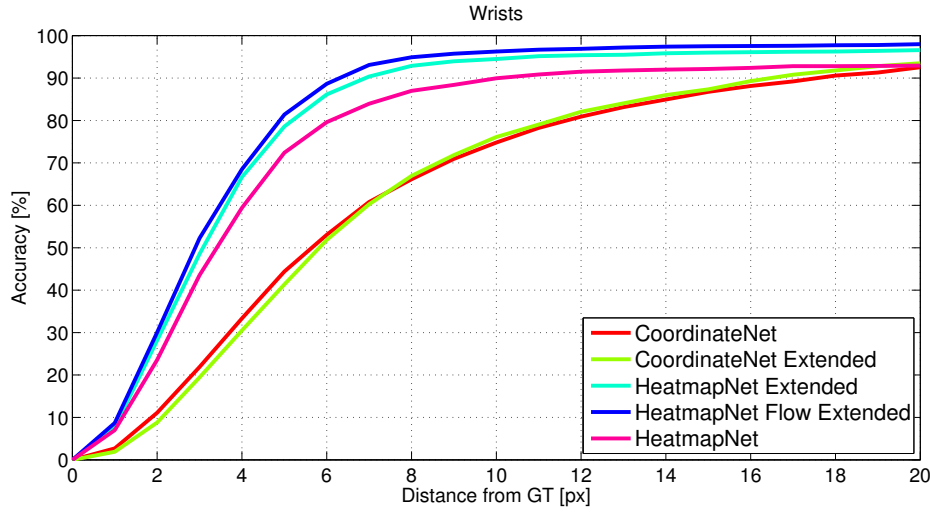
Figure 6.9: Net performance comparison for wrists on (Extended) BBC Pose. CoordinateNet is the network from the previous section; HeatmapNet is the heatmap network; and HeatmapNet Flow is the heatmap network with the parametric pooling layer. ‘Extended’ indicates that the network is trained on Extended BBC Pose instead of BBC Pose. We observe a significant gain going from CoordinateNet to HeatmapNet; for the HeatmapNet from using additional (automatically labelled – see Chapter 3) training data, and a further boost from using optical flow information (and selecting the warping weights with the parametric pooling layer). Plots show accuracy per joint type (average over left and right body parts) as the allowed distance from manual ground truth is increased.
