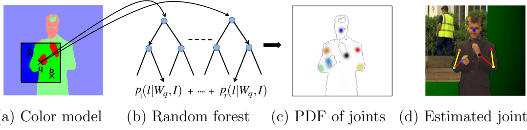
Figure 4.4: Estimating joint positions. (a) input colour model image; (b) random forest classifies each pixel using a sliding window and learnt test functions; (c) probability density function of each joint location, shown in different colours per joint (more intense colour implies higher probability); (d) joint estimates, shown as small circles linked by a skeleton.
