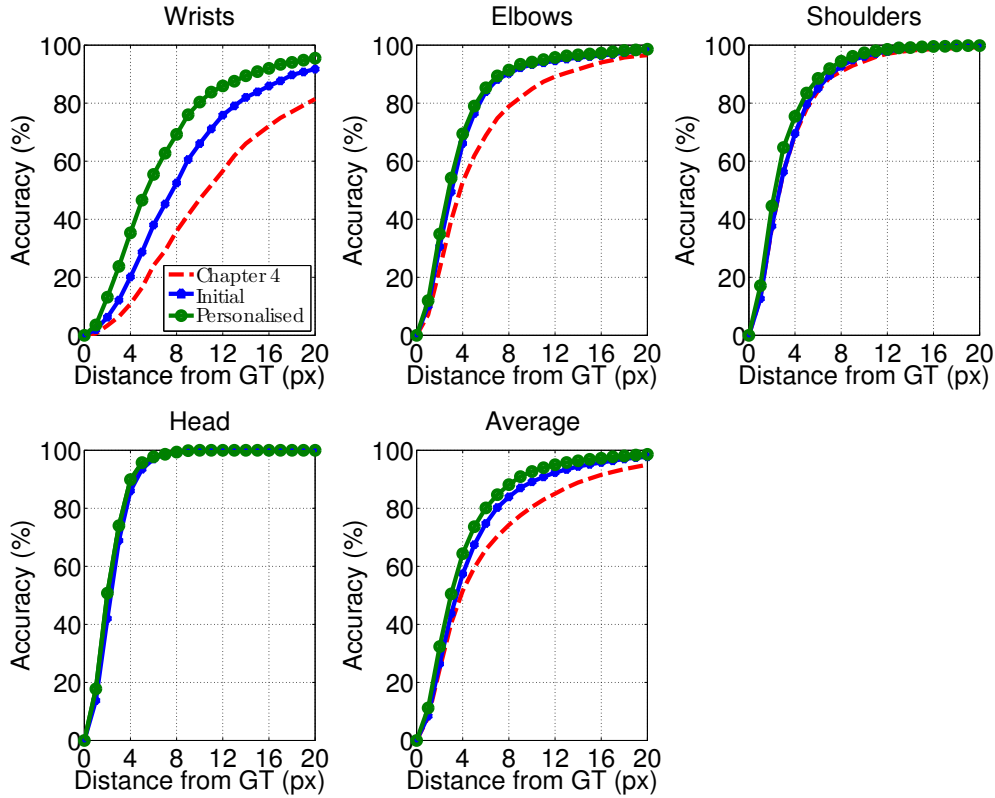
Figure 5.5: Pose estimation performance for short-sleeved test videos , showing a comparison of Chapter 4 (trained on long-sleeved training data) to the initial and personalised short sleeve pose estimator. Per-joint average accuracy against allowed pixel distance from ground truth is shown.
