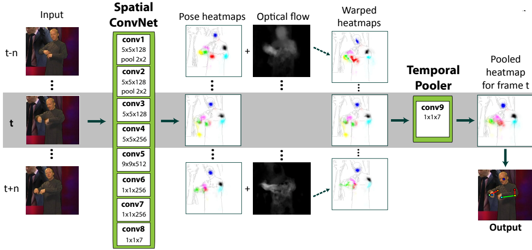
Figure 6.8: Deep expert pooling architecture for pose estimation. The network takes as an input all RGB frames within a n -frame neighbourhood of the current frame t . The fully convolutional Spatial ConvNet (consisting of 8 convolutional layers) predicts a confidence heatmap for each body joint in these frames (shown here with different colour per joint). These heatmaps are then temporally warped to current frame t using optical flow. The warped heatmaps (from multiple frames) are then pooled with another convolutional layer (the temporal pooler), which learns how to weigh the warped heatmaps from nearby frames. The final body joints are selected as the maximum of the pooled heatmap (illustrated here with a skeleton overlaid on top of the person).
