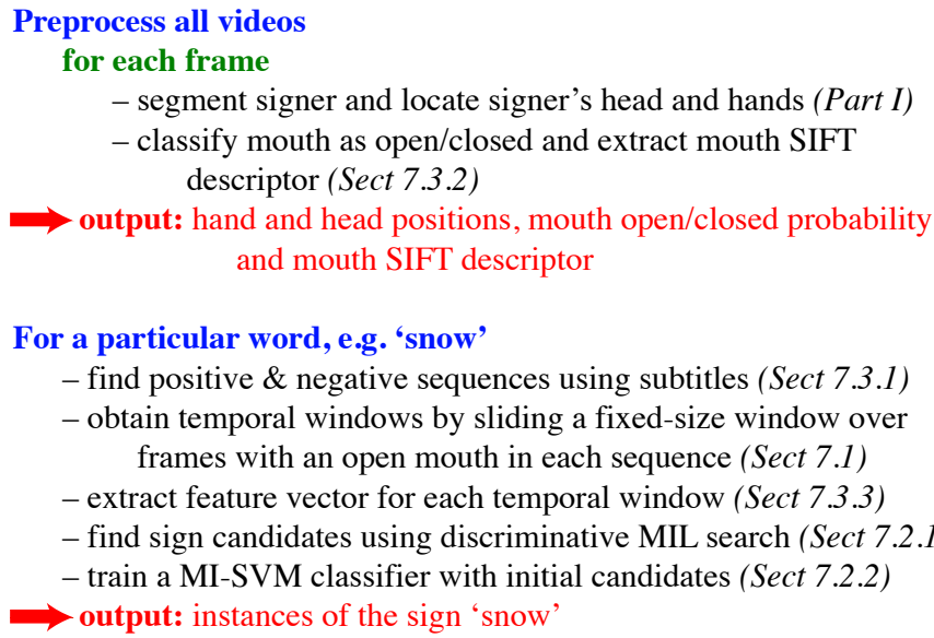
Figure 7.2: Sign Extraction pipeline. The preprocessing of videos (above) and the learning for a given word (below) are shown.
