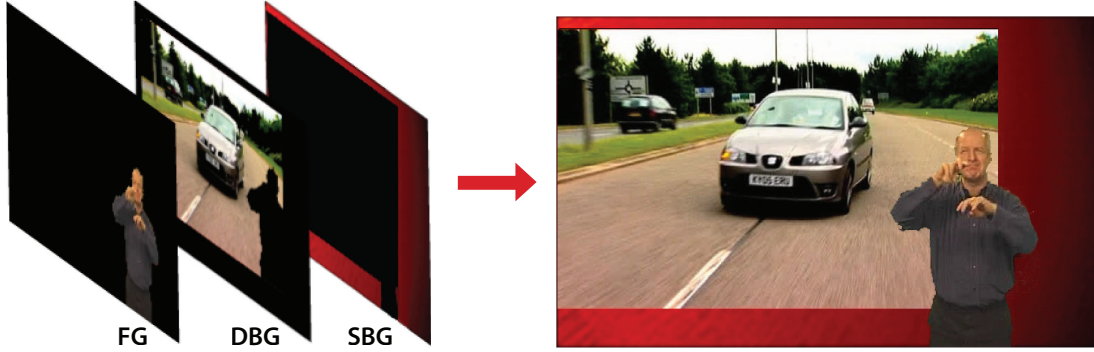
Figure 4.2: Generative layered model of each frame. The co-segmentation algorithm separates the signer from any signed TV broadcast by building a layered model consisting of a foreground (FG), dynamic background (DBG) and static background (SBG).
