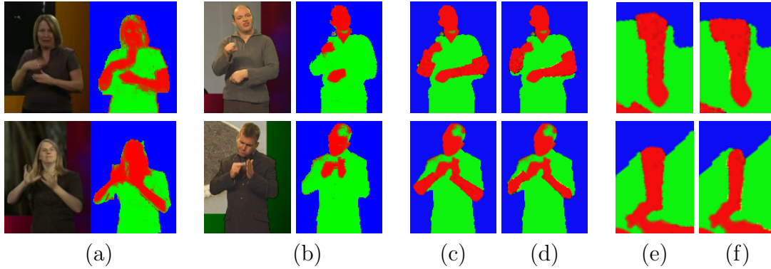
Figure 5.2: Stages in synthesising training data. Rows depict different sleeve length (sleeves in the top row are shorter than in the bottom row). (a) Raw RGB image and CP image counterpart of short -sleeved signers. (b) Example long -sleeved signers and CP images. (c) Synthetically produced CP images of short sleeves using CP images from (b) and of initial arm templates. (d) Personalised synthetic CP images using learnt arm templates. For closer comparison, rotated left arms of the synthetic images in (c) and (d) are shown in (e) and (f) respectively.
