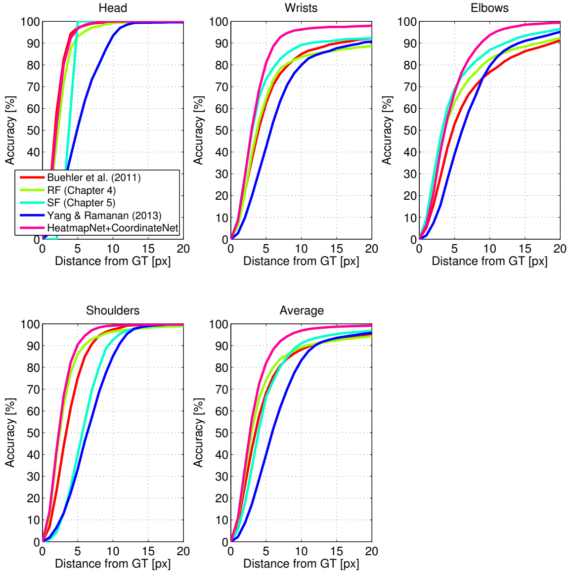
Figure 6.13: Comparison to previous work. We outperform all previous work by a large margin; notice particularly the performance for wrists, where we outperform the best competing method by over 10% at d = 6 . Our method (HeatmapNet+CoordinateNet) uses CoordinateNet Extended for elbows and shoulders, and HeatmapNet Flow Extended for head and wrists. CoordinateNet uses Extended BBC Pose for training; Buehler et al. , RF, SF and Yang & Ramanan use BBC Pose. Plots show accuracy per joint type (average over left and right body parts) as the allowed distance from manual ground truth is increased.
