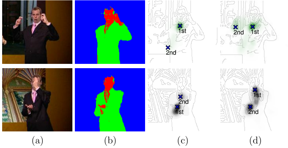
Figure 5.11: The improvement from using optical flow. (a) Example input images and (b) corresponding colour features, with the top row showing an error in segmentation (right arm missed), and bottom row showing a left hand in front of the face. (c) shows sequential forest (SF) confidences (superimposed on an edge image) for the left and right wrists for the two rows, with the first two modes of confidence (shown as crosses) both in wrong wrist locations. (d) demonstrates improved confidence output from using optical flow: in the top row the 2nd best mode of confidence now correctly locates the right wrist, and in the bottom row the 1st mode of confidence locates the left wrist.
