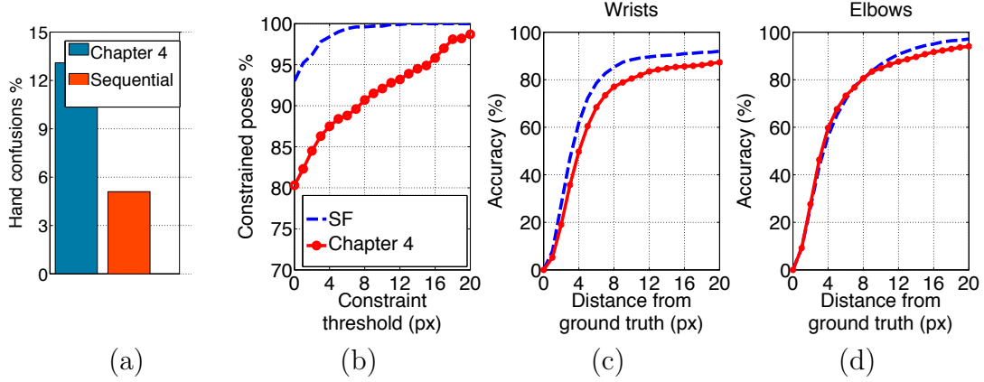
Figure 5.7: Sequential forest performance on the BBC TV dataset. (a) Bar chart showing percentage of hand confusions (lower is better); (b) number of constrained (near-correct) poses across all values of the constraint threshold (higher is better); (c) & (d) accuracy of average wrist and elbows joints respectively (averaged of left and right arms) against allowed pixel distance from ground truth (higher is better) (at 5 pixels).
