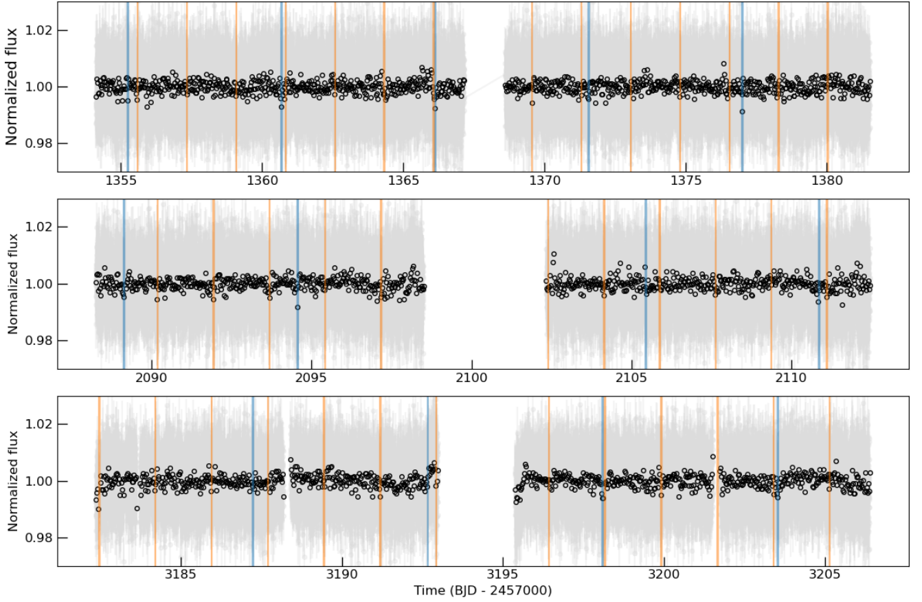
Figure 1. TESS 2-min cadence photometry of TOI-237 obtained with the TESS automatic aperture. Each of the panels shows the Sectors 2, 29, and 69, respectively. The gray points correspond to each measurement, and the black circles are binned by 36 minutes. TOI-237 b is highlighted in blue, and TOI-237 c (TIC 305048087.02) in orange.
