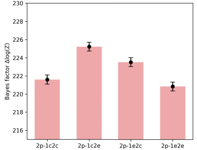
Figure 6. Bar plot representing the Bayes factor of the tested models for the TOI-4336 A system. The null hypothesis is taken as a one-planet circular fit, the other models are two-planet fits: two circular orbits, planet b circular and planet c eccentric, the inverse, and two eccentric orbits.
