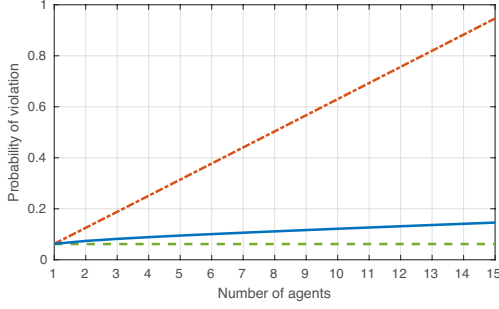
Fig. 2. Comparison of the bounds on the violation probability as functions of the number m of agents, when \beta = 10^{-5} , N_i = \bar{N} = 4500 , \beta_i = \beta/m , i = 1, \dots, m , and d = 50 . Dashed green line: \bar{\varepsilon} in Theorem 1; dotted-dashed red line: \tilde{\varepsilon} in Proposition 1; solid blue line: \varepsilon in Theorem 2. The dotted-dash red line has an approximately constant growth rate ( \tilde{\varepsilon} \approx m\bar{\varepsilon} ), and the solid blue line shows that \varepsilon is moderately increasing with m , while allowing for the information on the scenarios to be distributed.
