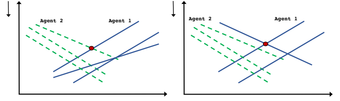
Fig. 1. Graphical illustration of the support set for a problem with two agents. The problem involves two decision variables, where we seek to minimize one of the two (downwards pointing arrow denotes the optimization direction). Agents have the same number of scenarios, and scenarios give rise to different type of constraints, i.e., solid and dashed line constraints for agent 1 and agent 2, respectively. Two instances corresponding to different scenario extractions are denoted: (left panel). d_{1,N} = 1 and d_{2,N} = 1 ; (right panel). d_{1,N} = 2 and d_{2,N} = 0 .
