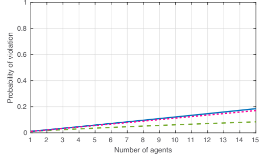
Fig. 3. Comparison of the bounds on the violation probability as functions of the number m of agents for the case of local decision vectors, when \beta = 10^{-5} , \beta_i = \beta/m , n_i = 5 , N_i = \bar{N} = 4500 , i = 1, \dots, m , and d = n = n_i m . The dashed green line representing the violation probability \bar{\varepsilon} in Theorem 1 grows with m because of the dependence of d on m . The dotted magenta and blue solid lines representing respectively the violation probability \varepsilon in Theorems 3 and 2 grow at a higher rate.
