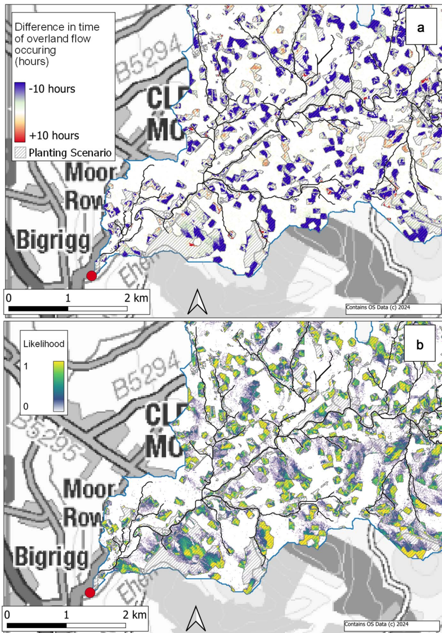
Figure 5. (a) Comparison of difference in overland flow for the 40% random tree planting scenario at the catchment outlet of the Ennerdale catchment, where decreased length of time of runoff is represented by the blue areas and increased length of time by the red areas. (b) Likelihood map for the same scenario where cells that have decreased overland flow observation time in all cells are given values of 1 (yellow regions) and cells that have no change are given values of 0 (white regions). The black line represents the water course, and the red dot is the catchment outlet.
