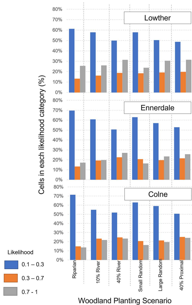
Figure 6. Comparison of likelihood values for each tree planting scenario and for each catchment (Lowther top, Ennerdale middle, Colne bottom).
