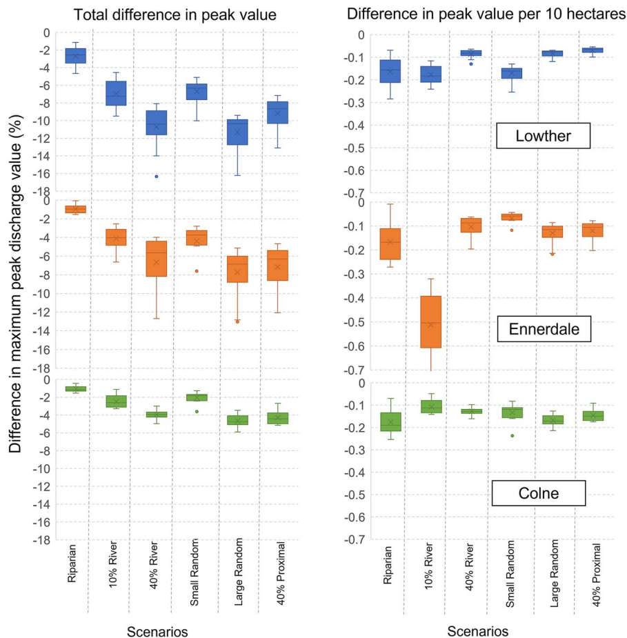
Figure 4. Box plot comparison of the difference in peak as a percentage for each planting scenario (left hand side), and the difference in peak per 10 hectares of planting (right hand side) for Lowther (top), Ennerdale (middle), Colne (bottom).
