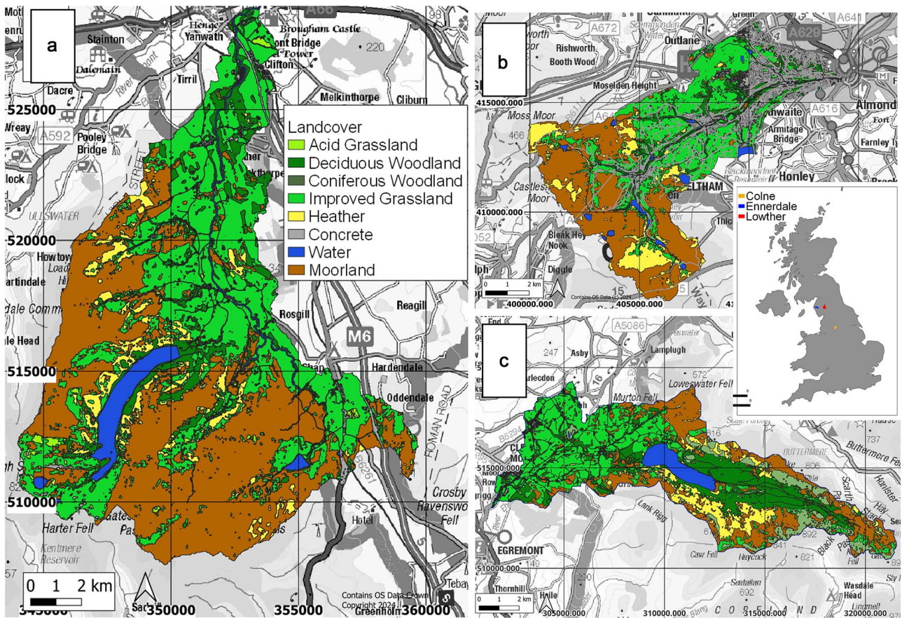
Figure 1. Location and existing landcover of the three catchments, Lowther (a), Colne (b), and Ennerdale (c), with location in the UK (inset) and with EPSG 27700 coordinates. Land cover classes are determined from UK CEH LandCover 2022 data, and based on the processing of sentinel 2 data described in section 3.1.
