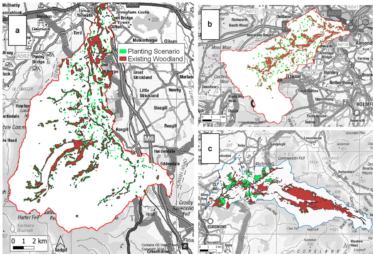
Figure 8. Combined best polygon planting scheme layout (green area) for Lowther (a), Colne (b), and Ennerdale (c).
