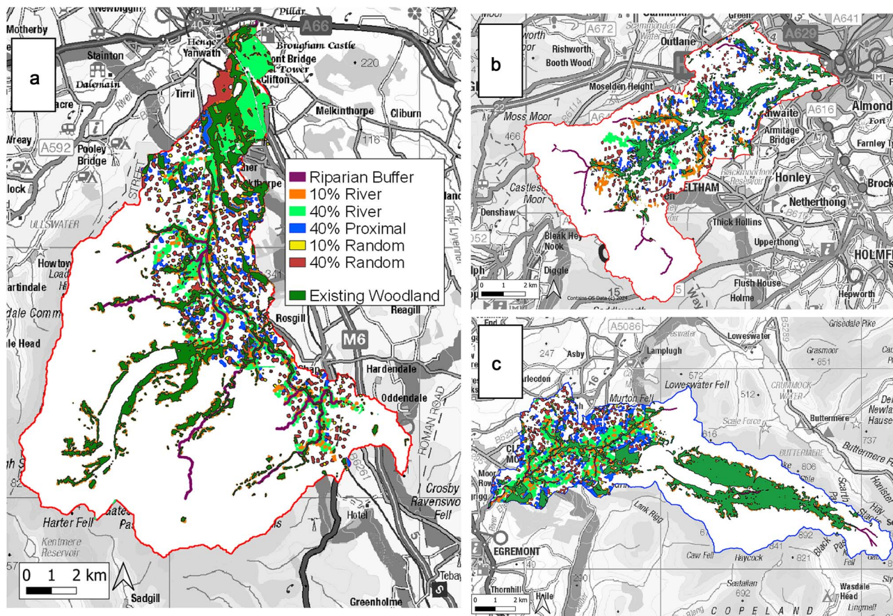
Figure 3. Woodland planting scenarios for the three catchments: Lowther (a), Colne (b), and Ennerdale (c).
