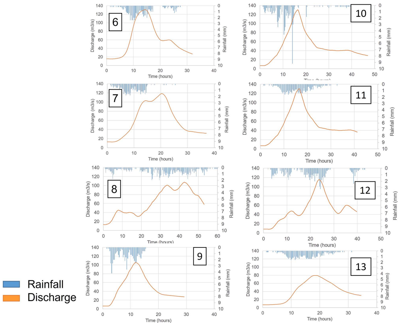
Figure 2. Storm event hydrographs for the Lowther catchment with each event from Table 2 numbered for each hydrograph.
