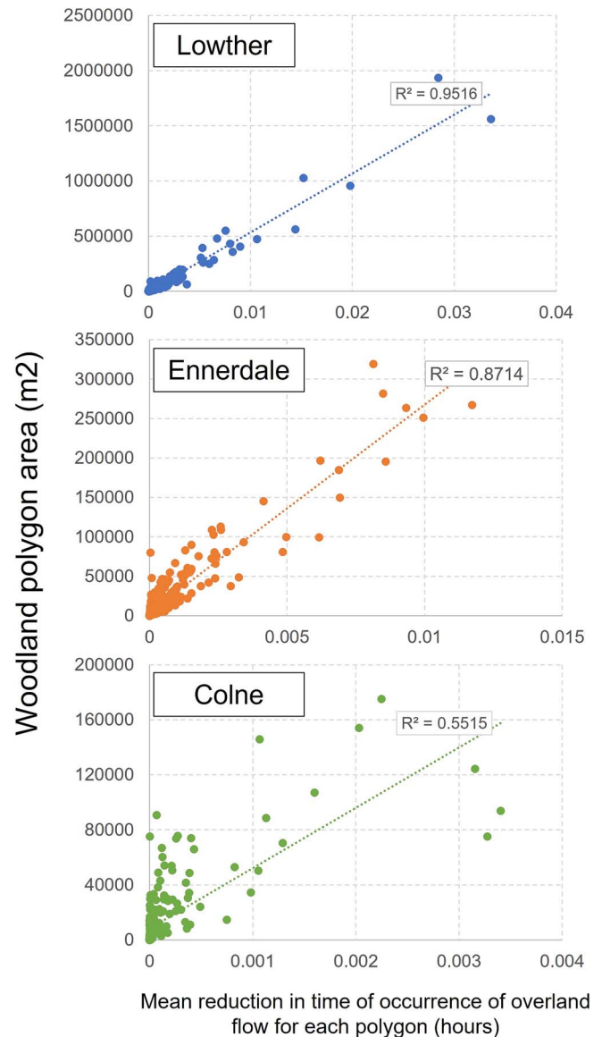
Figure 7. Regression plots for catchment characteristics against difference in time values for each polygon for the 40% random sampling tree scenario for each catchment.
