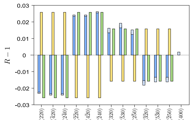
FIG. 5: (Color online) Bar chart of the observed flipping ratios ( R-1 ) shown in the first bar [blue, lighter area represents (R-1) \pm \sigma ] compared to the calculated values for a left-handed structure (second bar [yellow]) and a right-handed structure (third bar [green]).
