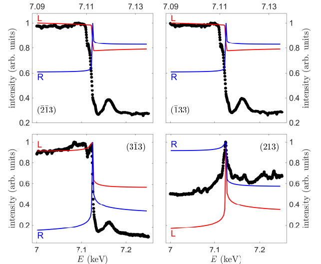
FIG. 9: (Colour online) The behavior of four non-coplanar reflections show large contrast in the simulations for the left-handed [(red) lines] and right-handed [(blue) lines] enantiomers. The black circles represent the renormalized experimental intensity of the four reflections measured in the center of our specimen at room temperature. As immediately evident only the simulations with the left-handed structure match the trend of the experimental data. No attempt was made to simulate the subtle feature shown by the experimental data across the transition.
