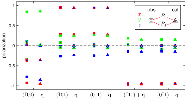
FIG. 8: (Color online) Observed (squares) and calculated (triangles) polarization values P_{if} for incident neutrons polarized along P_i (marker face color) and polarization analysis along P_f (marker edge color) for the three different directions x (red), y (green) and z (blue).
