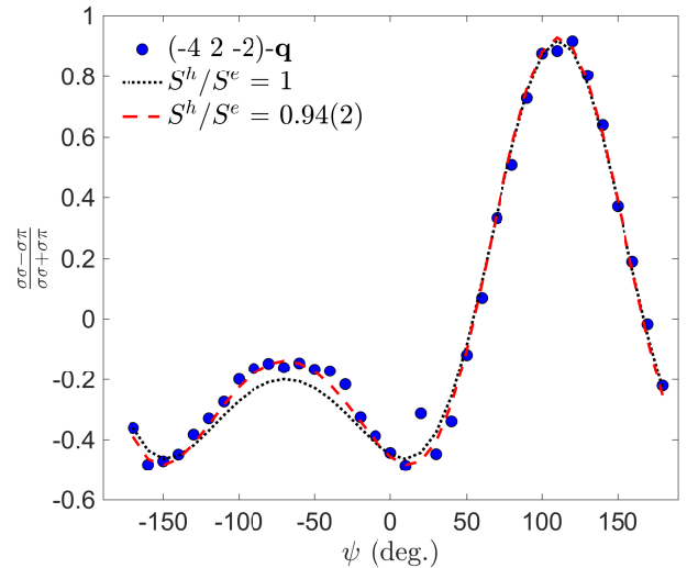
FIG. 11: (Colour online) Azimuthal scan with incident polarization perpendicular to the scattering plane in non-resonant condition on the (-4\ 2\ -2)\text{-}\mathbf{q} reflection. The ellipticity is given by the ratio of the spin component along the hard axis ( S^h ) and the easy axis ( S^e ) of the envelope.
