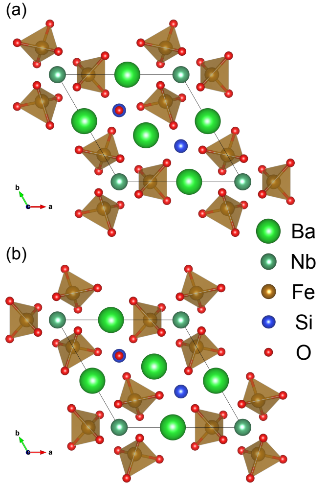
FIG. 1: (Color online) Left-handed (a) and right-handed (b) crystal structure of \text{Ba}_3\text{NbFe}_3\text{Si}_2\text{O}_{14} . The atomic positions of the left-handed structure [e.g. Fe atom at (0.249\ 0\ 0.5) ] are taken from Ref. 11 and have been inverted for the right-handed structure.
