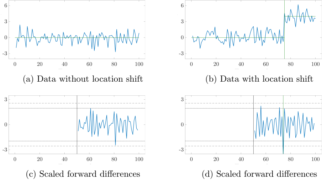
Figure 1: Illustration of the stylized Step-Indicator Saturation algorithm
