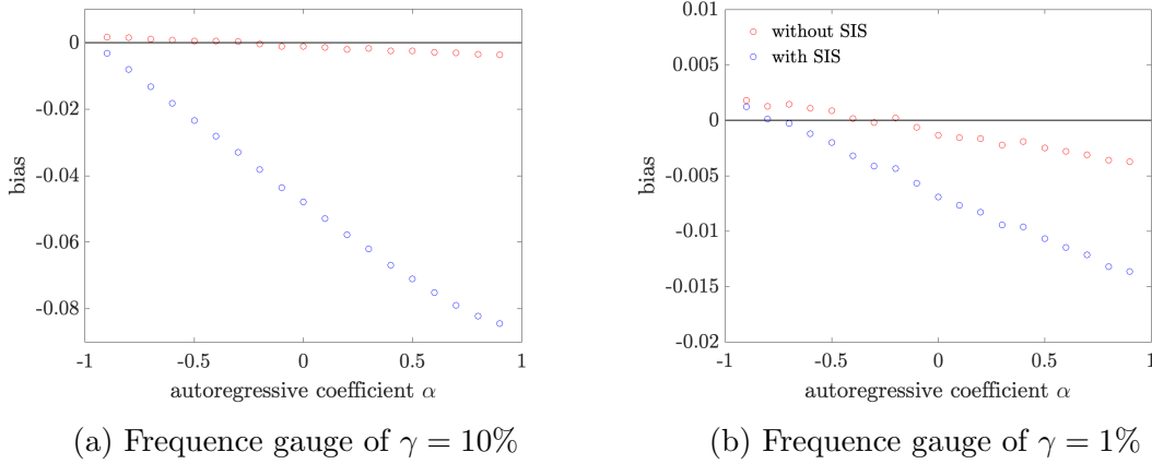
Figure 5: Bias of updated regression estimator as function of autoregressive coefficient
