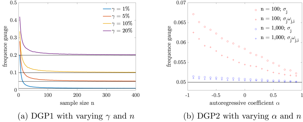
Figure 2: Finite sample properties of the frequency gauge
