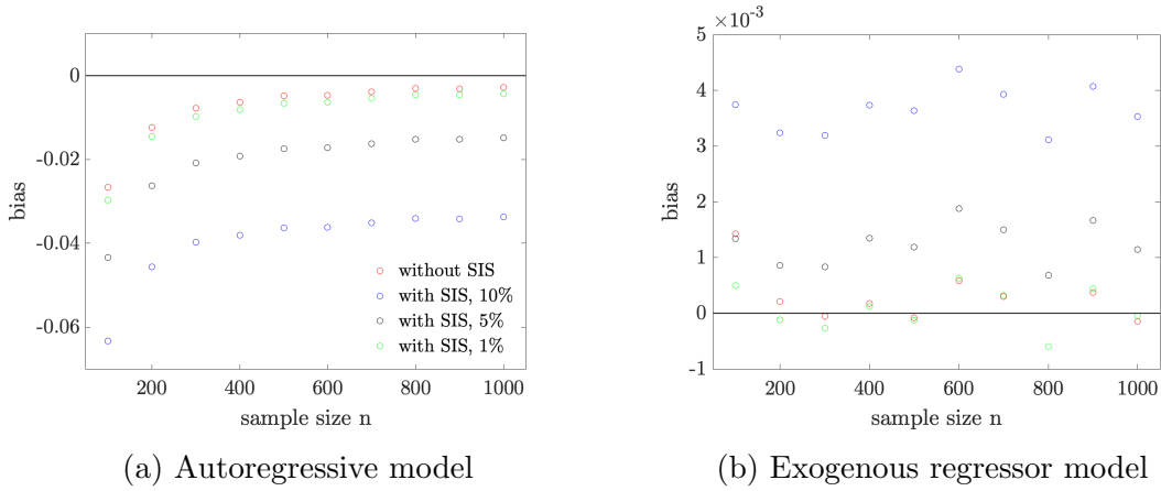
Figure 4: Bias of updated regression estimator as function of sample size
