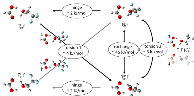
Fig. 7 Chirality-focused overview on the isomerisation options of the T_gF complex at B3LYP-D3(BJ)/def2TZVP level (ZPE corrected). Facile hinge motion conserves the T_g chirality, whereas T_{g+} \leftrightarrow T_{g-} inversion can be achieved by alcohol torsion through a transition state with mirror plane or through an asymmetric transition state following hinge motion, and also by concerted double proton transfer through an exchange barrier above the OH stretching fundamental excitation.
