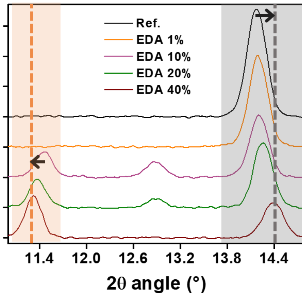
Figure S17: Zoom on 2\theta angles 11.2^\circ to 14.6^\circ . 2H(100) / 4H(100) peaks are highlighted in orange and cubic(100) in grey. Arrows indicate a shift of the 2H/4H(100) and cubic(100) phase with increasing EDA. Reduction of the peak at \sim 12.9^\circ from the 4H polytype confirms the phase mixture in the film shifting to entirely 2H polytype at the highest EDA concentration.
