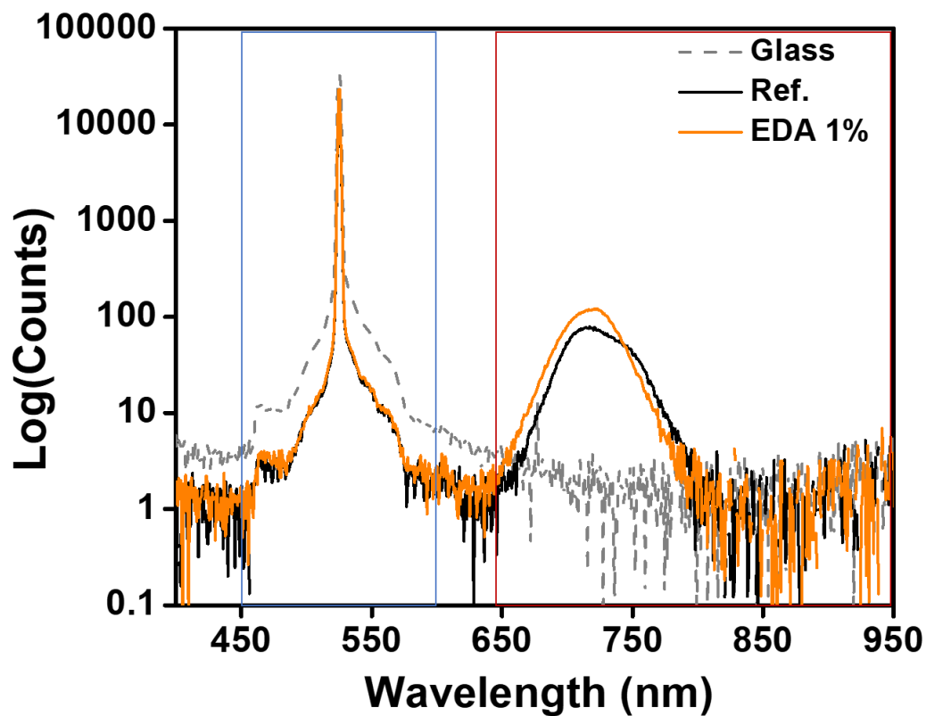
Figure S1: PL spectra from integrating sphere coupled with a 532 nm laser at 60 mA/cm 2 . Blue lines show the excitation region and the red lines the emission region. The dashed grey spectrum is the one of a bare glass film used as blank.
