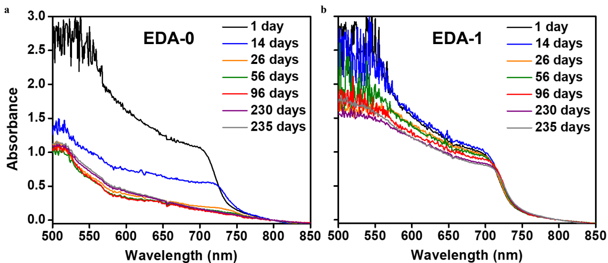
Figure S2: UV-Vis of EDA-0., EDA-1 over 235 days of aging. The absorbance was corrected for scattering by subtracting the background signal from 850 to 1200 nm. Samples were stored unencapsulated in the dark at an average room temperature of 19.5 °C and 31% RH.
