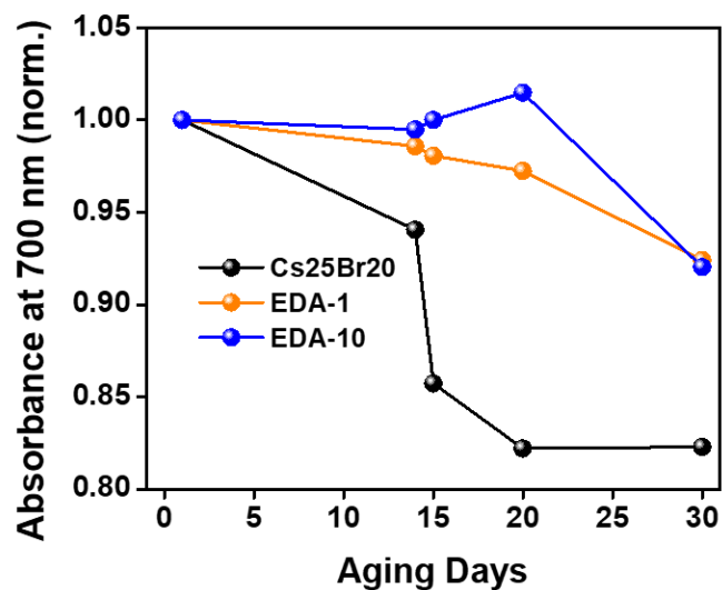
Figure S25: Absorbance at 700 nm from UV-Vis of FA_{0.83}Cs_{0.25}Pb(I_{0.80}Br_{0.20})_3 (black) with addition of 1 mol% (orange) and 10 mol% (blue) of EDA over 30 days of aging recorded on day 1, 14, 15, 20 and 30 of aging. The values are normalized to day 1. Samples were stored unencapsulated in the dark at an average room temperature of 19.5 °C and 31% RH
