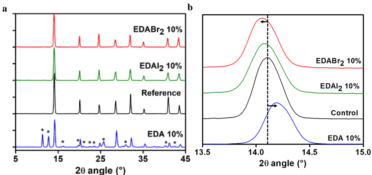
Figure S32: (a) XRD patterns of the reference film (black), after addition of 10 mol% of \text{EDA}\text{H}_2\text{Br}_2 (red), \text{EDA}\text{H}_2\text{I}_2 (green) and EDA (blue). Peaks denoted with * correspond to the 4H polytype phase. (b) Highlight on the region from 13.5^\circ to 15^\circ of the patterns shown in (a). The dashed line follows the signal of the (100) plane of the cubic phase of the control and the arrows indicates the shift to smaller angles in the case of \text{EDA}\text{I}_2 and \text{EDABr}_2 addition and larger angles with EDA.
