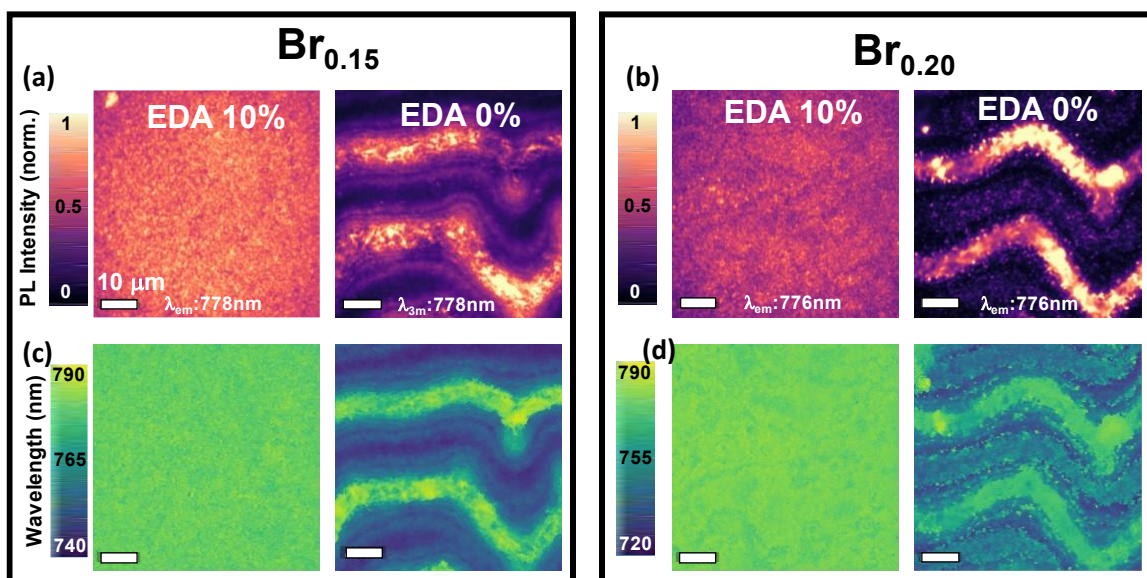
Figure S26: (a) Hyperspectral PL intensity map of FA_{0.83}Cs_{0.17}Pb(I_{0.85}Br_{0.15})_3 indicated as “Br 0.15 ” and (b) FA_{0.83}Cs_{0.17}Pb(I_{0.80}Br_{0.20})_3 indicated as “Br 0.20 ” with (EDA 10%) and without (EDA 0%) addition EDA. PL images are shown at the emission wavelength ( \lambda_{em} ) indicated at the bottom of the figures. Excitation was achieved with a white lamp with short pass filter at 500 nm. The emission was recorded using a 500 nm dichroic and 650 nm long pass filter. (c) Peak emission wavelength map of the Br 0.15 and (d) Br 0.20 with (EDA 10%) and without (EDA 0%) addition EDA.
