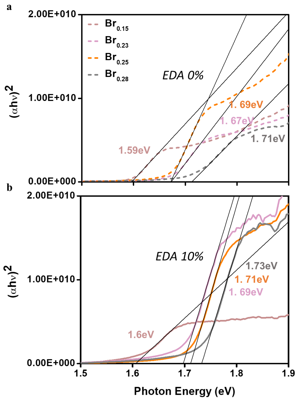
Figure S23: (a) Tauc plots of the EDA-0 and (b) EDA-10 \text{FA}_{0.83}\text{Cs}_{0.17}\text{Pb}(\text{I}_{1-x}\text{Br}_x)_3 with x=0.15 ( \text{Br}_{0.15} , brown), 0.23 ( \text{Br}_{0.23} , pink), 0.25 ( \text{Br}_{0.25} , orange), 0.28 ( \text{Br}_{0.28} , grey)
