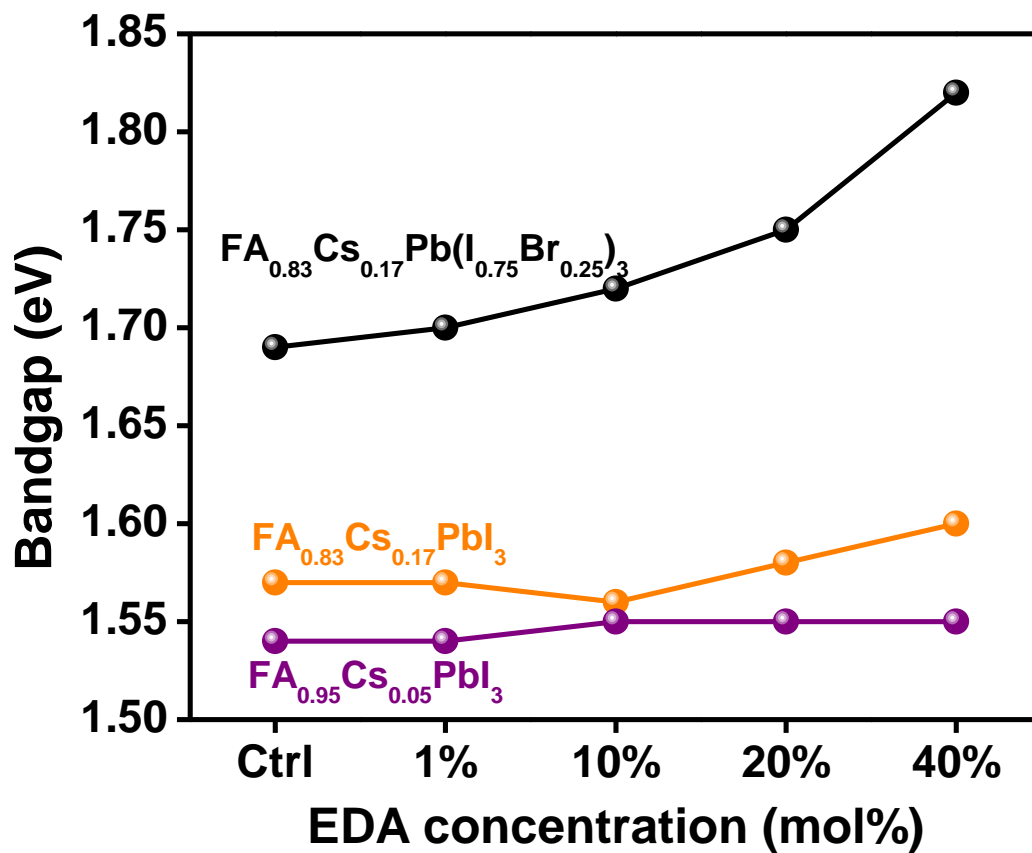
Figure S22: Bandgap extracted from Tauc plot shown in Figure S17 (black), Figure S20a (orange) and Figure S20b (purple) as a function of amount of EDA added in the precursor solution in mol%.
