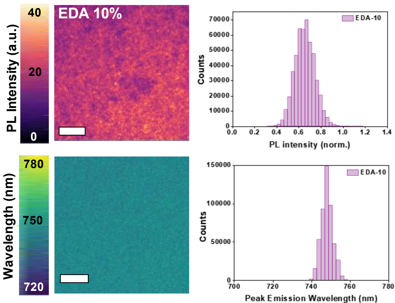
Figure S11: (a) Hyperspectral PL intensity map of the EDA-10 sample. Excitation was achieved with a white lamp with short pass filter at 500 nm. The emission was recorded using a 500 nm dichroic and 650 nm long pass filter. (b) Histogram of the PL intensity distribution at the maximum emission wavelength. (c) Peak emission wavelength map. (d) Histogram of the distribution of peak emission wavelengths.
