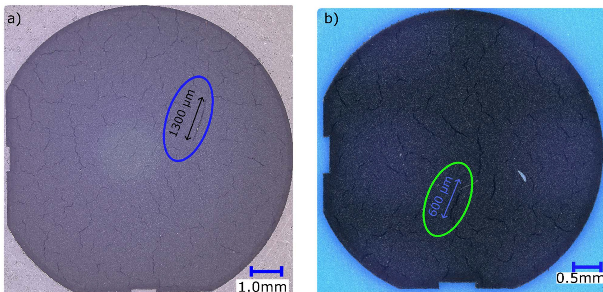
Fig. 1 Micrographs of the cathode used for operando measurements discussed here (a) and the electrode referred to in the SI (b). The crack that was studied in this work is circled with the length noted. The crack is comparable to those seen previously and imaged by X-ray computed tomography. 35,58
