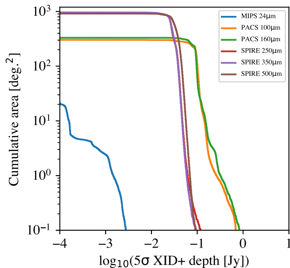
Figure 9. Cumulative area to a given depth or deeper for the XID+ forced photometry for far-infrared fluxes in the MIPS 24, PACS Green, Red, SPIRE 250, 350, and 500 bands.
