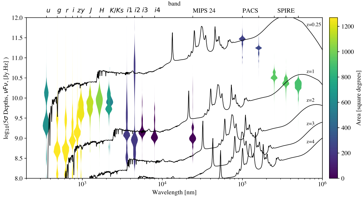
Figure 10. The distribution of area on the sky to a given depth, vFv , shown via a violin plot, for each broad-band type (taking the deepest specific band available in a given HEALPIX cell). Optical and NIR depths are 5\sigma depths in a 2 arcsec aperture. MIPS, PACS, and SPIRE depths are 5\sigma depths for the XID+ forced photometry values. The colour of each area is determined by the total area that data for that band is available. We also plot a HELP spectral energy distribution for a ULIRG galaxy with star formation rate of 200 M_{\odot} \text{ yr}^{-1} and a stellar mass of 10^{10} M_{\odot} at various redshifts.
