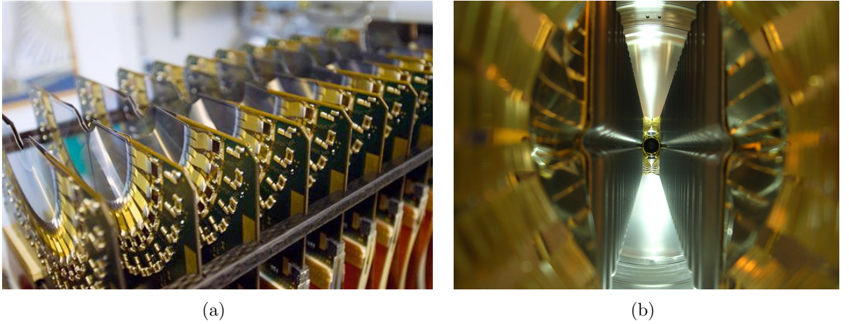
Figure 2.16: a) VELO modules. b) Interior of the RF foil, viewed in the open position.
