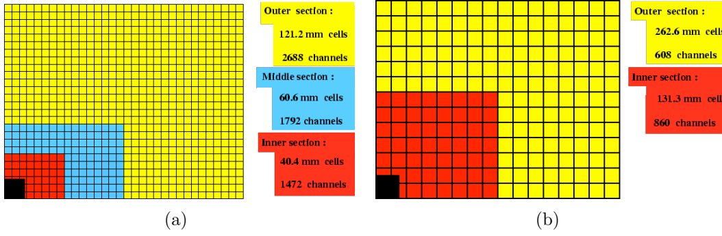
Figure 2.13: Calorimeter cell arrangement. One quarter of the face is shown. a) ECAL. b) HCAL.
