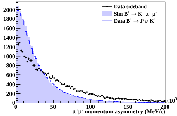
Figure 4.6: The muon momentum asymmetry, defined as |p_{\mu^+} - p_{\mu^-}| , shown for B^\pm \rightarrow K^\pm \mu^+ \mu^- simulation, B^\pm \rightarrow J/\psi K^\pm data and data sideband. In true dimuon decays, the two muons are more likely to have a similar momentum than if the muons come from combinatorial background.
