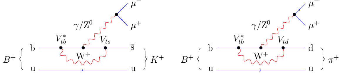
Figure 1.12: B^\pm \rightarrow h^\pm \mu^+ \mu^- decays where h = K (left) and h = \pi (right). The two decays vary in the CKM matrix element at the end of the W^\pm loop.
