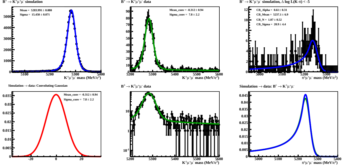
Figure 4.14: Determination of the convolution function necessary to correct simulation for data-simulation differences. Top left: K^\pm \mu^+ \mu^- mass peak fitted in simulation. Top centre: K^\pm \mu^+ \mu^- mass peak fitted in data, including a background function (seen on log scale, bottom centre). Bottom left: the convolution function necessary to translate from simulation to data. Top right: peaking background shape in simulation, fitted with a Crystal Ball. Bottom right: peaking background shape (blue) and when corrected for simulation-data differences (green).
