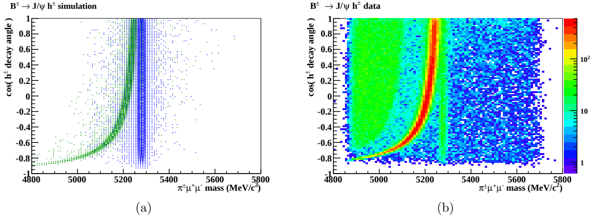
Figure 3.5: Decay angle of the hadron vs. the reconstructed \pi^\pm\mu^+\mu^- mass for: a) selected events from B^\pm \rightarrow J/\psi K^\pm (green) and B^\pm \rightarrow J/\psi \pi^\pm (blue) simulation. b) Selected events from data reconstructed as B^\pm \rightarrow J/\psi \pi^\pm . The green vertical band is the J/\psi \pi^\pm component. The red (high statistics) curving band is J/\psi K^\pm decays. The green region in the top left hand corner is partially reconstructed background.
