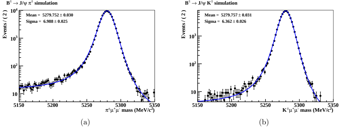
Figure 3.7: Selected signal events from simulation samples. a) B^\pm \rightarrow J/\psi \pi^\pm decays. b) B^\pm \rightarrow J/\psi K^\pm decays. The distributions are fitted with a modified Gaussian lineshape, see Equation 3.4.
