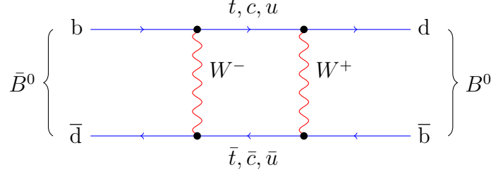
Figure 1.5: B^0 meson mixing. Properties of the top quark running in the loop may be inferred from the oscillation frequency.
