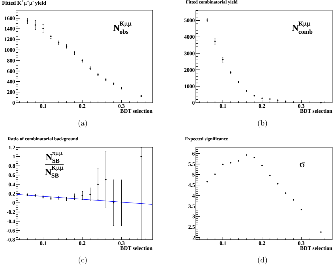
Figure 4.8: Choice of working point by maximising Equation 4.5. a) Fitted B^\pm \rightarrow K^\pm \mu^+ \mu^- signal yield. b) fitted combinatorial yield, measured from data as a function of BDT cut. c) Expected ratio of background events, measured from the sideband and fitted to avoid statistical fluctuations. d) Expected significance as a function of BDT cut.
