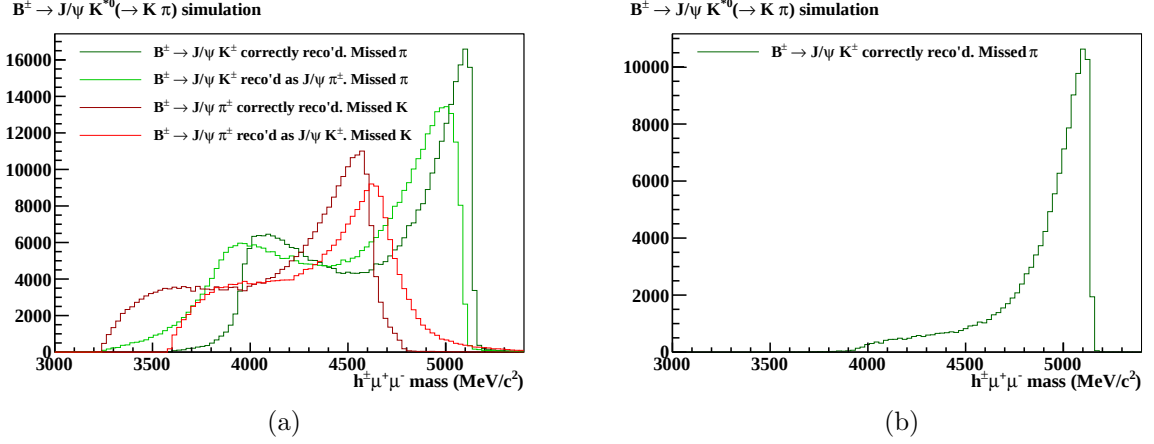
Figure 3.10: Various reconstructions of B^0 \rightarrow J/\psi K^{*0}(\rightarrow K\pi) simulation, see text for details. a) All simulated events. b) Simulated events which pass the selection. This is the only partially reconstructed background shape considered for B decays.
