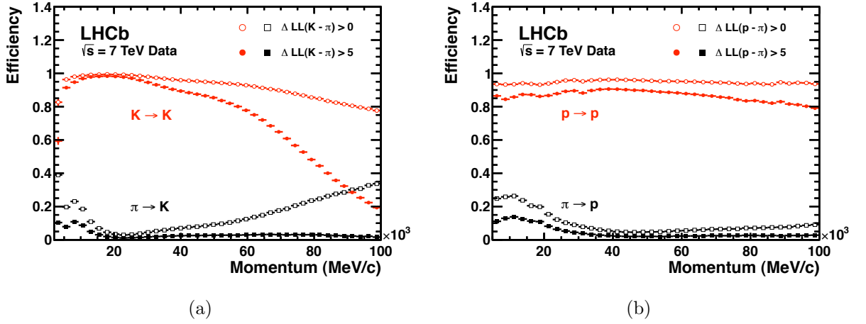
Figure 2.22: Kaon (a) and proton (b) identification efficiency, as a function of momentum. Two different \Delta \log \mathcal{L} requirements are shown, loose (open markers) and tight (closed markers). The pion misidentification rate is also shown.
