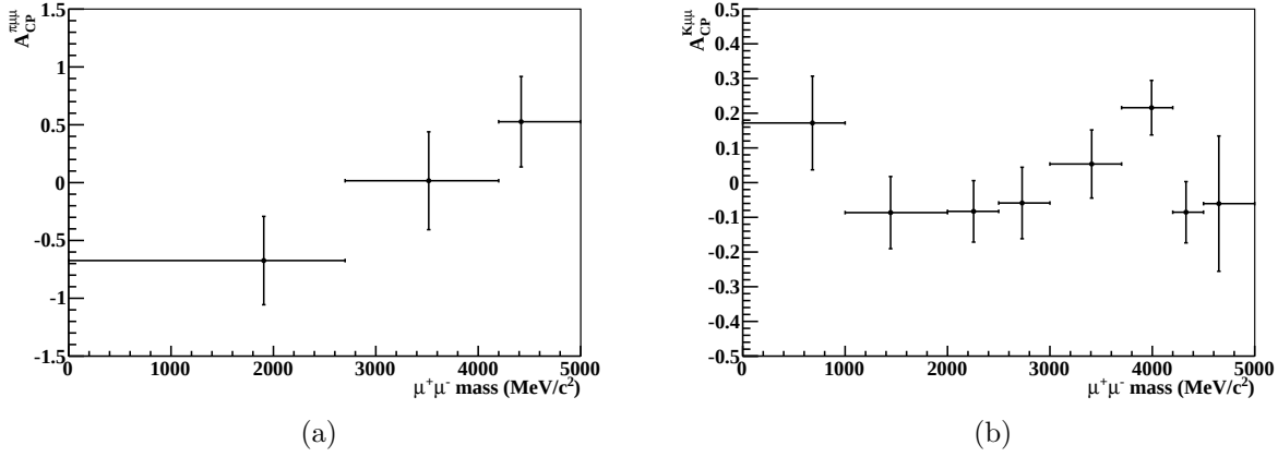
Figure 4.22: CP asymmetries of B^\pm \rightarrow \pi^\pm \mu^+ \mu^- decays (a) and B^\pm \rightarrow K^\pm \mu^+ \mu^- decays (b) in bins of dimuon mass. Bins were chosen to have roughly equal number of events. Horizontal error bars show the bin widths, the results are plotted at the barycentre of each bin. The uncertainties on the asymmetries are statistical only, and are taken from the fit.
