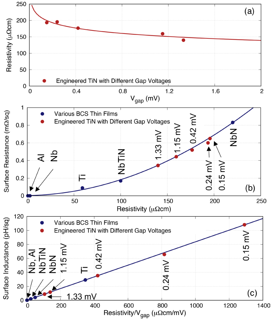
Figure 6. (a) Plot showing the resistivity of various engineered TiN film with different gap voltages, where V_{\text{gap}} is the gap voltage. (b) Relation between surface resistance and resistivity at 0.02 f_{\text{gap}} for various BCS (Bardeen-Cooper-Schrieffer) thin films under study, along with the engineered TiN films, all at 50nm thickness. & (c) Similar to (b) for the relation between surface inductance and the ratio of \rho_N/V_{\text{gap}} . The various engineered TiN films are labelled with their corresponding V_{\text{gap}} . Ti, Titanium; NbTiN, Niobium Titanium Nitride; NbN, Niobium Nitride; Al, Aluminium; Nb, Niobium; TiN, Titanium Nitride.
