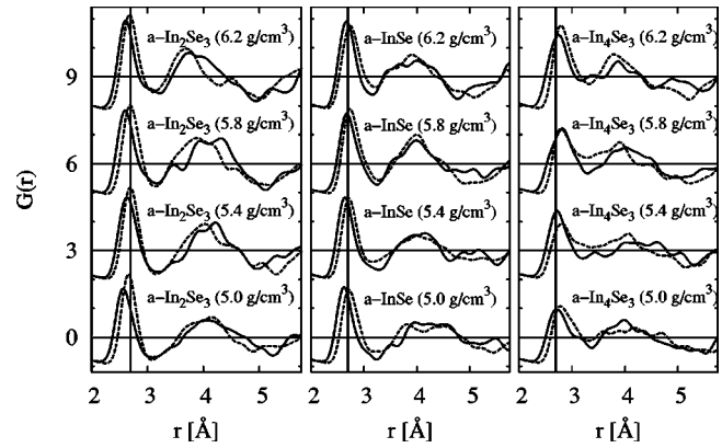
FIG. 2. Reduced radial distribution functions for different a\text{-In}_x\text{Se}_y structures with different densities. Solid and dashed lines predicted by DNP and SN basis set simulations, respectively. Vertical lines at r=2.7 \text{ Å} serve as a guide for the eyes.
