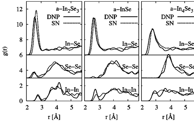
FIG. 3. Partial pair correlation functions in (a) a\text{-In}_2\text{Se}_3 ( \rho=5.0 \text{ g/cm}^3 ), (b) a\text{-InSe} ( \rho=5.4 \text{ g/cm}^3 ), and (c) a\text{-In}_4\text{Se}_3 ( \rho=5.8 \text{ g/cm}^3 ), for simulations performed by DNP (solid line) and SN basis sets (dashed line).
