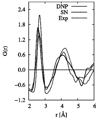
FIG. 1. Reduced radial distribution function of a\text{-In}_2\text{Se}_3 ( \rho=5.0 \text{ g/cm}^3 ). Solid and dashed lines show data for structures predicted by DNP and SN basis set simulations, respectively. Dotted line shows measurement from Ref. 13.
