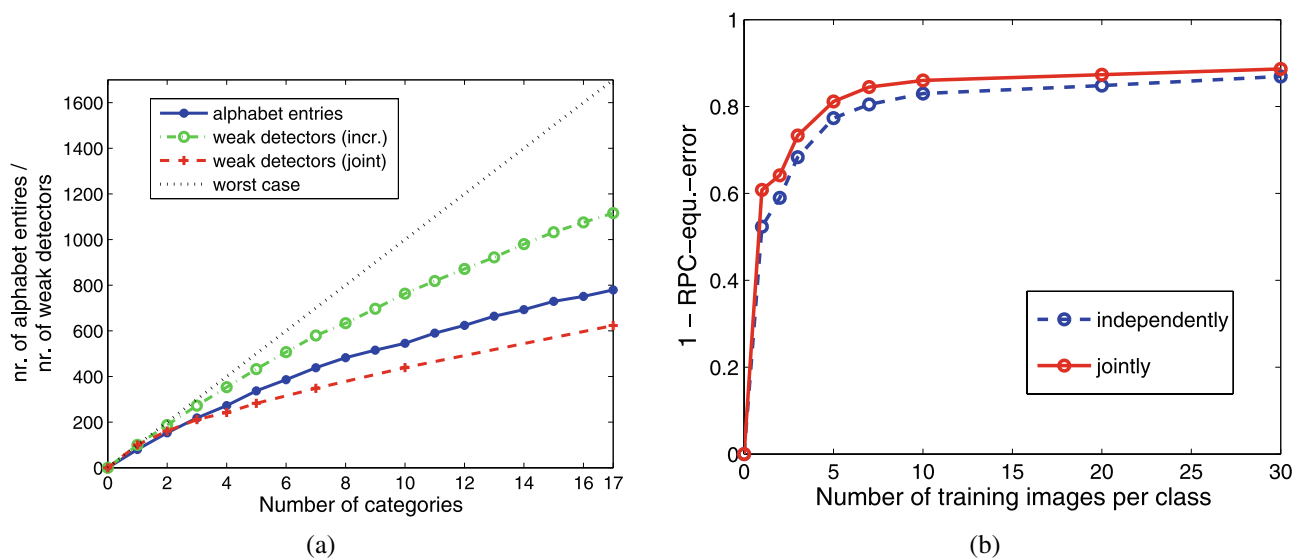
Fig. 29 (a) The increase in the number of alphabet entries w.r.t. the number of classes, and increase of the number of weak detectors when adding new classes incrementally or training a set of classes jointly. The values are compared to the worst case (linear growth, dotted line). For weak detectors the worst case is training independent and given by (\sum_{i=1}^C T_{c_i}) , and for the alphabet we approximate the worst case by
