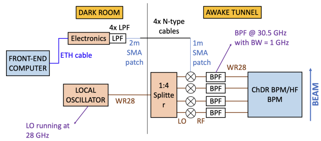
Figure 3: Schematic of the signal processing chain of the high-frequency BPMs at AWAKE.
