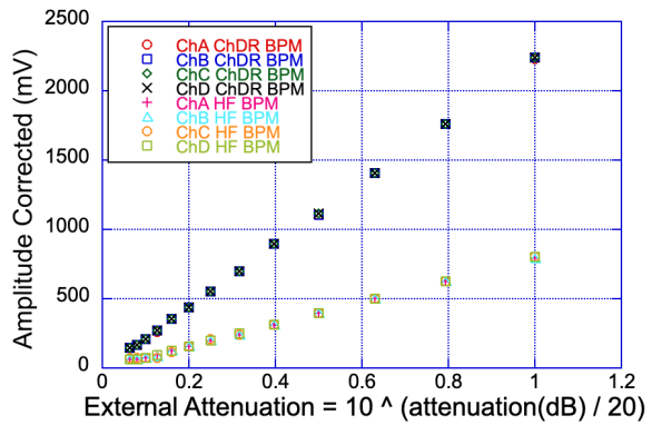
Figure 7: Averaged ADC amplitudes (corrected) as a function of the external variable attenuator setting.
