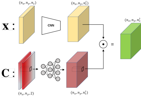
Figure 2: CoordGate. The data, \mathbf{X} , and coordinates, \mathbf{C} , are fed through a CNN and a MLP respectively, before the Hadamard product is used between the resultant tensors.
