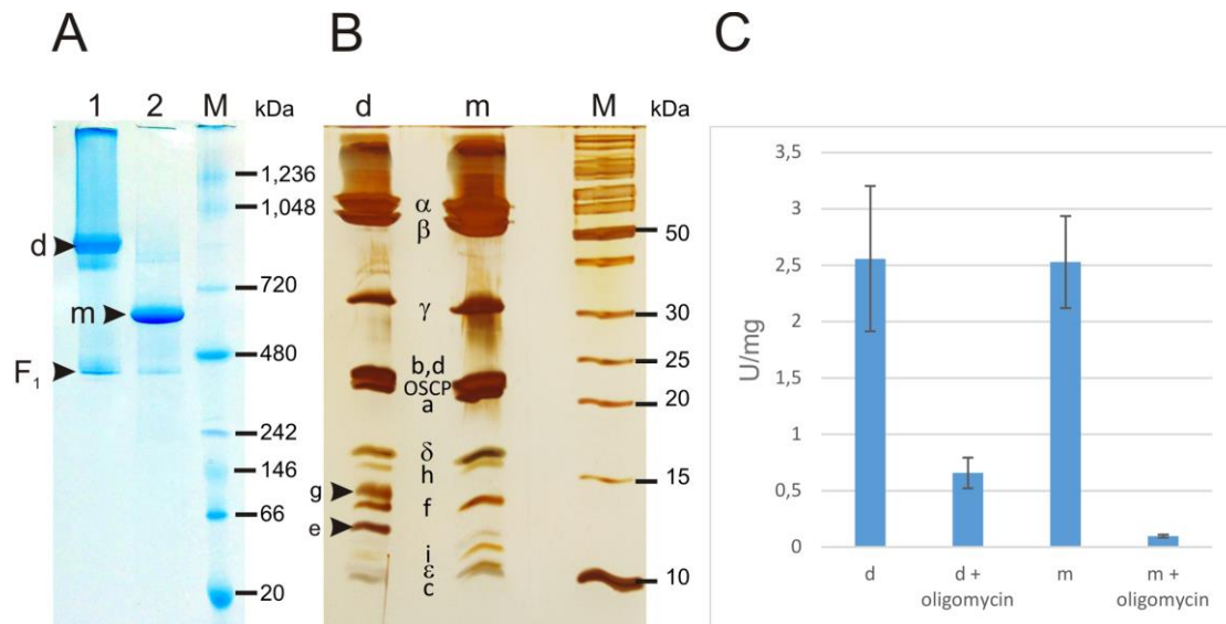
Figure S1, related to Figure 2. Subunit composition of monomeric and dimeric Y. lipolytica ATP synthase and ATP hydrolyase activities of purified ATPases. The (1) dimeric (digitonin) and (2) monomeric (dodecylmaltoside) purified ATP synthase samples were separated by (A) Blue Native-PAGE. Indicated protein complexes (d, m) were cut out of the gel and used for LC-MS analysis and 2 nd dimension SDS-PAGE. (B) ATP synthase subunits were separated in the 2 nd dimension SDS-PAGE using a 15% polyacrylamide gel, according to (Schägger and von Jagow, 1987). The subunits are indicated according to their molecular weight (Liu et al., 2015). Molecular weight markers (in kDa) are indicated on the right side of the gels. Arrow heads indicate the presence of subunit e and g only in the (d)dimer preparation but not in the (m)monomeric ATP synthase preparation. (C) Determination of ATP hydrolytic activities using the spectrophotometric coupled assay (Cook et al., 2003) and inhibition of ATP hydrolytic activity upon adding 5 \mu g/ml oligomycin (= 6.3 \mu M). Error bars are indicated ( n=3 ).
