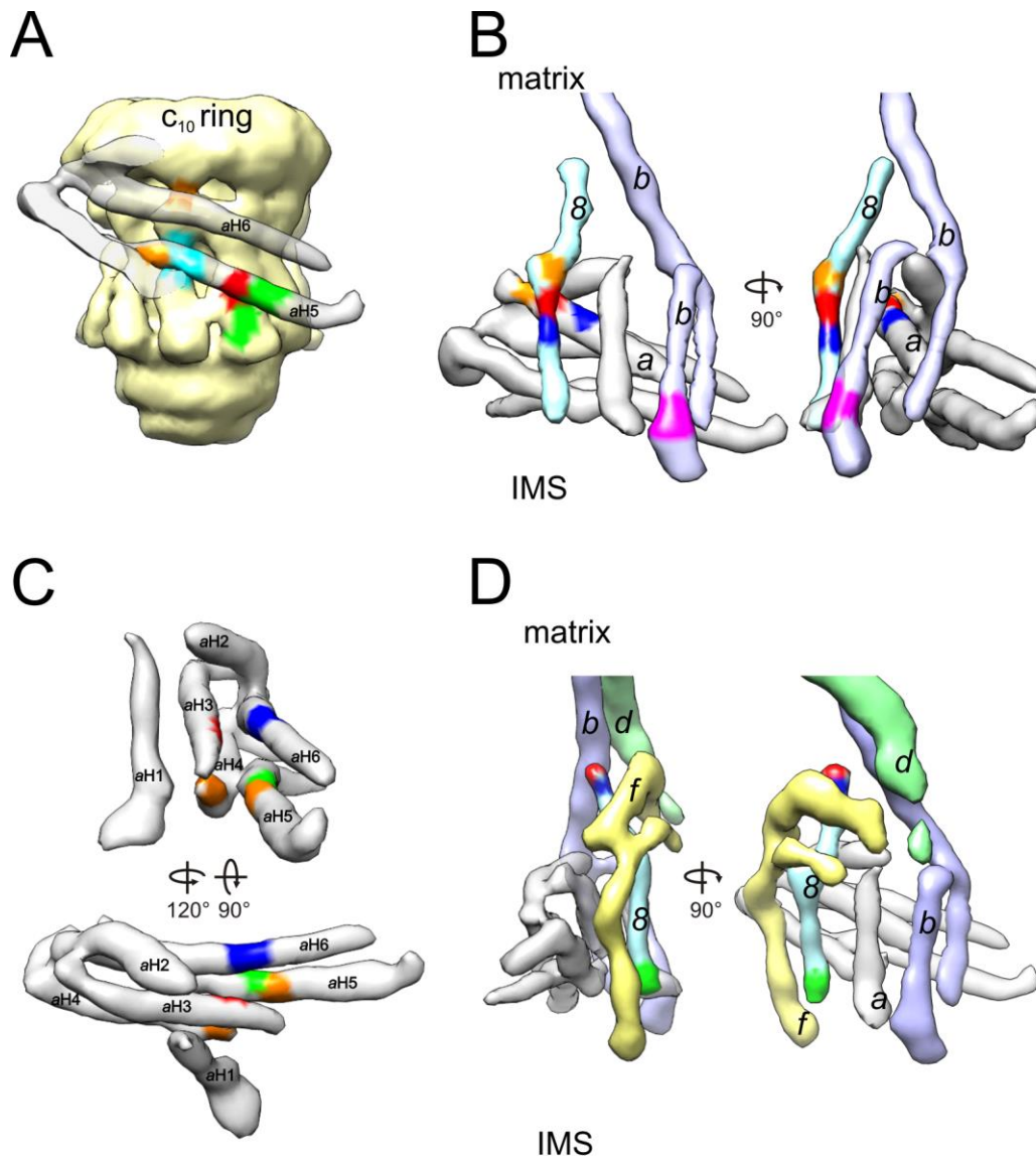
Figure S6, related to Figure 6. Cys-Cys crosslink positions in E. coli and S. cerevisiae . To verify the assignment of \alpha -helices in the F_0 region of the Y. lipolytica F_1F_0 dimer, we compared available crosslink studies for E. coli and S. cerevisiae (DeLeon-Rangel et al., 2013; Jiang and Fillingame, 1998; Schwem and Fillingame, 2006; Stephens et al., 2003) with our ATP synthase dimer model. By using multiple pairwise sequence alignment ESPript (Robert and Gouet, 2014) we generated a homology model and assigned corresponding amino acids in Table S3 . To visualize the crosslink positions, the crosslinks are shown as color pairs on the segmented cryo-EM volumes as indicated in Table S3 . (A) Cys-Cys crosslink positions of subunit aH5 to the c_{10} ring. The crosslink pairs follow the curvature of aH5 around the c_{10} ring. (B) Subunit \delta is in close proximity to aH2 and aH3 . Val111 and Pro112 of subunit a are located in the flexible loop region between aH3 and aH4 , which lies in close proximity to Ser55 from subunit b (pink). (C) Crosslink positions in the horizontal double hairpin between aH3 and aH5 (red/green), aH4 and aH5 (orange), aH3 and aH6 (red/blue) and aH5 and aH6 (green/blue). (D) Crosslinks between subunit \delta and subunit b , d and f (red/blue) on the matrix side. Our model places the N terminus of subunit \delta (green) and the C terminus of f in close proximity at the IMS, which also matches with S. cerevisiae crosslinks (Stephens et al., 2003).
