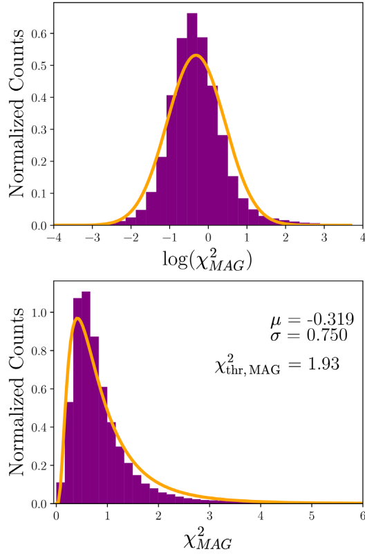
Figure B1. The MAGPHYS \chi^2 distribution of a filtered sub-sample of galaxies in the COSMOS field that have both MAGPHYS and CIGALE fits. The sources displayed here have \Delta z < 0.02(1+z) between the MAGPHYS and CIGALE catalogues. Upper: logged MAGPHYS \chi^2 values clearly display a Gaussian distribution. Purple is a histogram of the logged MAGPHYS \chi^2 values; orange is a Gaussian fit to the data. Lower: a lognormal fit to the MAGPHYS \chi^2 distributions, with calculated mean, \mu , standard deviation, \sigma , and subsequently calculated MAGPHYS \chi^2 threshold, \chi^2_{\text{thr,MAG}} displayed.
