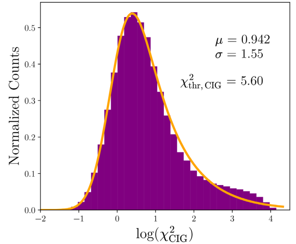
Figure B2. The CIGALE \chi^2 distribution of a filtered sub-sample of galaxies in the COSMOS field that have both MAGPHYS and CIGALE fits. The sources displayed here have \Delta z < 0.02(1+z) between the MAGPHYS and CIGALE catalogues. Logged CIGALE \chi^2 values clearly do not display a Gaussian distribution (purple histogram); as such, a lognormal distribution cannot be fitted to the data. Instead, an exponentially modified Gaussian distribution is fitted to the logged \chi^2 values (orange line). The calculated mean, \mu , standard deviation, \sigma , and subsequently calculated CIGALE \chi^2 threshold, \chi^2_{\text{thr,CIG}} are displayed.
