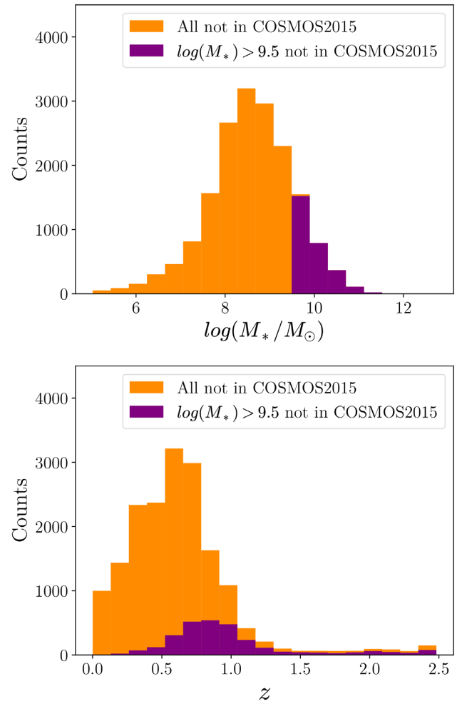
Figure C2. The stellar mass and redshift distribution of sources in the MAGPHYS catalogue but not in the COSMOS2015 catalogue. Orange marks all the sources; purple marks sources with \log(M_*/M_\odot) > 9.5 .
