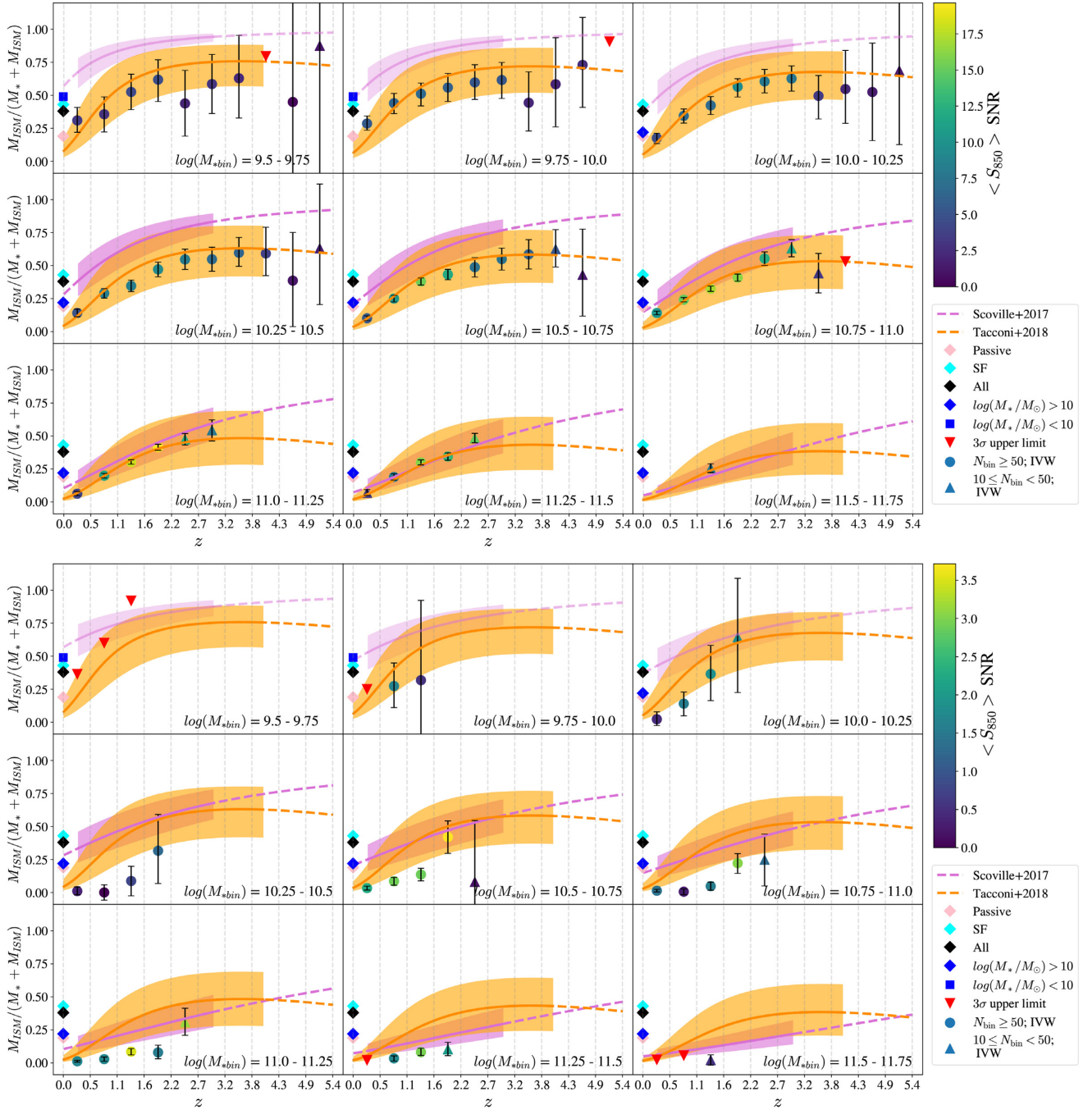
Figure 7. As in Fig. 5, here we show the resulting stacked ISM mass fractions with redshift, based on 850 \mu\text{m} fluxes in the COSMOS field, but now split into star-forming (top) and passive (bottom) sets. The filled circles are the IVW data for stacks with N \geq 50 . The filled triangles are the IVW data for stacks with 10 \leq N < 50 . The colour of the points represents the SNR of the stacked flux for that given point. The red triangles denote negative stacked fluxes; here, the 3\sigma error value is used to calculate an upper limit to the ISM mass fraction. The purple and orange lines are the scaling relations from Scoville et al. (2017) and Tacconi et al. (2018; shown as the dashed lines where the relationship extends beyond the redshift limit of their samples), for galaxies on the Main Sequence (MS). The average gas fraction based on 640 local galaxies (black diamond) is also shown at redshift zero (Pieter De Vis, private communication), defined as M_{\text{gas}}/(M_{\text{gas}} + M_*) (see the main text). We also split the local gas fraction into late-type and early-type galaxies (490 LTGs and 150 ETGs, the cyan and pink diamonds, respectively) and by stellar mass (373 galaxies with \log M_* < 10 and 267 galaxies with \log M_* > 10 , denoted by the blue square and diamond, respectively).
