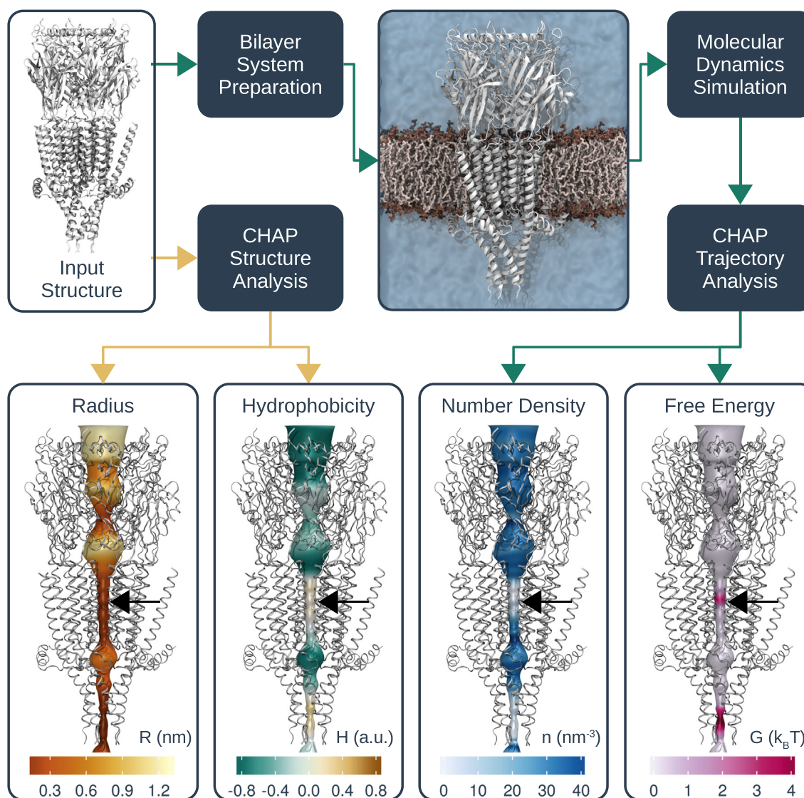
Fig. 2. Overview of workflow for functional annotation of ion channels with CHAP. Given a simple protein structure as input, CHAP can calculate pore radius and hydrophobicity profiles. In addition, the protein can be simulated in its native lipid bilayer environment in order to assess the behavior of water inside the channel pore. From the resulting simulation trajectory data, CHAP can derive water density and free energy profiles that aid the identification of hydrophobic gates. Yellow arrows indicate steps of the pipeline that can be carried out on structural data alone, while cyan arrows indicate those steps that are based on subsequent MD simulation. The black arrows indicate the location of the 9' ring of leucine residues in the middle of the hydrophobic gate in the transmembrane domain of the channel. There is a further free energy barrier within the intracellular domain, which coincides with a narrowing of the radius of the pore. In an open structure of the 5-HT 3 receptor, ions are thought to permeate lateral portals within the intracellular domain, thus bypassing this constriction.
