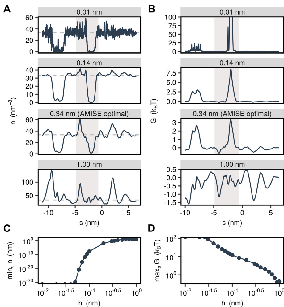
Fig. 7. Influence of bandwidth parameter. (A) Water number density along the permeation pathway of the 5-HT 3 receptor for various values of the kernel bandwidth. A value of 0.14 nm corresponds to the approximate size of a water molecule and a value of 0.34 nm corresponds to the statistically optimal bandwidth. (B) Corresponding free energy profiles calculated via Boltzmann inversion of the density profiles. The gray shaded area in panels A and B represents the transmembrane domain. (C) Minimum of number density profile in dependence of bandwidth. (D) Maximum of free energy profile in dependence of bandwidth.
