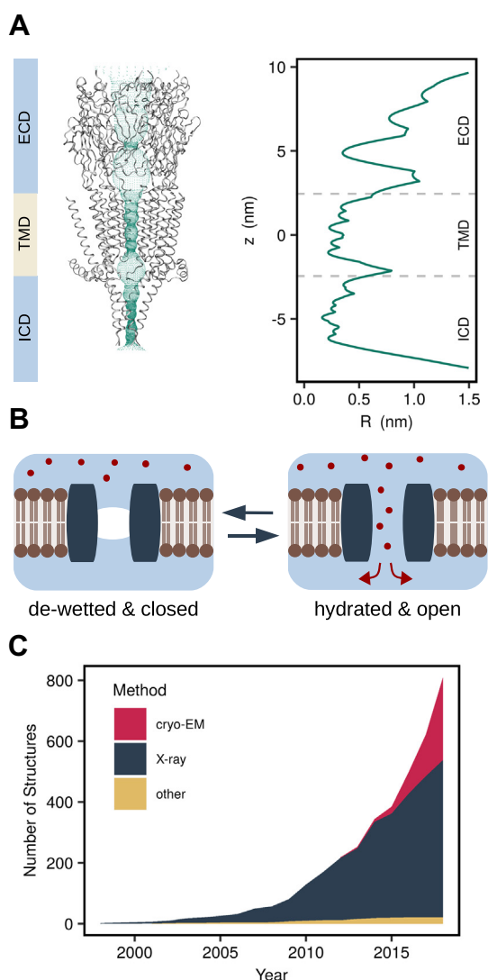
Fig. 1. Hydrophobic gates pose a challenge to the functional annotation of ion channel structures. (A) HOLE profile of the entire PDB structure of a 5-HT 3 receptor (PDB ID: 4PIR). The color bar indicates the extracellular (ECD), transmembrane (TMD), and intracellular (ICD) domains. (B) Hydrophobic gating: A non-conducting state is characterized by the de-wetting of a part of the permeation pathway lined by hydrophobic residues. Ions are prevented from crossing this region by the free energy barrier associated with their desolvation even if the pore is sufficiently large to accommodate them. (C) The number of ion channel structures deposited in the Protein Data Bank is growing exponentially (data retrieved on 5 December 2018).
