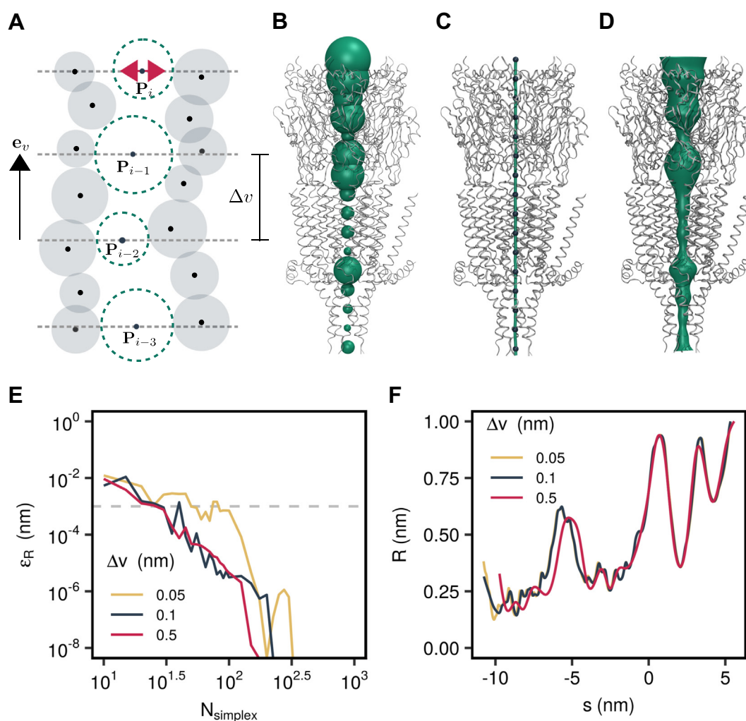
Fig. 5. Pore geometry calculations in CHAP. (A) Schematic representation of probe-based pathway finding. The position of a spherical probe is optimized in subsequent parallel planes to maximize its radius without overlapping the van der Waals sphere of any ion channel atom. (B) Configuration space view of probe positions (green spheres) in the permeation pathway of a 5-HT 3 receptor structure (PDB ID: 4PIR). For visual clarity, a large probe step of v = 1 nm was used here. (C) The probe center positions (blue spheres) are interpolated with cubic B-splines to yield a continuous spatial curve (green tube) representing the pore center line. (D) A surface representation of the channel pore is generated by extruding a circular cross section along the center line spline curve. (E) Convergence of the Nelder–Mead algorithm carried out to optimize the probe position in each parallel plane. The radius error falls below a threshold of 0.001 nm within 100 optimization steps irrespective of the value of the probe step. The reference radius profile is calculated with a very large number of 2000 Nelder–Mead iterations. (F) Influence of probe step on radius profile resolution. While a probe step of 0.5 nm only captures the general feature of the radius profile, decreasing the probe step from 0.1 to 0.05 nm leads only to minimal changes.
