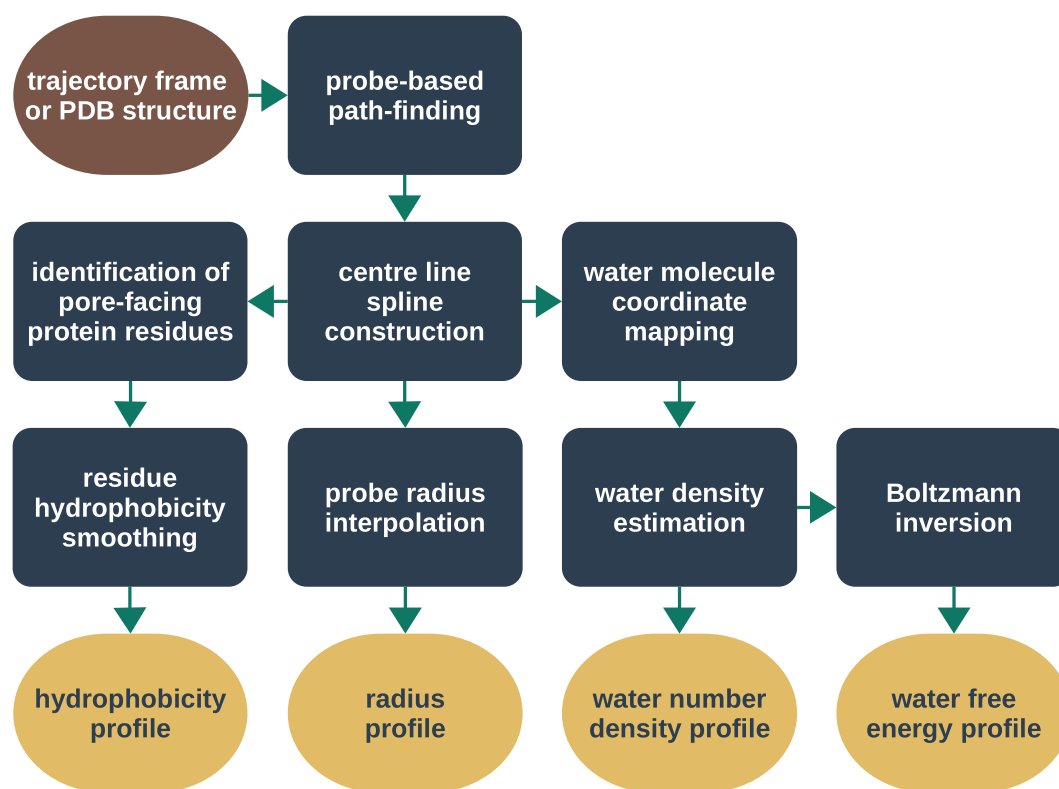
Fig. 4. Workflow diagram of data processing in CHAP. For an individual PDB structure, this procedure is carried out once. For trajectory data, the above procedure is carried out individually for each frame, that is, for each structural configuration at a sampled time point. The resulting hydrophobicity, radius, density, and free energy profiles are averaged over all time steps, and confidence bands are estimated from the standard deviation over time.
