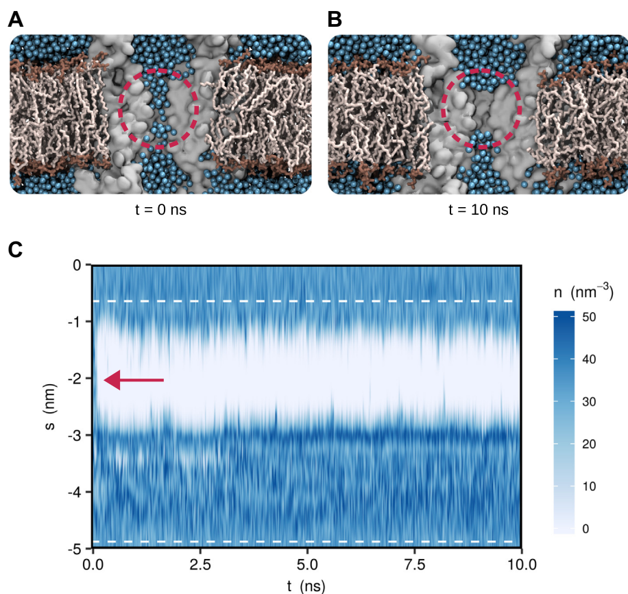
Fig. 3. Hydrophobic gates can be identified through equilibrium MD simulation. (A) Cross section of the starting structure for MD simulation of a 5-HT 3 receptor (PDB ID: 4PIR) embedded in a DOPC lipid bilayer. The protein is represented by a gray surface with two of five subunits omitted for visual clarity. Only the transmembrane (TM) domain is shown. Water oxygens are represented by blue spheres, and lipid molecules are shown in liquorice representation. Note that the entire channel pore is initially filled with water. (B) Snapshot from the MD trajectory clearly exhibiting a de-wetted region (highlighted with red circle) in the TM domain of the channel. Note that the channel pore is not physically occluded. (C) Water density profile in the receptor pore over time. An approximately 2-nm-long region of the TM domain indicated by a red arrow de-wets at the beginning of the simulation and remains devoid of water throughout.
