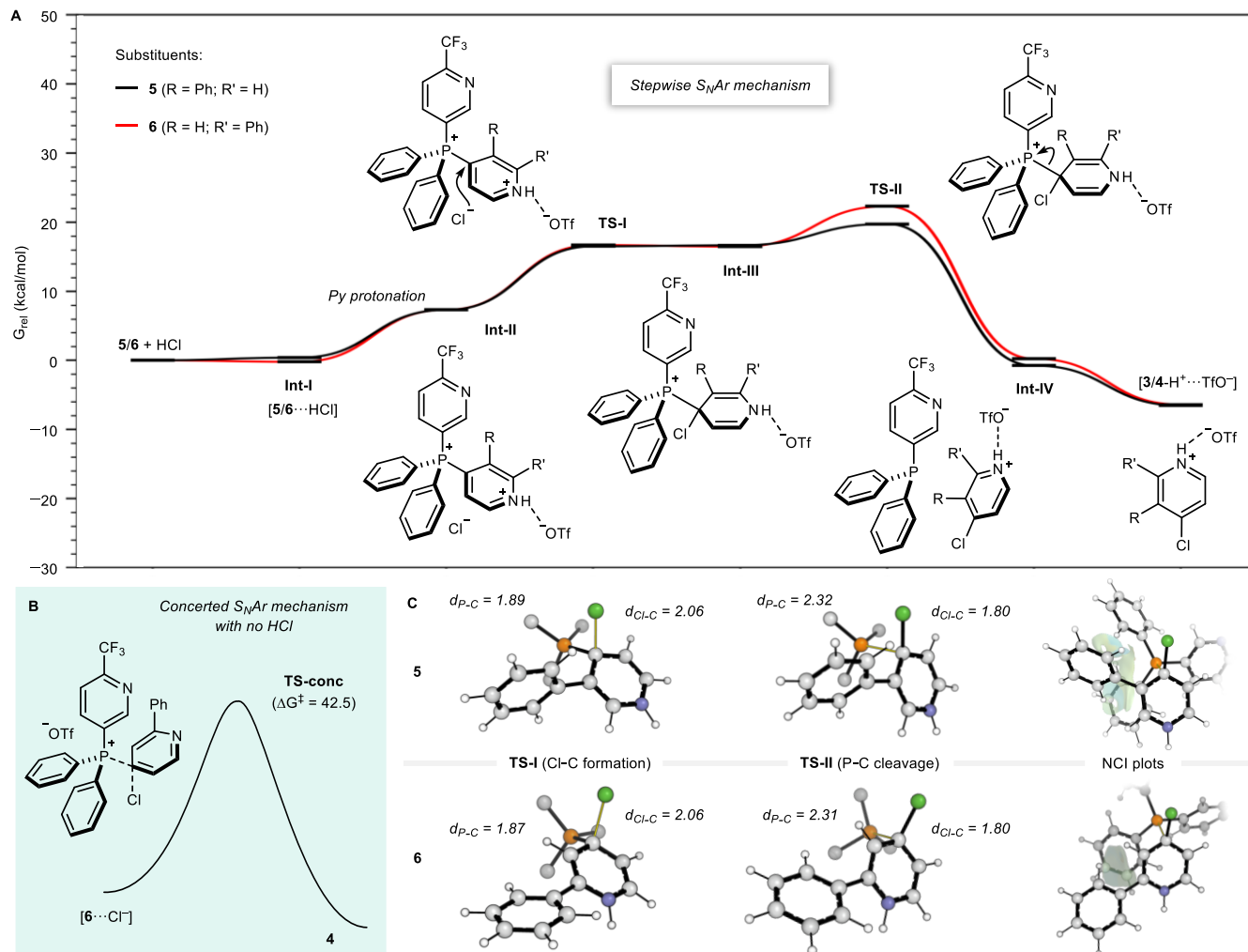
Figure 2. (A) Boltzmann weighted relative G in kcal/mol during the formation of products 3 (3-Ph substituent, black line) and 4 (2-Ph substituent, red line) at 80 °C ( \omega B97X-D/Def2-QZVPP// \omega B97X-D/Def2-SVP, SMD with 1,4-dioxane). (B) Reaction coordinate to form 4 when using Cl^- instead of HCl. \Delta G^\ddagger is shown in kcal/mol. (C) Representations of the most favorable TS-I and TS-II steps with P–C and Cl–C bond distances (in Å) when using 5 and 6 , along with NCIPlot 32 surfaces of the corresponding TS-II steps. Bonds involved in the TSs are represented as yellow lines. Phosphorus substituents and the TfO^- counteranion are omitted for clarity in some cases.
