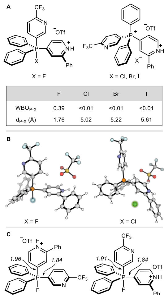
Figure 1. (A) WBO and distances of P-X bonds of the different species formed with phosphonium salts and different halogen anions. (B) Representation of the most stable conformers when using F and Cl atoms. (C) Lengths of axial and equatorial P-C bonds, in Å, in multiple conformations of the fluorophosphorane studied.
