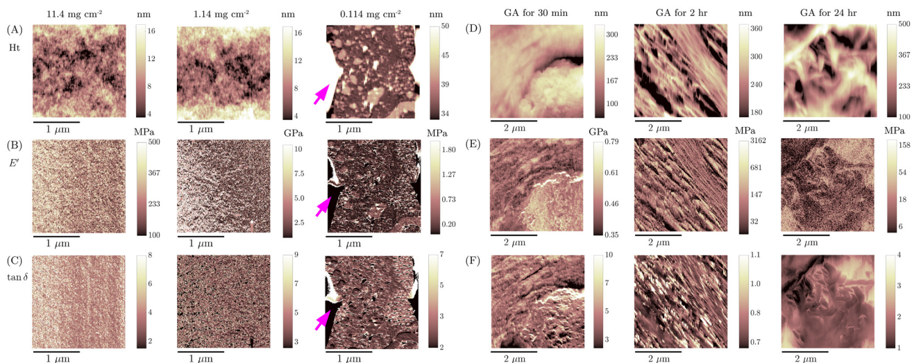
Fig. 3 Representative AM-FM AFM images of each substrate. Sample feature height (Ht) is shown in the top row for poly(HEMA) and pureCol substrates (A and D, respectively), storage modulus, E' , in the middle row (B and E, respectively), and loss tangent, \tan \delta , in the bottom row (C and F, respectively). Poly(HEMA) substrates were synthesized by successively diluting poly(HEMA) in ethanol, depositing the resulting solutions onto glass coverslips, and allowing the substrate to polymerize. The columns in A–C correspond to substrates with 11.4 mg of poly(HEMA) per \text{cm}^2 of sample surface area, 1.14 mg poly(HEMA) per \text{cm}^2 , and 0.114 mg poly(HEMA) per \text{cm}^2 , respectively. Magenta arrows indicate poly(HEMA) clumps in the 0.114 mg per \text{cm}^2 sample that interfered with quantification of E' and \tan \delta . PureCol substrates were synthesized by allowing pureCol (collagen I) to polymerize, then crosslinking the collagen with glutaraldehyde (GA) for varying amounts of time. The columns in D–F correspond to substrates crosslinked for 30 minutes, two hours, or 24 hours.
