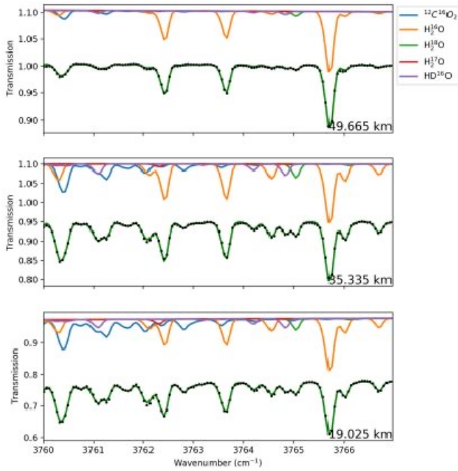
Figure 1: Example of one ACS MIR spectral window in diffraction order 224, measured at tangent heights of 19, 35 and 49.665 km. The black dots represent the measured spectra, and the green line shows the best fit to the data. The contribution from each spectra is also shown, following the colours in the legend.
