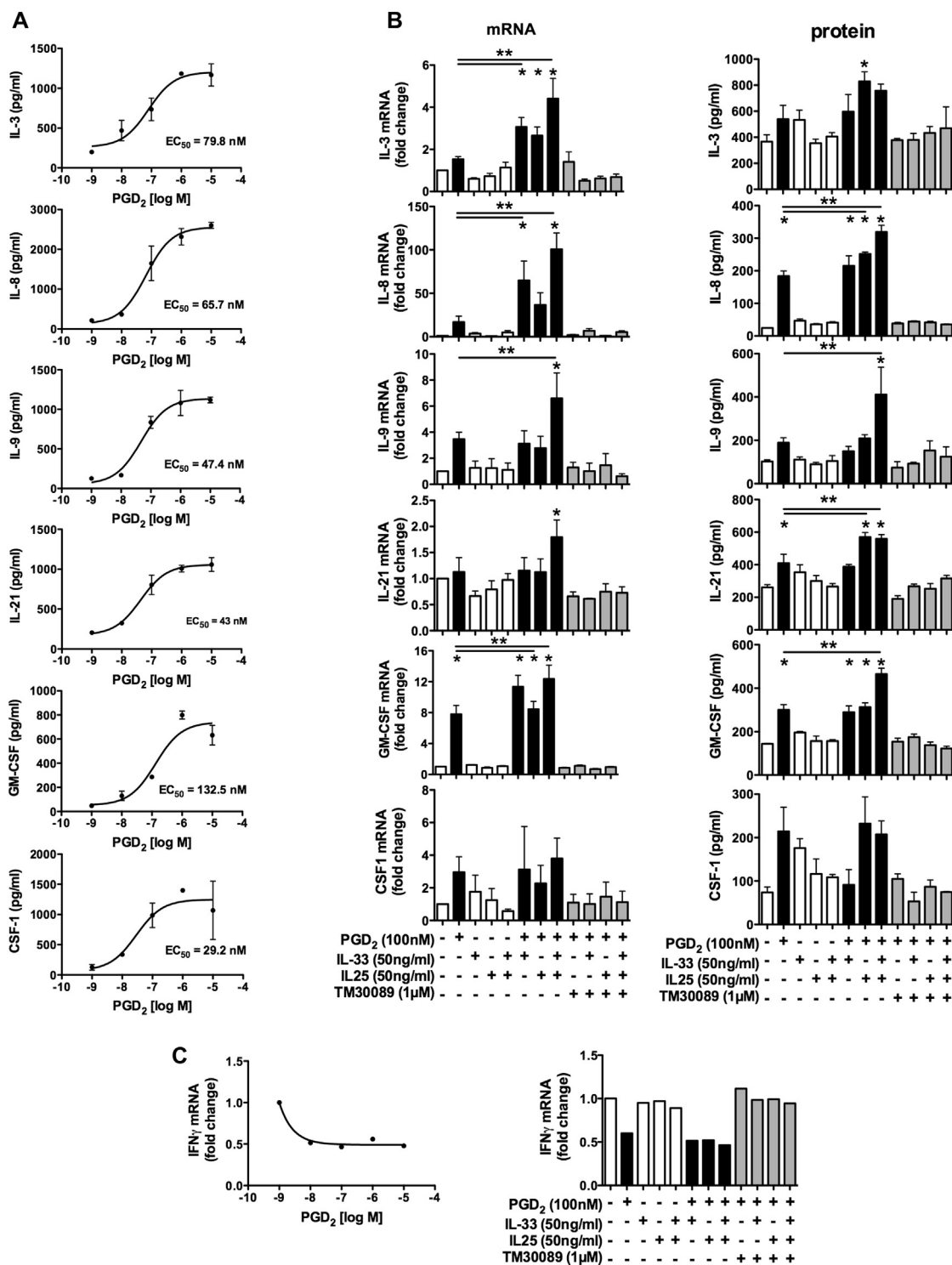
FIG 4. Activation of CRTH2 evokes proinflammatory cytokine production in ILC2s (skin). A , Cytokine concentrations after stimulation with PGD _2 . B , mRNA levels of cytokines (mRNA) and concentrations of cytokines (protein) after treatments, as indicated. C , mRNA level of IFN- \gamma after treatments. * P < .05 between control and other treatments and ** P < .05 between PGD _2 and indicated treatments ( n = 3).
