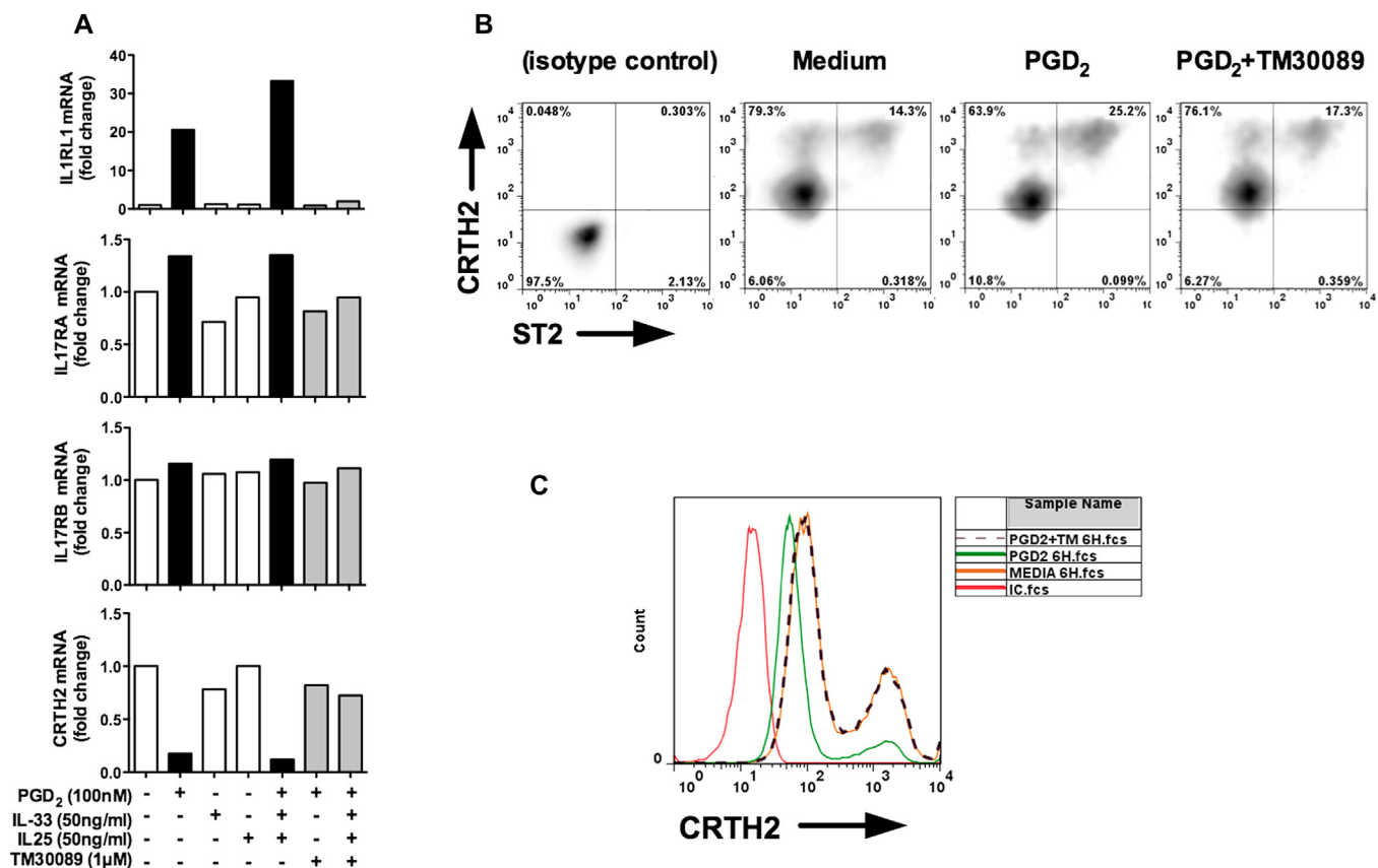
FIG 5. Activation of CRTH2 modulates receptor expression in ILC2s ( A , blood; B and C , skin). Fig 5, A, mRNA levels of receptor genes after treatments ( n = 3 ). The expression of ST2 (Fig 5, B) and CRTH2 (Fig 5, C) in ILC2s after incubation with medium or PGD 2 with or without TM30089 for 4 (Fig 5, B) or 6 (Fig 5, C) hours, as determined by using fluorescence-activated cell sorting, is shown.
