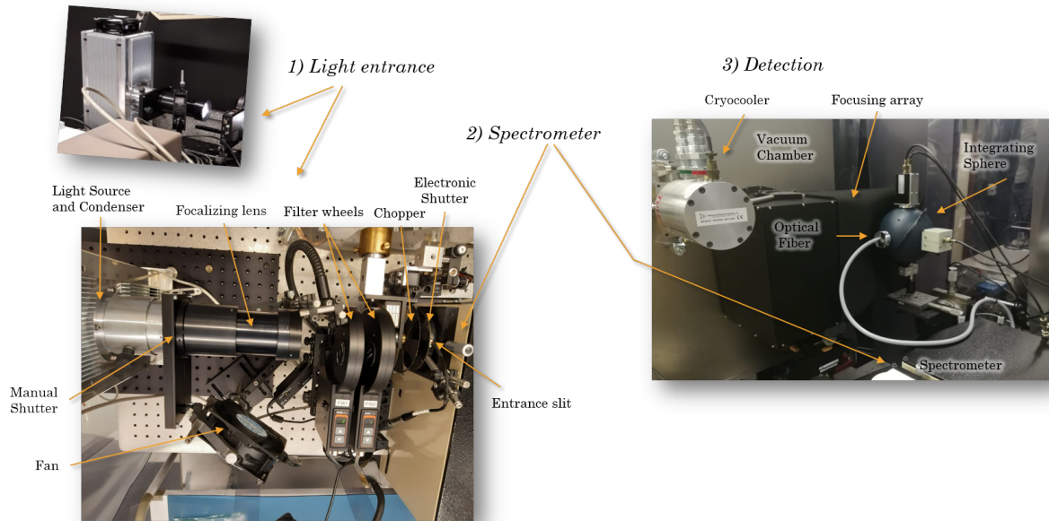
Figure 5. Opto-mechanical equipment of the MAJIS VIS-NIR facility: 1) light entrance, 2) spectrometer, and 3) detection blocks.
