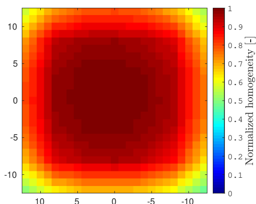
Figure 10. Characterization of the propagation function H(x, y) for the diffuse configuration of the facility that describes the inhomogeneity in the working plan of the facility. The vertical and horizontal dimensions are in mm.
