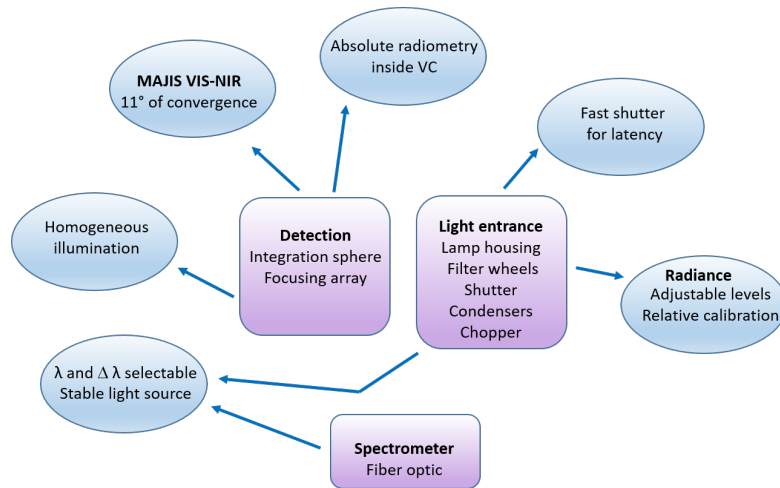
Figure 6. Interconnections between the opto-mechanical equipment of the facility and the performances specifications.
