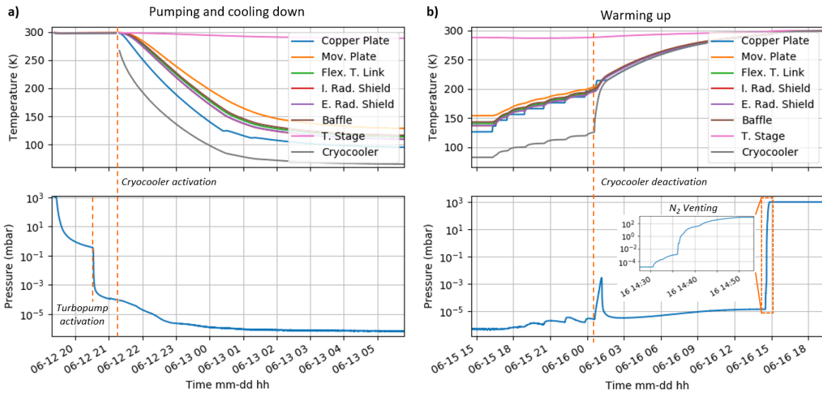
Figure 14. a) Pumping down of the vacuum chamber and coling down of the FPU mount, b) warming up of the FPU mount and N_2 venting of the vacuum chamber. This blank test allowed the characterization of the total waiting time to achieve the operating temperature of the FPA and the definition of the warming up process of the FPU. No FPU model was installed in the mount during this test.
