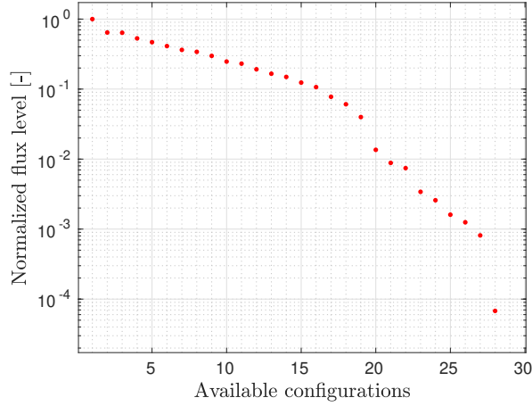
Figure 11. Distribution over three to four orders of magnitude of the level of illumination, using the filter wheels system of the facility.
