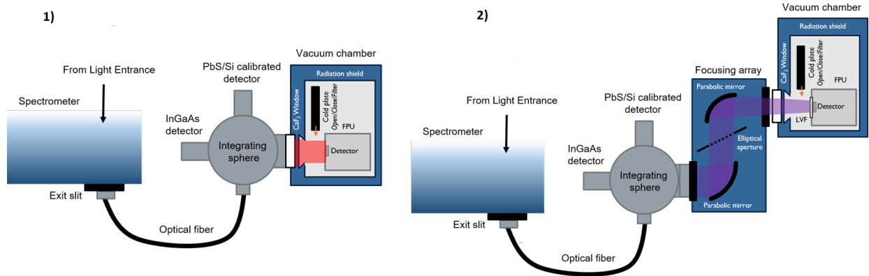
Figure 7. Configurations provided for a payload characterization (the MAJIS VIS-NIR FPU for instance): 1) uniform diffuse light beam, 2) uniform converging beam.
