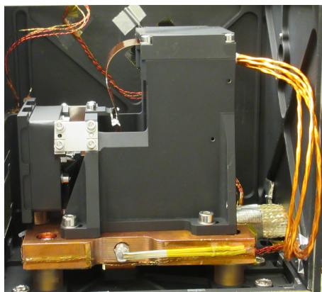
Figure 1. General view of the MAJIS VIS-NIR FPU as integrated in the facility.
