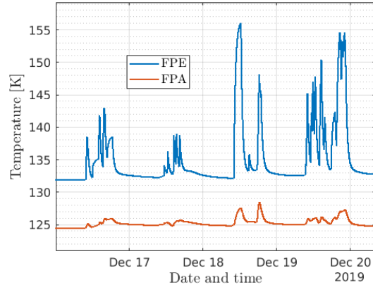
Figure 12. Thermal coupling between the FPE and the FPA, induced by the FPF during measurements; the temperature of the copper plate was stable. The high temperature increase observed on December 18, corresponds to the use of the high acquisition mode. The estimated amplification factor defined as the ratio between the temperature increase of the FPA and FPE is roughly around 10 % for the slow acquisition mode.
