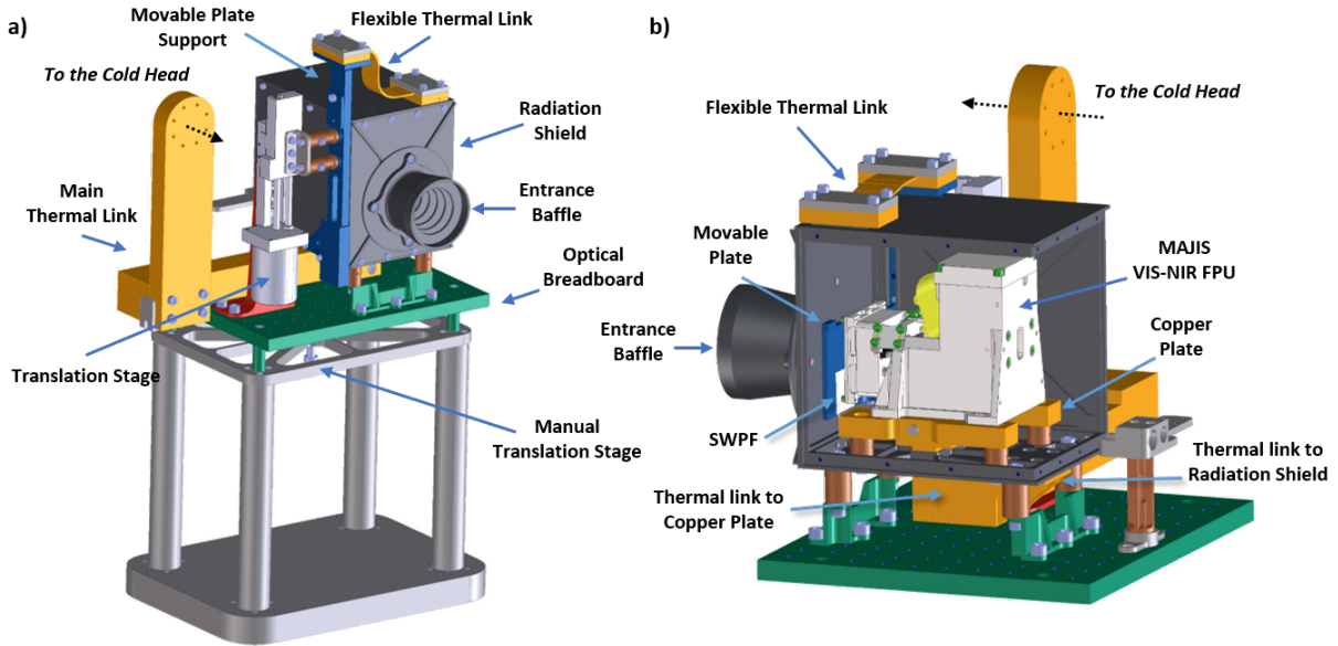
Figure 3. The FPU mount developed to support and thermalize the MAJIS VIS-NIR detector: a) Frontal view, b) internal view of the radiation shield. The optical breadboard (at room temperature) is mounted on a translation system for optical alignment.
