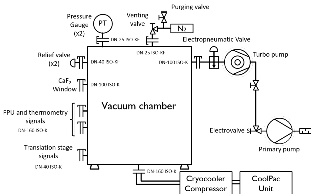
Figure 2. General vacuum diagram of the MAJIS VIS-NIR characterization facility.
