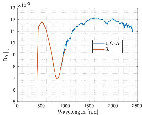
Figure 9. Spectral distribution of the transfer function R_0 as measured for the converging configuration of the facility.
