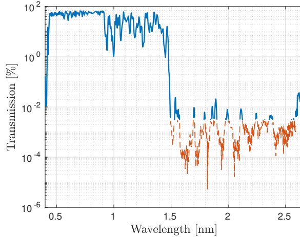
Figure 8. Transmission of the SWPF used for the MAJIS VIS-NIR project for straylight rejection of the optical path.
