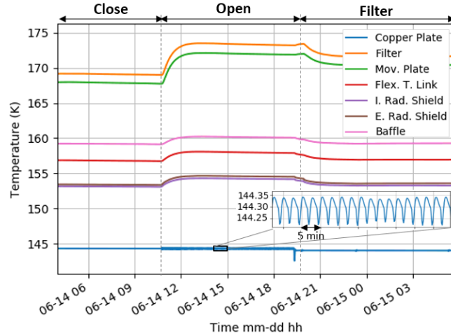
Figure 13. Temperature variations induced in the different components of the radiation shield when the movable plate changes position. A similar effect is expected in the FM FPU during its characterization. For this test, the copper plate was simulating the worst temperature case for the facility, so the movable plate overpasses by 1 K the temperature limit of 172 K in open position; the FPA would be around 150 K. It is not expected that the perturbations observed in the copper plate affect the stability of the temperature of the FPA during its characterization.
