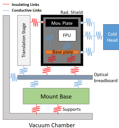
Figure 4. Thermal lumped scheme of the FPU mount.
