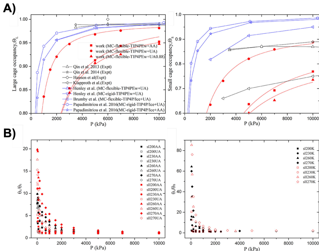
Fig. 4 A) Pressure dependence of CH 4 occupancy in large (left) and small (right) sl cages at ~270 K. Red, blue, and black symbols correspond to Qiu et al. , 63 previous simulations, 64–67 and experiments. 68–71 B) Temperature- and pressure-dependent occupancy ratios \theta_L/\theta_S for CH 4 (left) and CO 2 (right) in sl and sII hydrates; \theta_L and \theta_S denote fractions of large and small cages filled. Panels A) and B) adapted from Qiu et al. 63 Copyright © 2018 American Chemical Society.
