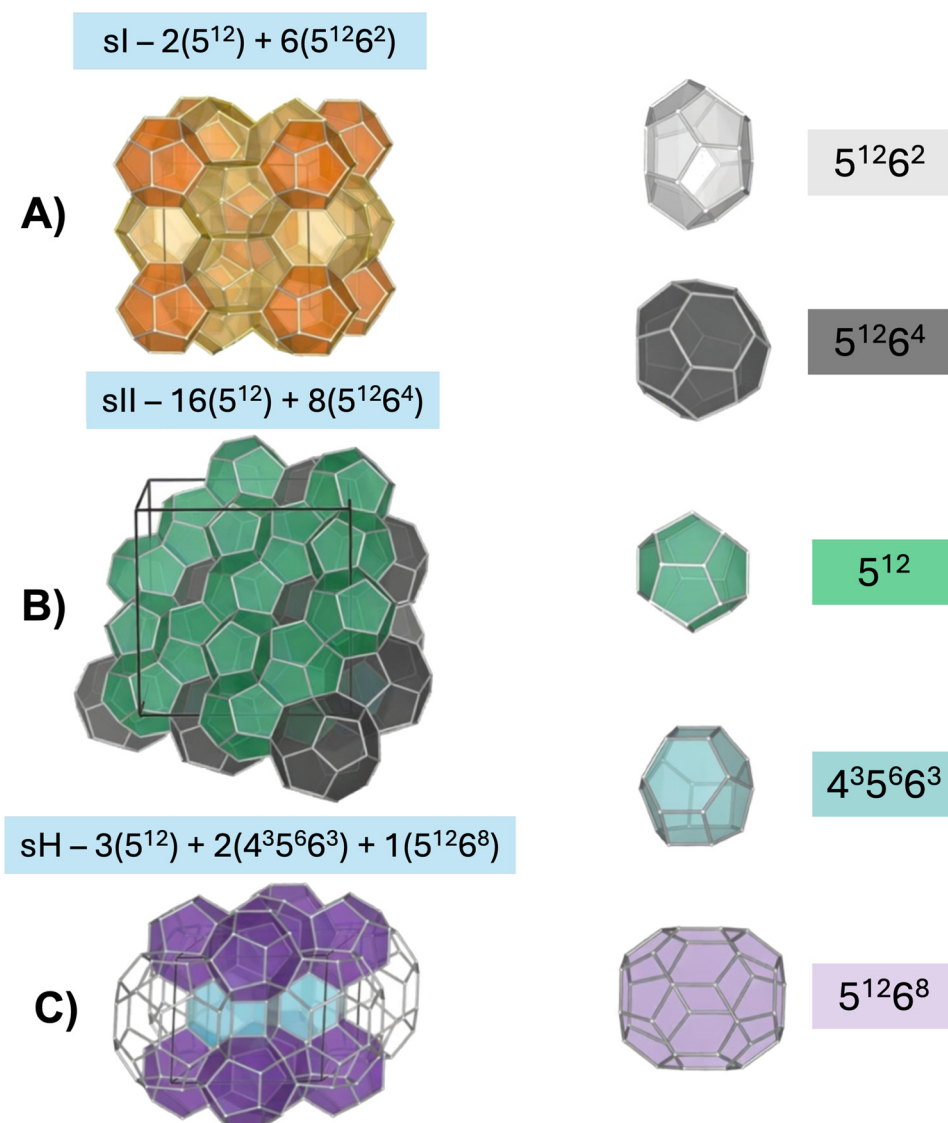
Fig. 1 Three main hydrate structures—sI (A), sII (B), and sH (C) with different host water cages. Adapted from Hassanpouryouzband et al. 2 Copyright © 2020 Royal Society of Chemistry.
