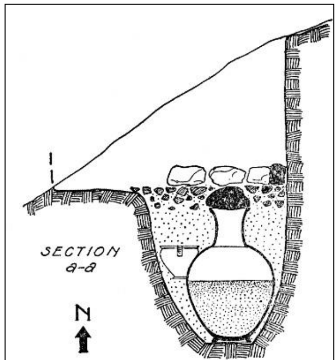
Plate 7 c & d: Sections of ATT22 . After the Agora excavations website ( http://agathe.gr/id/agora/image/1997.20.0036 ; http://agora.gr/id/agora/image/1997.20.0034 ) accessed 21/02/2014.
