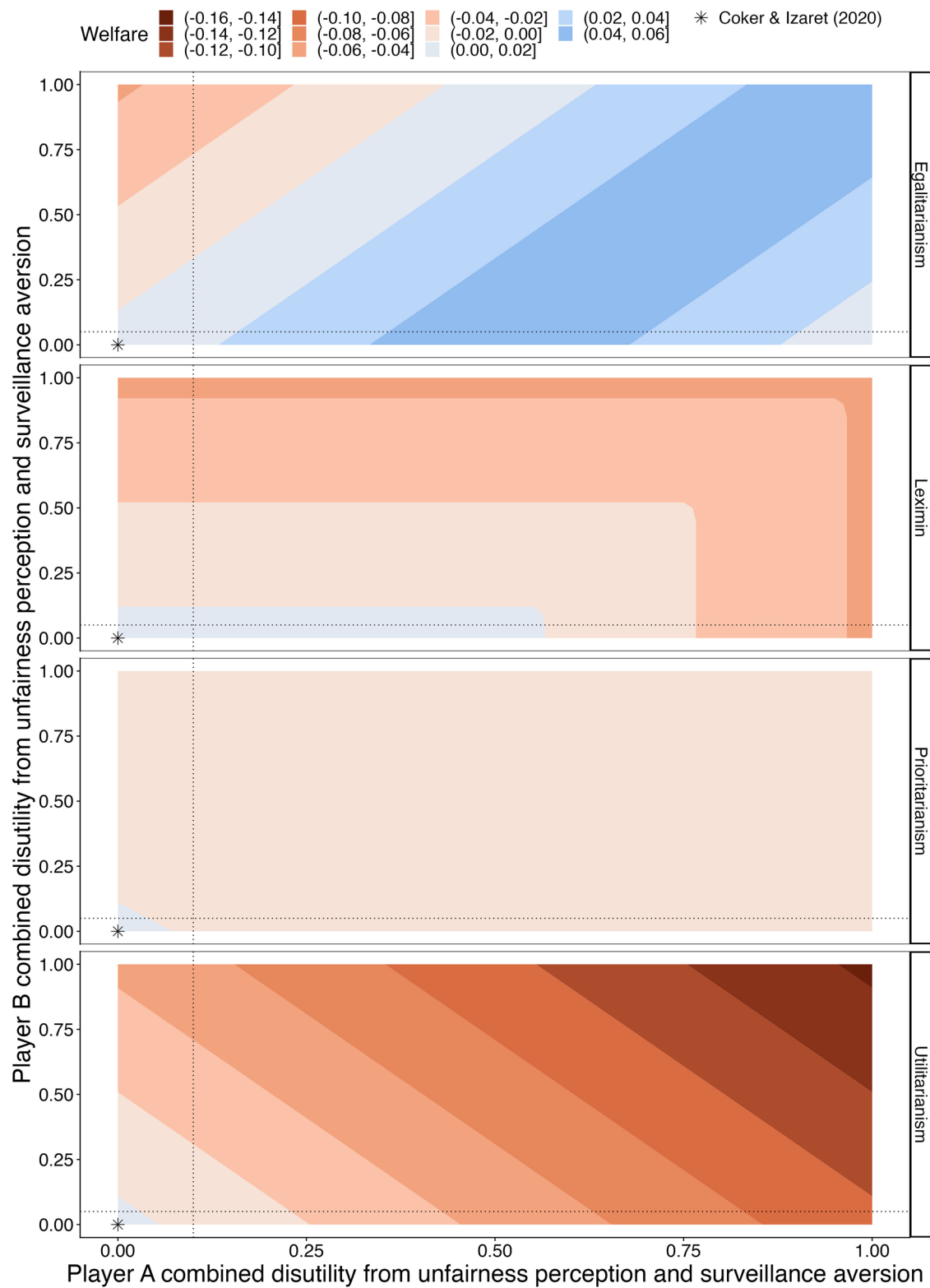
Fig. 5 Difference in welfare under personalized pricing versus unitary pricing for any level of loss incurred by player A and player B expressed as a percentage of the utility from the purchase. Dashed line reflects our initial specification of additive proportional loss
