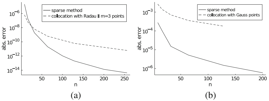
Fig. 2 a shows absolute error between analytic and computed solutions for Eq. 17 and b for Eq. 18 for approximations of order n . The errors for the collocation method are taken directly from Tables 1 and 2 in [47]. For the errors with our method, the bandwidth was set to increase to convergence; see Table 2 for a bandwidth-based view of errors
