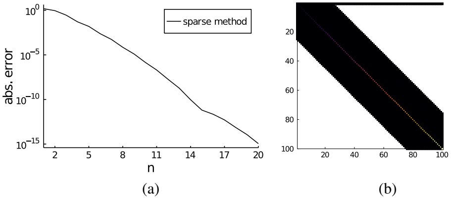
Fig. 4 a shows absolute error between analytic and computed solutions for u_1 in Eq. 20 for polynomial approximation of order n , b shows quasi-bandedness of full sparse method operator for n = 100
