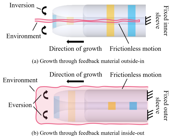
Fig. 1. Comparison of growing manipulators: The fundamental difference between (a) our new inversion robot and (b) the well-known eversion robot is that our manipulator grows by feeding material from the outside to the inside rather than feeding material from the inside to the outside, as is the case for the traditional eversion robot. Hence, our robot will introduce frictionless motion between the robot and the external environment that is encapsulated by the inner sleeve.
