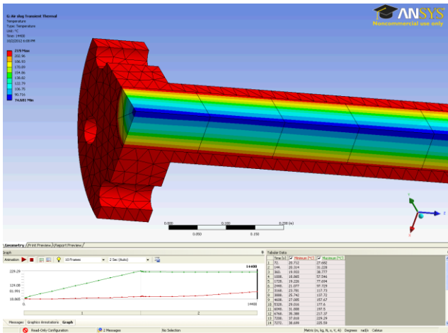
Figure 8. Temperature distribution through the stagnant test gas within the HDT, for 2 hours of active heating to ~500K and 2 further hours of conductive heat spread with no heat addition or loss ( T=75\text{--}219^\circ\text{C} ).
