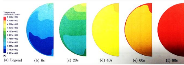
Figure 11. Evolving temperature distributions during the test gas heat up for preheat of 500K and a fill pressure of 50bar ( T=298\text{--}500\text{K} ).
