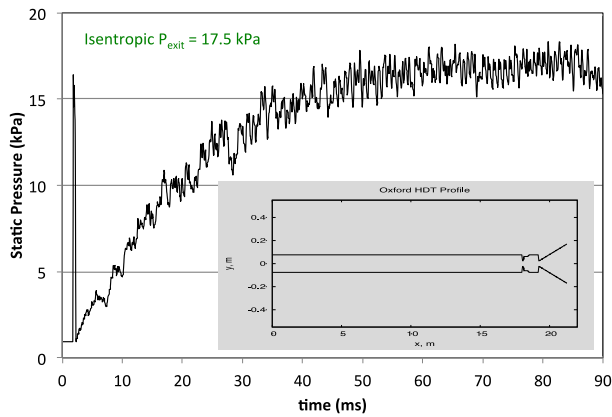
Figure 3. L1D calculation of the pressure history at exit of the HDT nozzle with incorporation of the plug valve and plenum geometry for a fill pressure of 276bar and preheat of 500K.
