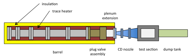
Figure 5. Schematic layout of the HDT showing the heated and insulated Ludwig tube supplying the hypersonic nozzle.
