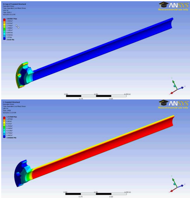
Figure 7. Transient thermal-structural simulation of stress distribution in a section of the HDT for preheat of 500K comparing the cases of (a) no internal pressure (Stress=0.2–27MPa) and (b) for a fill pressure of 276bar (Stress=1–120MPa).
