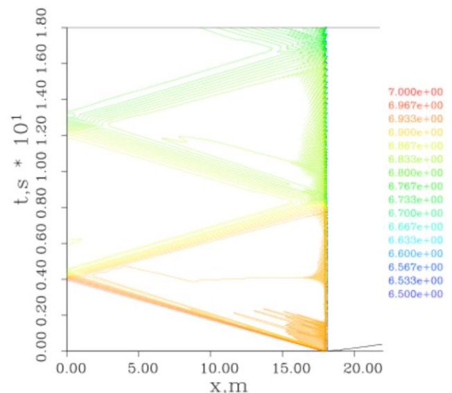
Figure 1. Example x-t diagram of flow in the HDT for fill pressure of 90 bar and preheat of 500K showing the passage of the expansion wave through the Ludwieg tube. (add key)
