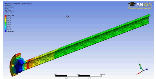
Figure 6. Temperature distribution in a section of the HDT Ludwig tube for preheat to 673K for 3 hours using 13.9\text{kW/m}^2 on the flange, 8.3\text{kW/m}^2 near the flange and 3.6\text{kW/m}^2 on the tube ( T= 393\text{--}405^\circ\text{C} ).
