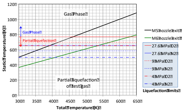
Figure 4. Plot of the static temperature at the exit of M5 and M6 nozzles, assuming isentropic expansion, as a function of the preheat temperature, superimposed on the liquefaction thresholds for N_2 and O_2 at a range of charge pressures.
