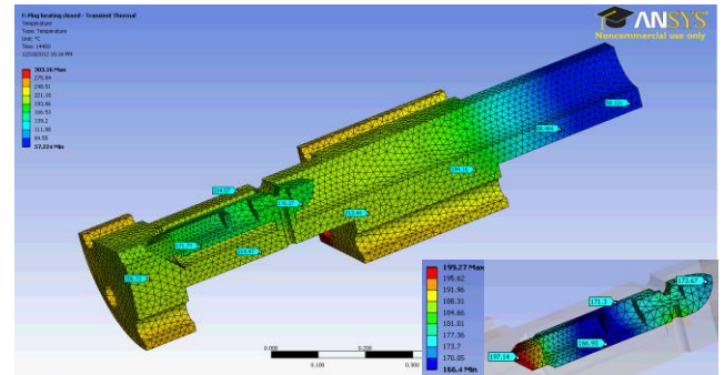
Figure 13. Temperature distribution in the plug valve assembly for a 3-hour, 500K wall preheat ( T=57\text{--}303^\circ\text{C} , T=166\text{--}199^\circ\text{C} ).
