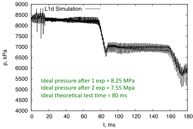
Figure 2. L1D calculation of the nozzle supply static pressure for a fill pressure of 90bar and preheat of 500K showing the pressure steps resulting from the passage of the expansion wave.
