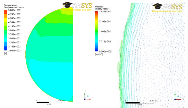
Figure 10. Distribution of (a) temperature ( T=298\text{--}500\text{K} ) and (b) flow velocity ( V=0\text{--}0.3\text{m/s} ) in the tube during preheating
