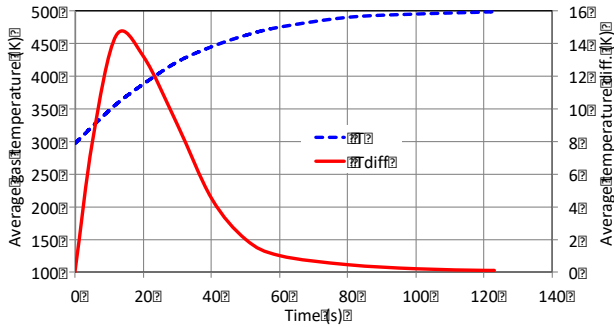
Figure 12. Plot of histories of (a) average gas temperature and (b) maximum temperature variation in the test gas for preheat of 500K and a fill pressure of 50bar.
