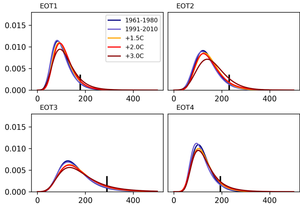
Fig. 10 Generalized Extreme Value distribution fit to EOT base region intensity distributions (mm/5-day) during five periods: 1961–1980 and 1991–2010 historical periods (dark and light blue respectively), + 1.5, + 2 and + 3 °C projection periods based on the SSP370 scenario (orange, red and dark red lines). The black vertical lines show the position of the 95th percentile from the 1961–1990 period
