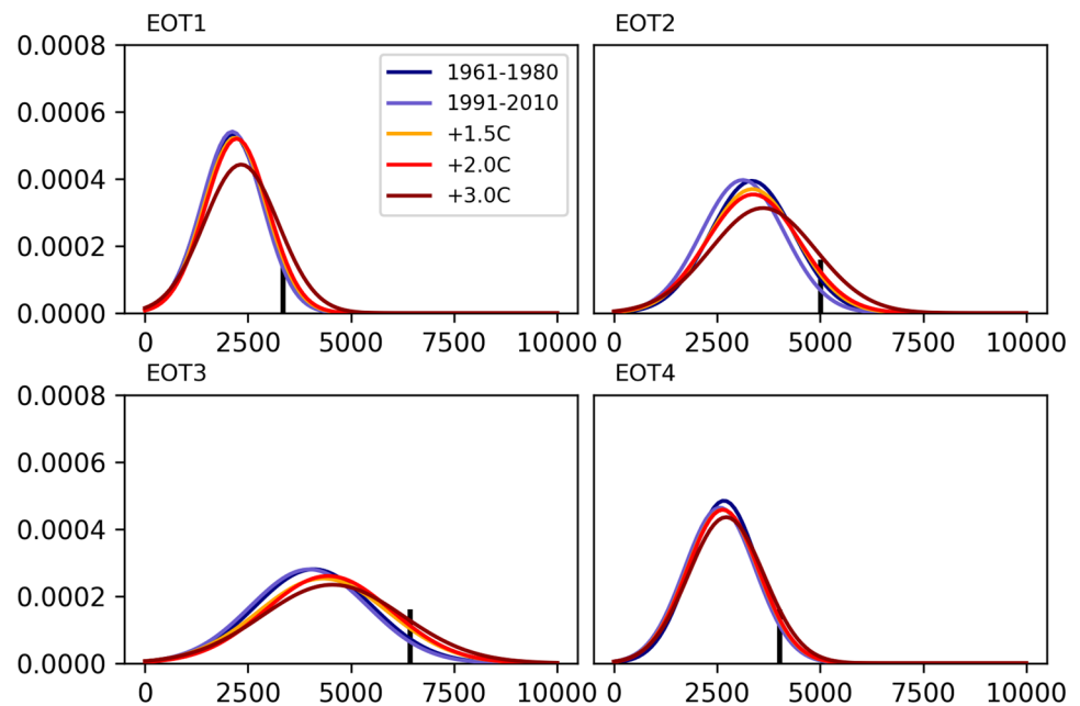
Fig. 11 Same as Fig. 10 but for the total JJA seasonal precipitation at EOT base region (mm) using a normal distribution
