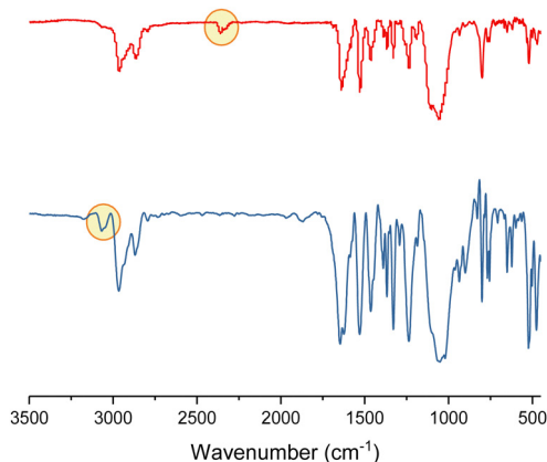
Fig. 1 IR spectra of 1 (blue) and its deuterated analogue: [\text{D}_2^{\text{Bu,DippL}}][\text{BF}_4] (red). The corresponding NH and ND signals are highlighted.
