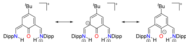
Fig. 3 The accessible resonance forms of the bis-iminium phenoxy-imine cation.
