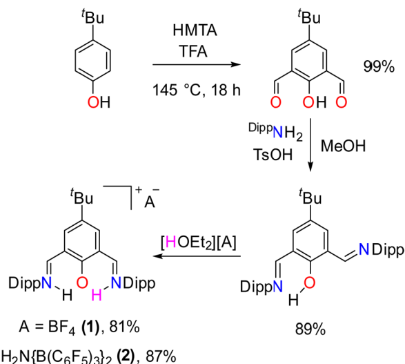
Scheme 1 Three-step syntheses of bis(iminium)phenoxide salts [\text{H}_2^{\text{Bu,DippL}}][\text{BF}_4] ( 1 ) and [\text{H}_2^{\text{Bu,DippL}}][\text{H}_2\text{N}\{\text{B}(\text{C}_6\text{F}_5)_3\}_2] ( 2 ). Dipp = 2,6- i -Pr 2 -C 6 H 3 .
