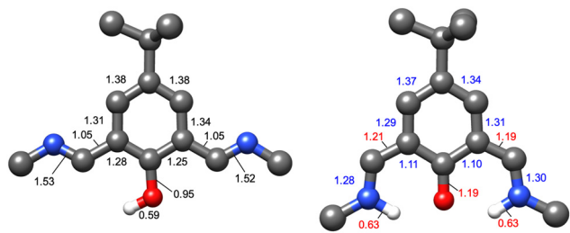
Fig. 5 Computed delocalisation indices – \delta(A,B) – for H^{tBu,DippL} (left) and 1 (right); reported in red are the values that increase upon formation of 1 , whereas those reported in blue are seen to decrease.
