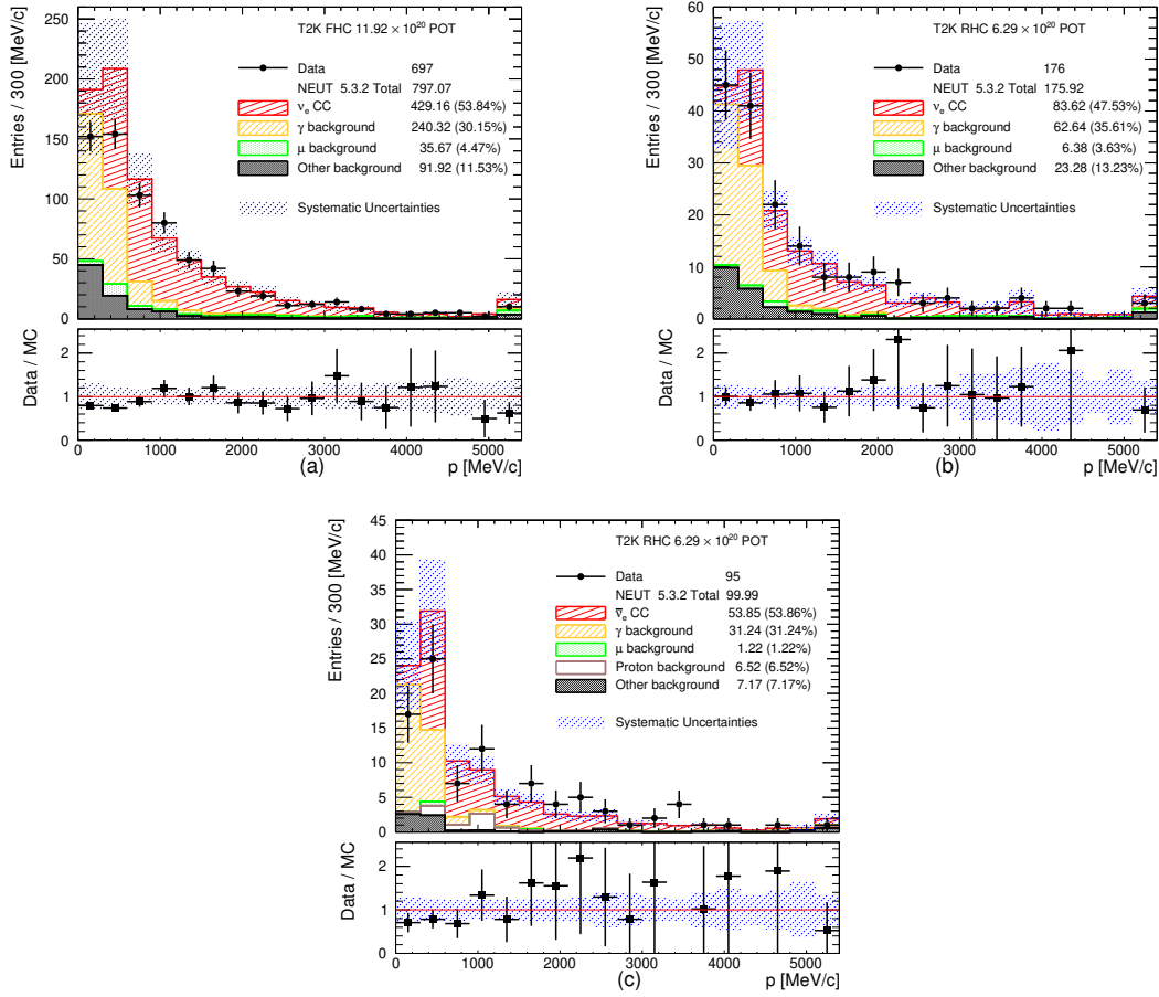
Figure 8. Momentum distribution of the selected electron and positron candidates for (a) FHC CC- \nu_e , (b) RHC CC- \nu_e and (c) RHC CC- \bar{\nu}_e . The number of MC events is normalized to the data POT. The effect of the total systematic uncertainty on the MC event yields (see section 6 for details) is also shown on these plots. The last bin is the overflow bin.
