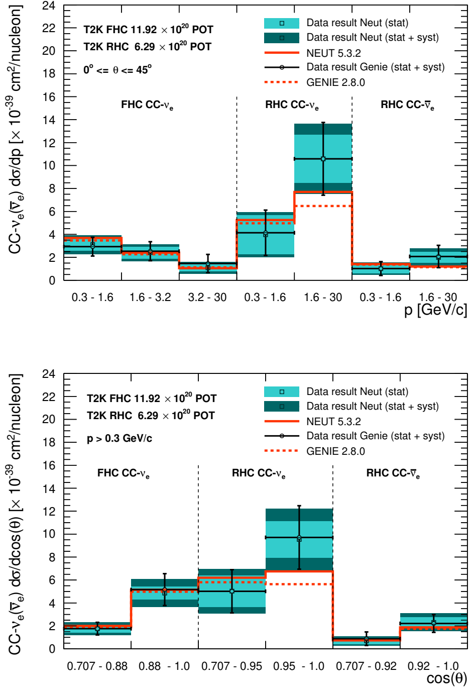
Figure 17. CC- \nu_e and CC- \bar{\nu}_e inclusive cross-section results in d\sigma/dp (top) and d\sigma/d\cos(\theta) (bottom) in a limited phase-space ( p > 300 \, \text{MeV}/c and \theta \leq 45^\circ ). The statistical uncertainty is computed by fixing all the nuisance parameters to their post-fit nominal values and redoing the fit. The systematic uncertainty is computed by subtracting in quadrature the statistical uncertainty from the total uncertainty.
