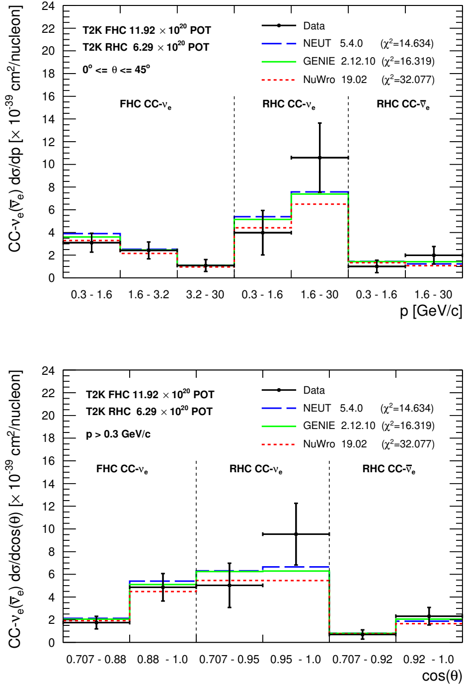
Figure 19. Flux integrated CC- \nu_e and CC- \bar{\nu}_e inclusive cross-section results in a limited phase-space ( p > 300 MeV/c and \theta \leq 45^\circ ) with comparisons to neutrino generator models from NEUT 5.4.0, GENIE 2.12.10 and NuWro 19.02 obtained using the NUISANCE framework. The top plot shows the results in momentum and the bottom plot the results in scattering angle. The \chi^2 is the total from the combined measurements in momentum and \cos(\theta) .
