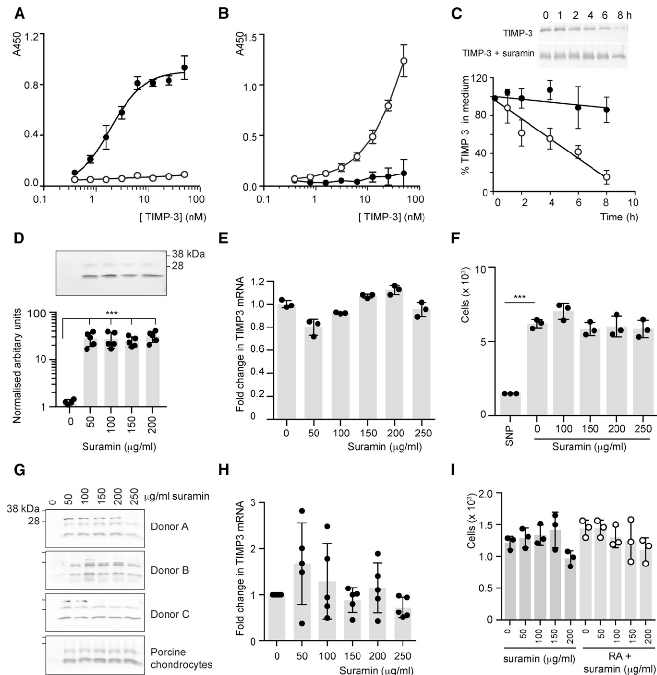
Fig. 1. Suramin binds to TIMP-3 and inhibits its cellular endocytosis by LRP1. (A) Glycosaminoglycan-binding 96-well plates were coated with suramin (10 µg/ml in PBS, filled circles) or PBS (open circles) and blocked in 0.2% gelatin in PBS. Wells were then incubated with TIMP-3 (0.4–50 nM) and binding was detected using an M2 anti-FLAG antibody (mean ± S.D., n = 3 ). (B) Medium-binding 96-well ELISA plates were coated with LRP1 (5 nM) and blocked with 10% BSA in TNC buffer. Wells were then incubated with TIMP-3 (0.4–50 nM), either alone (open circles) or preincubated with suramin (filled circles, 200 µg/ml, 1 hour, 37°C) and binding was detected using an M2 anti-FLAG antibody (mean ± S.D., n = 3 ). (C) HTB94 cells were incubated with recombinant TIMP-3 (1 nM) or TIMP-3 preincubated with suramin (200 µg/ml, 1 hour, 37°C) for 0–8 hours and TIMP-3 remaining in the medium was analyzed by immunoblotting and densitometry (mean ± S.D., n = 4 ). TIMP-3 (open circles) was taken up from the medium with a half-life of 4.0 \pm 1.3 hours, whereas TIMP-3 preincubated with suramin (filled circles) was minimally endocytosed. (D) HTB94 chondrosarcoma cells were incubated with suramin (50–200 µg/ml) in serum-free DMEM for 30 hours. Conditioned media were concentrated by TCA precipitation and TIMP-3 levels were analyzed by immunoblotting and densitometry. Values are expressed relative to the amount of TIMP-3 in the medium of untreated cells, defined as 1 (mean ± S.D., n = 5 ; *** P \leq 0.001 by one-way ANOVA with Bonferroni's correction). (E) HTB94 chondrosarcoma cells were treated with suramin (0–250 µg/ml, 18 hours) and expression of TIMP-3 mRNA was analyzed by quantitative PCR relative to RPLP0. TIMP-3 expression in the absence of suramin was defined as 1 (mean ± S.D., n = 3 , P > 0.05 by one-way ANOVA with Bonferroni's correction). (F) HTB94 cells were treated with suramin (0–250 µg/ml) or sodium nitroprusside (10 mM) for 72 hours and cell viability was assessed using MTS (mean ± S.D., n = 3 ; *** P \leq 0.001 by one-way ANOVA with Bonferroni's correction). (G) Primary chondrocytes were isolated from human OA or porcine cartilage and incubated with suramin (0–250 µg/ml) in serum-free DMEM for 48 hours. Conditioned media were concentrated by TCA precipitation and TIMP-3 levels were analyzed by immunoblotting. (H) Human OA chondrocytes were treated with suramin (0–250 µg/ml, 48 hours) and expression of TIMP-3 mRNA was analyzed by quantitative PCR relative to RPLP0, with expression in the absence of suramin defined as 1 ( n = 5 donors, mean ± S.D., P > 0.05 by one-way ANOVA with Bonferroni's correction).
