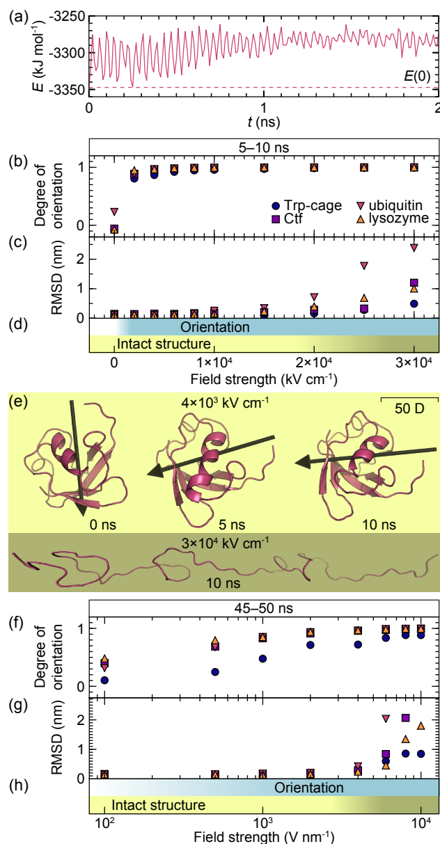
Figure 2: (a) The total internal energy – not including the dipole–field energy – during the first 2 ns of a ubiquitin simulation with a 4000 \text{ kV cm}^{-1} field. The dashed line shows the energy at t = 0 . Fig. S3(a) is based on the same simulation. (b) The degree of orientation and (c) RMSD of the C_{\alpha} over the last 5 ns of 10-ns simulations. (d) The regimes where orientation can be achieved and where nativelylike structures are preserved on the 10 ns timescale. (e) Snapshots from a simulation of ubiquitin at 4000 \text{ kV cm}^{-1} [same as in (a)], and one extreme case at 30\,000 \text{ kV nm}^{-1} . (f)–(h) Analogous to (b)–(d) for the 50-ns simulations (note the logarithmic x-axis). See Figs. S5–S10; Supplemental Videos 1 and 2.
