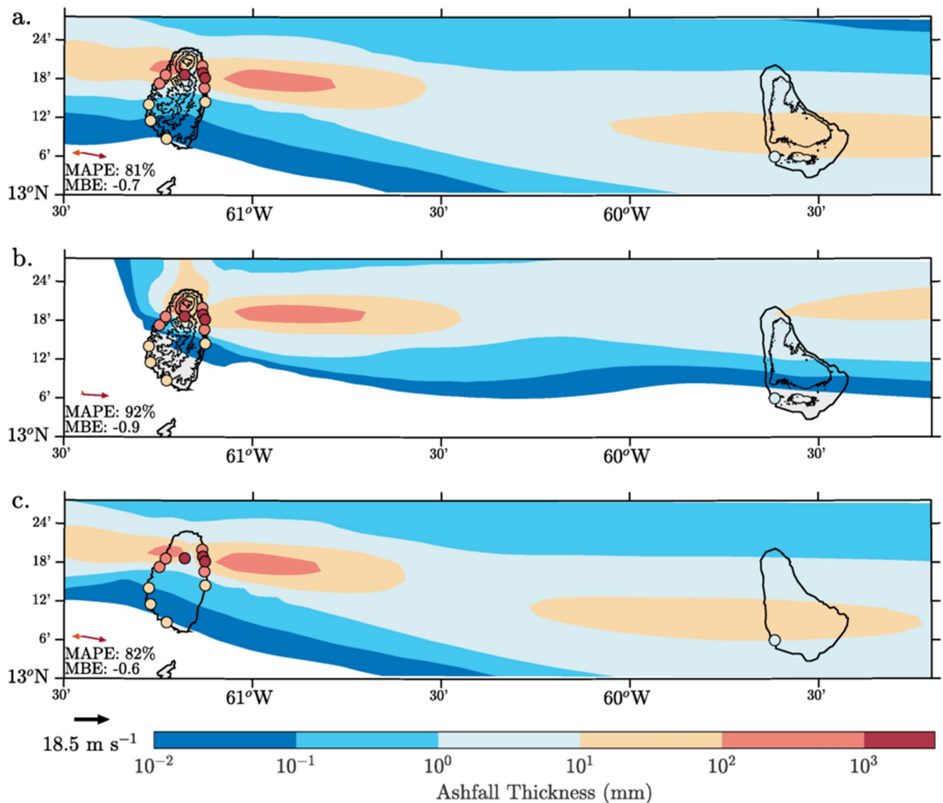
Figure 2. Ash thickness distributions following the 7 May 1902 eruption of Soufriere St Vincent. Simulated from the meteorological-ash-dispersion model where the experiments are (a) Control; (b) Alternative Wind profile; and (c) Flat Topography. Ash thickness observations are plotted over the contours using filled circle markers. Note the ash thickness scale is logarithmic. Topographic contours are shown at 100 m and every 300 m after that. Domain-averaged wind vectors at 100 m (orange) and averaged between 6–12 km (dark red) are shown in the bottom left corner. A deposit density of 1200 \text{ kg m}^{-3} was assumed to convert model ash fall to ash thickness. Topography contours are shown at 100 m and for every 300 m after that. Plotted using MATLAB Release 2016b, The MathWorks, Inc., Natick, Massachusetts, United States.
