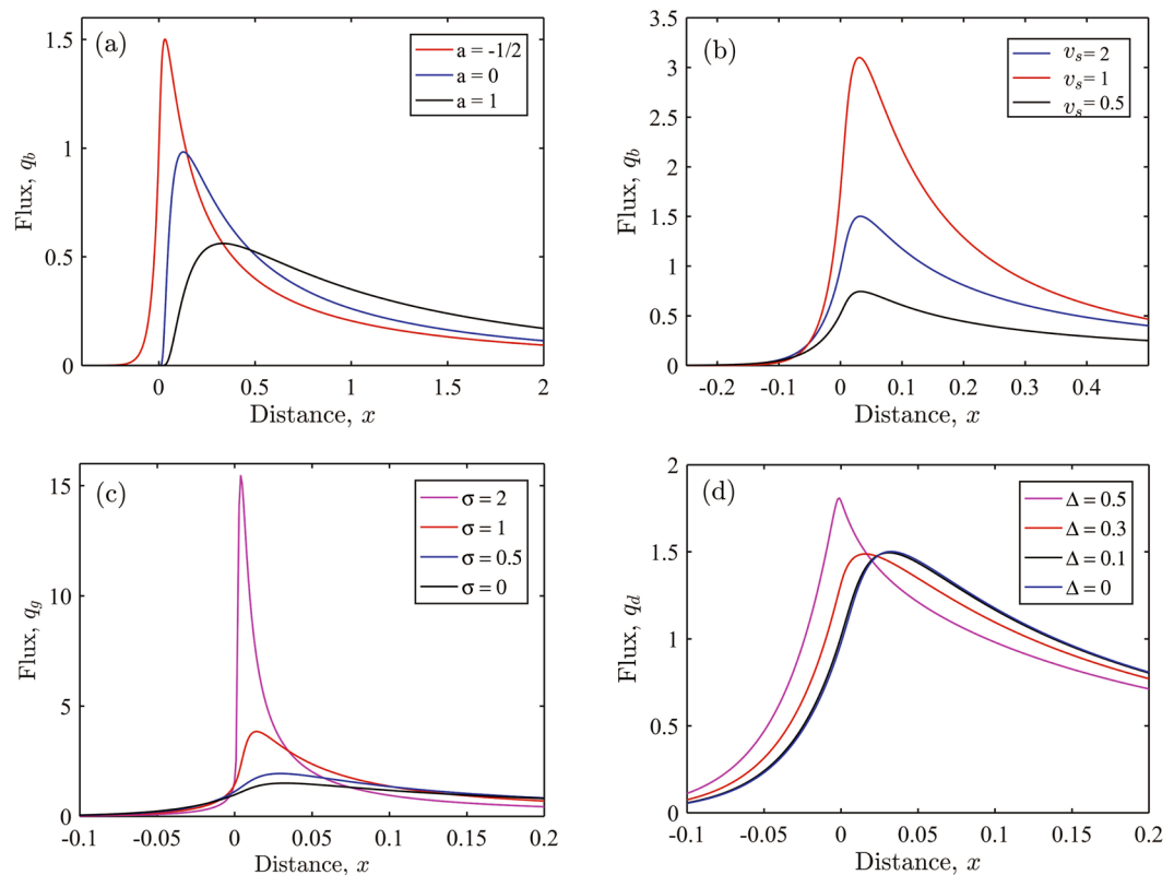
Figure 5. Ash deposition fluxes from an idealised advection-diffusion calculation. Results have been non-dimensionalised and show depositional flux at ground level q_b versus distance for different source and wind conditions. Depositional flux for various: (a) wind profiles of the form u(z)/U = a + (1-a)z/H , where U is wind speed at the source height H and a = -1/2 (a trade wind reversal profile); a = 0 (uniform shear); a = 1 (uniform flow); (b) settling velocities v_s ; (c) grain size distributions, where \sigma is the standard deviations in \varphi units (the mean \varphi is 5); and (d) source thicknesses \Delta = Z_s/H , where Z_s is the source layer depth. Default settings use the trade wind reversal profile a = -1/2 , a settling velocity v_s = V_s H/\kappa = 1 (where V_s is the particle settling velocity and \kappa is the turbulent diffusivity), a standard deviation of grain size \sigma = 2 , and a source thickness of Z_s/H = 0 .
