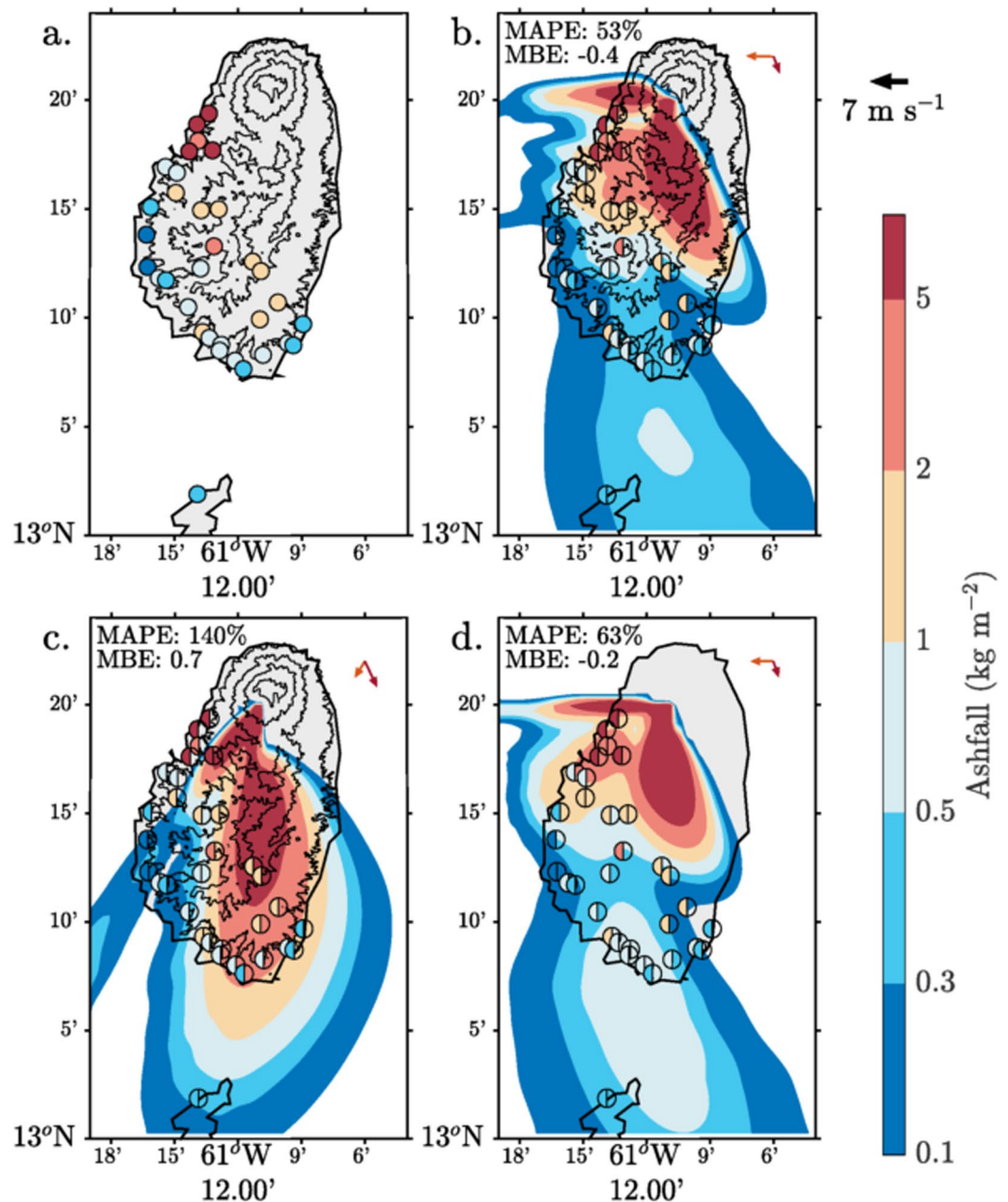
Figure 1. Ash fall distributions following the 26 April 1979 eruption of Soufriere St Vincent. (a) Observed, (b–d) simulated from the meteorological-ash-dispersion model, where the experiments are (b) Control; (c) Alternative Wind profile (lower shear); and (d) Flat Topography. Observations are plotted over the contours using filled circles markers. In Panels b–d observations correspond to the left half of the marker and modelled values to the right. Topographic contours are shown at 100 m and every 300 m after that. Domain-averaged wind vectors at 100 m (orange) and averaged between 6–12 km (dark red) are shown in the top right corner. Plotted using MATLAB Release 2016b, The MathWorks, Inc., Natick, Massachusetts, United States.
