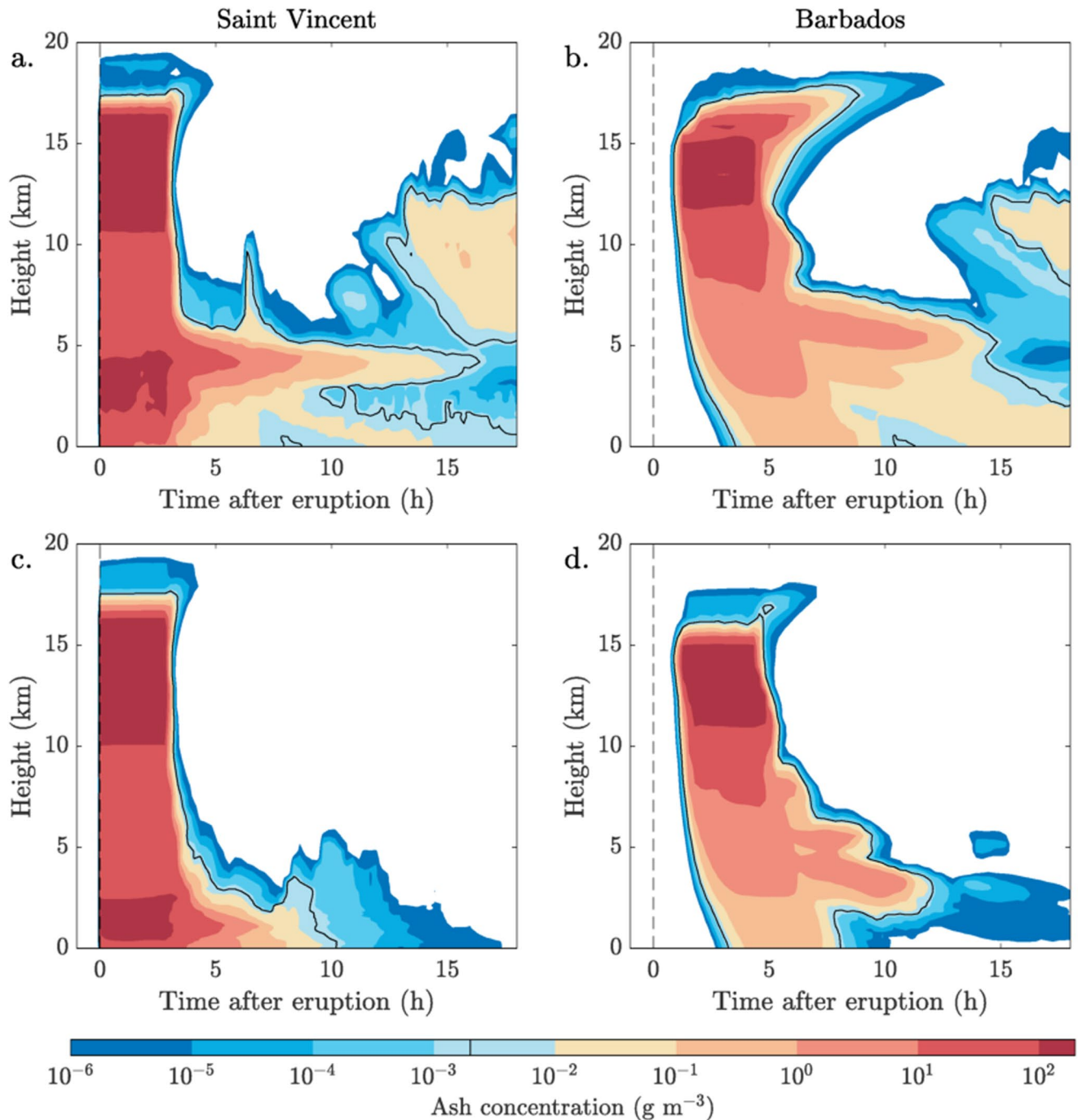
Figure 4. Maximum ash concentration above St Vincent and Barbados over time following the 7 May 1902 eruption. The ash concentration scale is logarithmic and the 2 \text{ mg m}^{-3} contour (the threat to aviation threshold) is marked in black. The top panels are from the Control simulation and the bottom panels are from the Alternative Wind profile simulation. A lingering hazardous ash cloud is present over St Vincent – and appears over Barbados – throughout the Control simulation, but is not simulated when the wind profile has little vertical wind shear. Plotted using MATLAB Release 2016b, The MathWorks, Inc., Natick, Massachusetts, United States.
