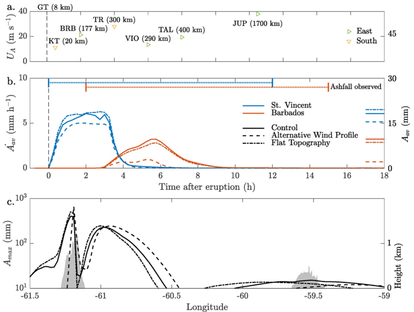
Figure 3. Ash observations and simulations for the 7 May 1902 eruption. (a) Estimated ash cloud velocity based on observations of ashfall east and south of the volcano; the numbers in brackets indicate the distance from the volcano. (b) Time series of ash thickness change (mm h -1 ) averaged over the two islands for the Control, Alternative Wind and Flat Topography experiments. The final averaged ash thickness (mm) is shown on the right-hand side of the plot. The periods of observed ashfall over the two islands is shown by the dotted lines at the panel top. (c) Cross-section of the maximum ash thickness against longitude. Local maxima over St Vincent, east (windward) of St Vincent, and over Barbados are evident. The maximum in topography of the islands is shaded in light grey.
