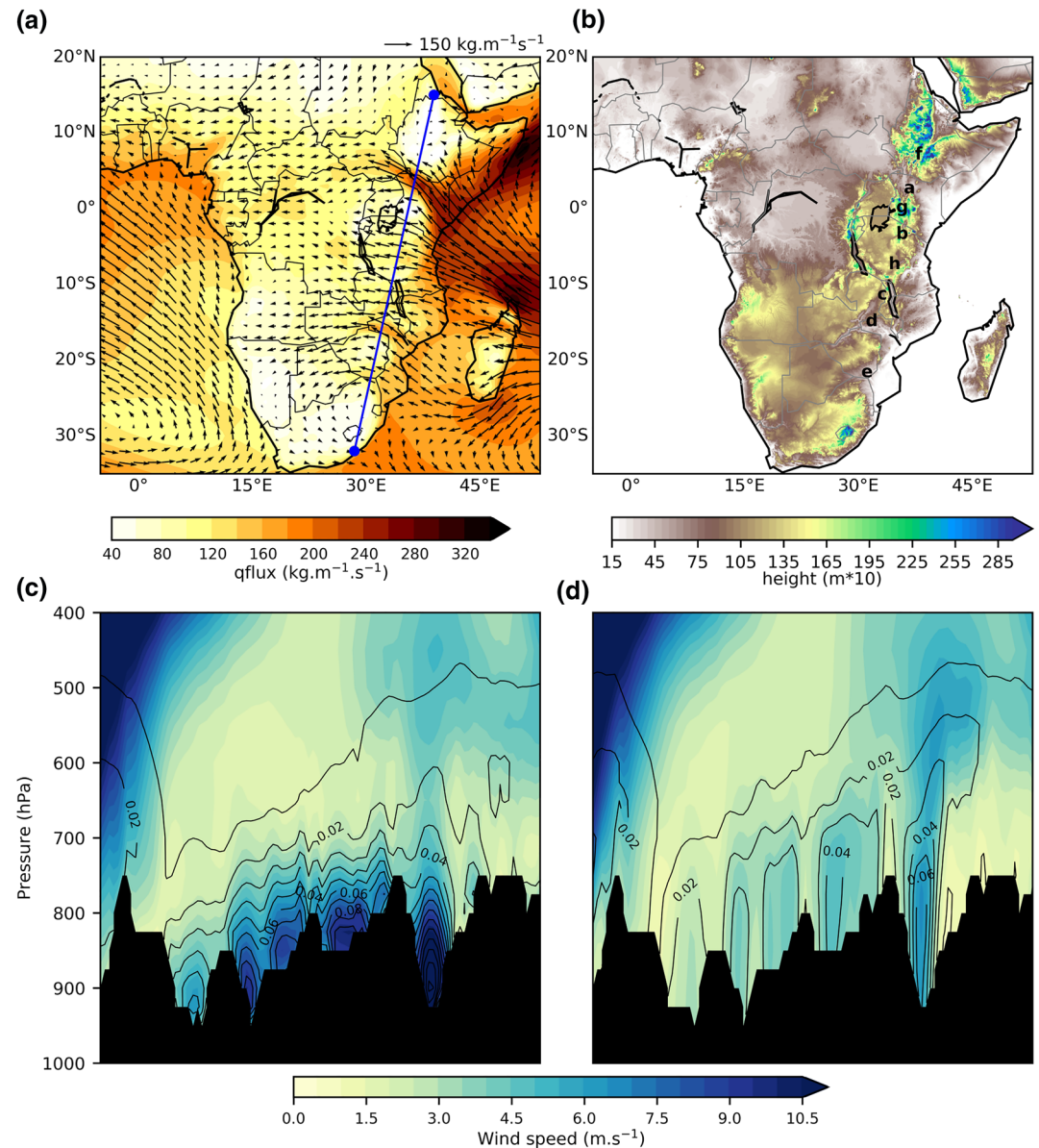
Figure 1. (a) Vertically integrated water vapor transport to 700 hPa (shaded; \text{kg m s}^{-1} ) with vectors of integrated water vapor transport. (b) African surface height (USGS—GTOPO30), units in \text{m}^*10 . Labels a–e are for LLJs: (a) Turkana; (b) Rufiji; (c) Malawi; (d) Zambezi; (e) Limpopo. Labels f, g, and h show orographic features: Ethiopian Highlands; Kenyan Highlands; and Tanzanian escarpment, respectively (c) 00:00 UTC and (d) 12:00 UTC vertical section through atmosphere of windspeed (shaded; \text{m s}^{-1} ) and water vapor flux (contours; \text{kg m s}^{-1} ) along blue line in (a) ( 15^\circ\text{N} ; 39^\circ\text{E} – 32^\circ\text{S} ; 28.5^\circ\text{E} ). LLJs, Low-Level Jets.
