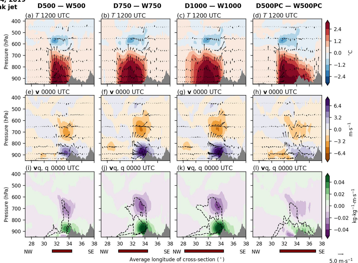
FIGURE 10 Vertical cross-sections of 10-day mean atmospheric differences between dry and wet simulations initialised on March 4, 2019. The panels show differences between (a, e, i) D500 and W500, (b, f, j) D750 and W750, (c, g, k) D1000 and W1000, and (d, h, l) D500PC and W500PC. Shown are differences in (a–d) air temperature (filled, ^{\circ}\text{C} ), (e–h) channel-orientated wind speed (filled, \text{m} \cdot \text{s}^{-1} ), and (i–l) channel-orientated moisture flux (filled, \text{kg} \cdot \text{kg}^{-1} \cdot \text{m} \cdot \text{s}^{-1} ). Arrows in (a)–(d) and (e)–(h) are horizontally and vertically scaled by differences in channel-orientated and vertical wind speed ( \text{m} \cdot \text{s}^{-1} ) respectively. To improve visualisation, arrows are only shown for every eighth grid point horizontally ( \approx 0.32^{\circ} ) and fifth grid point vertically. Additionally, vertical wind speeds are multiplied by 100.0. Dashed contours in (i)–(l) show differences in specific humidity at intervals of -0.5 \text{ g} \cdot \text{kg}^{-1} . Grey shading indicates the orographic cross-section, which is based on the minimum 20th percentile of simulated surface pressure between the two simulations across the cross-section throughout the 10-day simulation. The red rectangles below bottom-row panels denote locations where at least one grid point has fully prescribed soil moisture for each simulation set. [Colour figure can be viewed at wileyonlinelibrary.com ]
