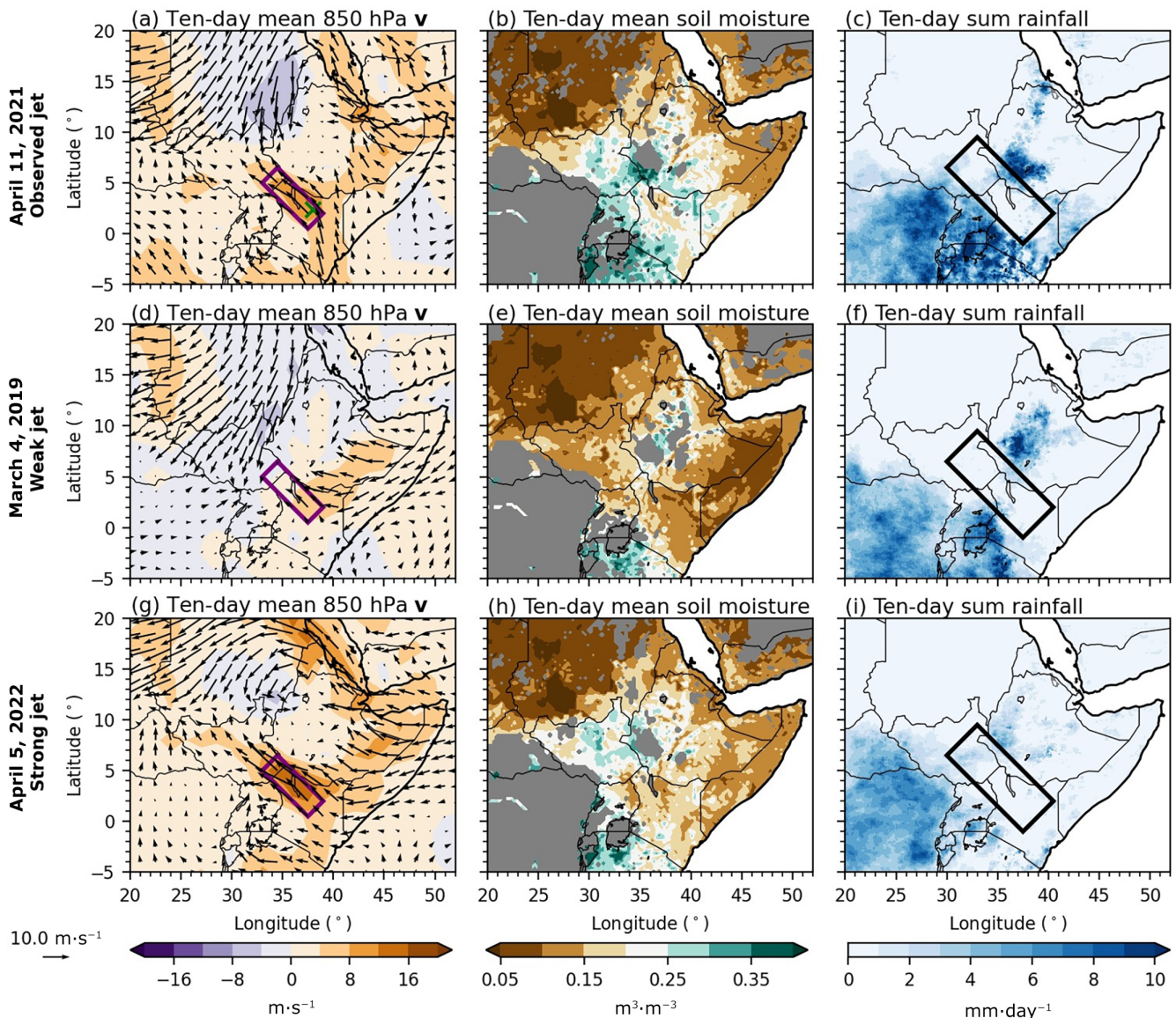
FIGURE 1 The 10-day mean of (a, d, g) the channel-orientated (filled) and horizontal (arrows) wind ( \text{m} \cdot \text{s}^{-1} ) at 850 hPa, (b, e, h) the European Space Agency Climate Change Initiative surface soil moisture ( \text{m}^3 \cdot \text{m}^{-3} ); (c, f, i) the 10-day rainfall accumulation ( \text{mm} \cdot \text{day}^{-1} ) during each of the chosen case studies. (a)–(i) Environmental conditions for 10-day case studies commencing on (a–c) April 11, 2021, (d–f) March 3, 2019, and (g–i) April 5, 2022. To improve visualisation, horizontal wind components are only shown for every fourth grid point ( \approx 1.0^\circ ). The purple transect in panels (a), (d), and (g) denotes the area used to identify periods with strong and weak jet conditions, and the black transect in panels (c), (f), and (i) denotes the area used to quantify rainfall in the periphery of the Turkana jet (Supporting Information Figure S1). The green cross in (a) denotes the town of Marsabit, where radiosondes were launched from during the Radiosonde Investigation for the Turkana Jet campaign. [Colour figure can be viewed at wileyonlinelibrary.com ]
