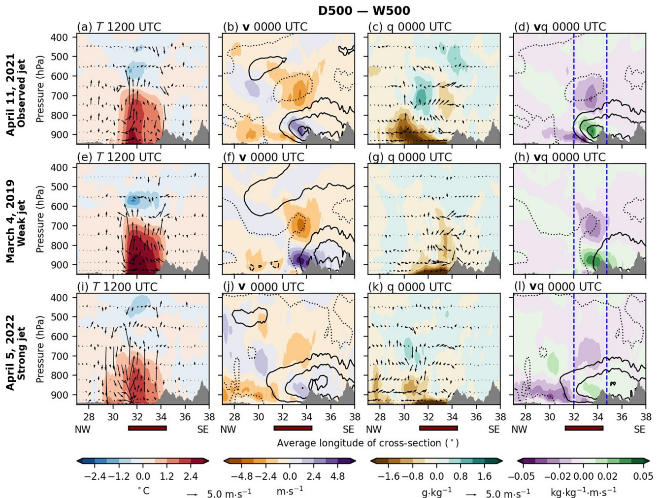
FIGURE 6 Vertical cross-sections of 10-day mean atmospheric differences between D500 and W500 simulations with prescribed soil moisture within 500 km of the Turkana channel's exit: (a, e, i) air temperature (filled, ^{\circ}\text{C} ), (b, f, j) channel-orientated wind speed (filled, \text{m}\cdot\text{s}^{-1} ), (c, g, k) specific humidity (filled, \text{g}\cdot\text{kg}^{-1} ), and (d, h, l) channel-orientated moisture flux (filled, \text{kg}\cdot\text{kg}^{-1}\cdot\text{m}\cdot\text{s}^{-1} ). Arrows in the first and third columns are horizontally and (c, g, k) vertically scaled by differences in channel-orientated and vertical wind speed ( \text{m}\cdot\text{s}^{-1} ) respectively. To improve visualisation, arrows are only shown for every eighth grid point horizontally ( \approx 0.32^{\circ} ) and fifth grid point vertically. Additionally, vertical wind speeds are multiplied by 100.0. The lined contours in the second and fourth columns show absolute values from control simulations in intervals of 5\text{ m}\cdot\text{s}^{-1} and 0.5\text{ kg}\cdot\text{kg}^{-1}\cdot\text{m}\cdot\text{s}^{-1} respectively. Solid lines denote positive values, whereas dotted lines indicate the zeroth contour. Grey shading indicates the orographic cross-section, which is based on the minimum 20th percentile of simulated surface pressure between D500 and W500 across the cross-section throughout the 10-day simulation. The red rectangles below all bottom-row panels denote locations where at least one grid point has fully prescribed soil moisture. Blue dashed lines in panels (d), (h), and (l) highlight the area used to compute moisture flux profiles (Figure 7). [Colour figure can be viewed at wileyonlinelibrary.com ]
