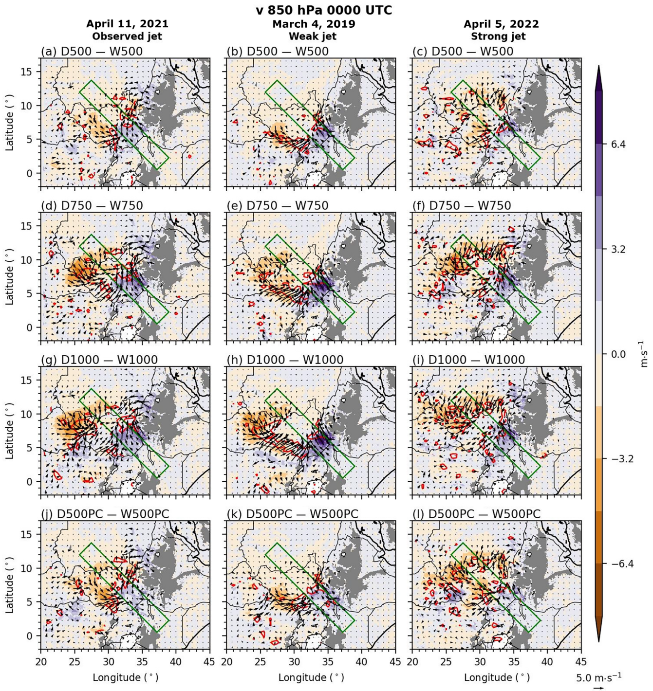
FIGURE 9 Differences in 10-day mean channel-orientated wind speed (filled, \text{m} \cdot \text{s}^{-1} ) between dry and wet simulations. The panels show differences between (a–c) D500 and W500, (d–f) D750 and W750, (g–i) D1000 and W1000, and (j–l) D500PC and W500PC. Arrows, which are only shown for every 20th grid point ( \approx 0.8^\circ ) to improve visualisation, denote horizontal wind components. Red lined contours denote areas of wind convergence greater than 2.5 \times 10^{-5} \text{ s}^{-1} after downscaling to a 0.5^\circ resolution. Left, center and right panels show simulated atmospheric differences for case studies initialised on 11th April 2021, 4th March 2019 and 5th April 2022 respectively. On all panels grey shading indicates grid points where the minimum surface pressure between the two simulations is smaller than 850 hPa at any time in the 10-day simulation. Green rectangles in all panels highlight the area used for vertical cross-sections through the Turkana channel (Figure 10 and Supporting Information Figures S9 and S10). [Colour figure can be viewed at wileyonlinelibrary.com ]
