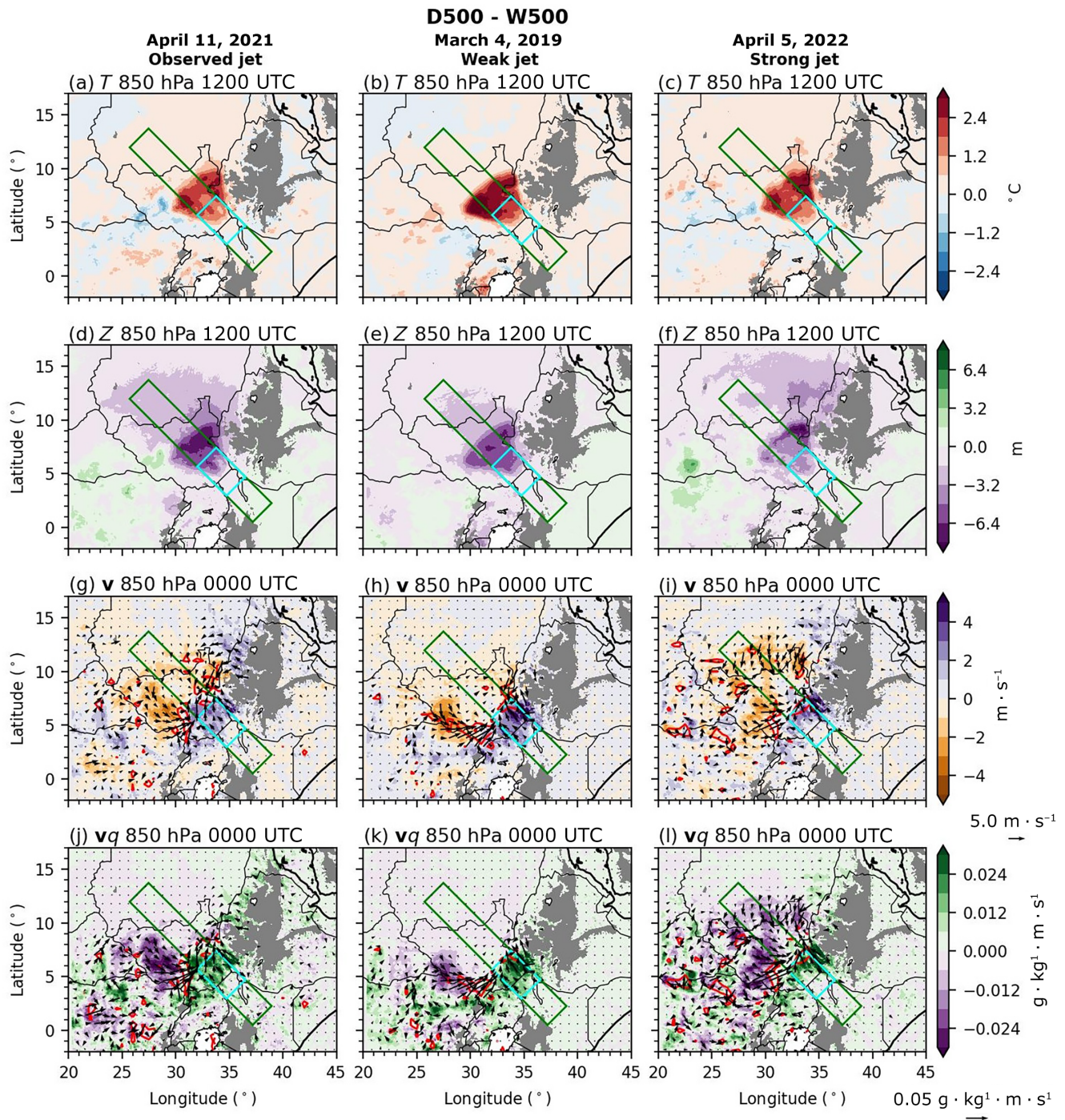
FIGURE 5 The 10-day mean atmospheric differences between D500 and W500 simulations with prescribed soil moisture within 500 km of the Turkana channel's exit: (a–c) air temperature (filled, °C) and (d–f) geopotential height (filled, m) at 1200 UTC/1500 h EAT; (g–i) channel-orientated wind speed (filled, \text{m} \cdot \text{s}^{-1} ) and (j–l) channel-orientated moisture flux (filled, \text{kg} \cdot \text{kg}^{-1} \cdot \text{m} \cdot \text{s}^{-1} ) at 0000 UTC/0300 h EAT. All atmospheric differences are shown at 850 hPa. Arrows in (g)–(i) denote horizontal wind components, whereas in (j)–(l) they denote horizontal moisture flux components. To improve visualisation, arrows are only shown for every 20th grid point ( \approx 0.8^\circ ). Red lined contours in (g)–(i) and (j)–(l) mark areas of wind and moisture convergence greater than 2.5 \times 10^{-5} \text{ s}^{-1} and 2.5 \times 10^{-7} \text{ kg} \cdot \text{kg}^{-1} \cdot \text{s}^{-1} respectively, after downscaling to a 0.5^\circ resolution. Simulated atmospheric differences are shown for case studies initialised on (a, d, g, j) April 11, 2021, (b, e, h, k) March 4, 2019, and (c, f, i, l) April 5, 2022. On all panels, grey shading indicates grid points where the minimum surface pressure between D500 and W500 is smaller than 850 hPa at any time in the 10-day simulations. Green and cyan rectangles in all panels highlight the areas used for vertical cross-sections through the Turkana channel (Figure 6) and computing vertical profiles of the channel-orientated moisture flux (Figure 7) respectively. [Colour figure can be viewed at wileyonlinelibrary.com ]
