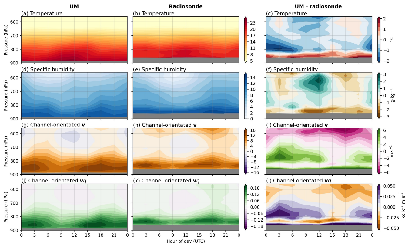
FIGURE 4 The 10-day mean diurnal cycles of atmospheric profiles in (a–c) temperature ( ^{\circ}\text{C} ), (d–f) specific humidity ( \text{g} \cdot \text{kg}^{-1} ), (g–i) channel-orientated wind speed ( \text{m} \cdot \text{s}^{-1} ), and (j–l) channel-orientated moisture flux ( \text{kg} \cdot \text{kg}^{-1} \cdot \text{m} \cdot \text{s}^{-1} ). (a, d, g, j) Mean absolute values from the control simulation initialised on April 11, 2021; (b, e, h, k) mean radiosonde observations taken during the same 10-day period. (c, f, i, l) Differences between control simulations and radiosonde observations. In all panels, grey shading represents pressures greater than the 10-day minimum surface pressure, calculated at 3-hr intervals. For panels comparing simulations with observations, the minimum surface pressure between radiosonde data and UK Met Office Unified Model simulation output is used. [Colour figure can be viewed at wileyonlinelibrary.com ]
