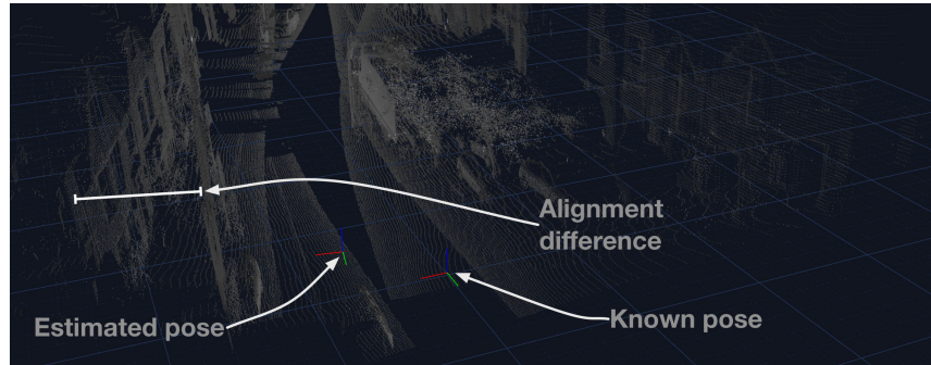
Figure 4.27: Hard registration task. A difficult registration task. In this case, we have an induced error of over 3m in both X and Y directions, and 10^\circ of orientation error.
