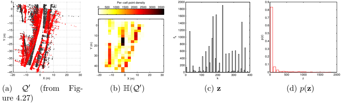
Figure 4.46: Mutual Information process: Swathe. Steps illustrating the MI estimation process for the swathe, \mathcal{Q}' . (a) Projected swathe, \mathcal{Q}' in red, and the prior \mathcal{P} in black (b) Histogram approximation \mathbb{H}(\mathcal{Q}') , (c) Pseudo-measurements \mathbf{z} , and (d) Density estimation, p(\mathbf{z})
