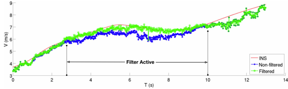
Figure 6.37: Filtered velocity estimates. The corresponding filtered velocity estimates (shown in green) against the unfiltered estimates (blue) over the scene shown in Figure 6.34, as compared to the INS estimate (red).
