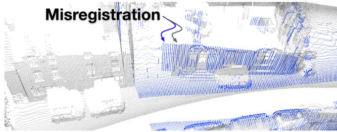
Figure 5.21: GICP: Matching failure. A location in Woodstock that causes GICP to fail to find a good match. The runtime data was generated using velocities inferred from LO. Point-to-point matching algorithms (and their variants) perform worse when the velocity estimates exhibit any degree of compression/expansion. A comparison of the trajectories obtained using GICP is shown in Chapter 5.
