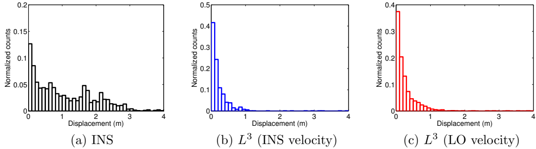
Figure 5.28: Relative displacement: L^3 (24/07/2012). Histograms of the relative displacement for L^3 over the trajectories shown in Figure 5.27(a), showing (a) the INS performance, (b) L^3 with INS velocity, and (c) L^3 with LO velocity.
