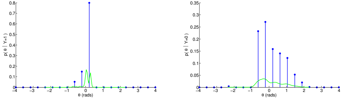
Figure 6.22: Non-stationary Model conditionals: angle. The conditional distributions over angle for the same model shown in Figure 6.21. The form is very similar to the conditional distribution over angle from the stationary model (Figure 6.20), which implies that while traffic appears uniformly over distance, the same is not true for bearing. (Blue corresponds to the PMF from histogrammed counts, green to the kernel-density estimated PDF).
