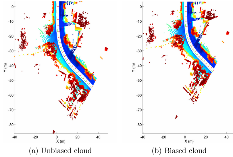
Figure 6.11: Comparison of biased vs. unbiased point clouds. (a) Shows an overhead view of the point cloud from the downward-facing LIDAR (coloured by height above the ground, blue being lowest and red highest) using the INS velocity feed. (b) Shows the same LIDAR-data, but generated using the biased velocity estimate (shown in Figure 6.10). This “compression” leads to point clouds that are a poor representation of reality, resulting in localisation error. In both cases, a centre-swathe of points has been omitted in order to render the poses.
