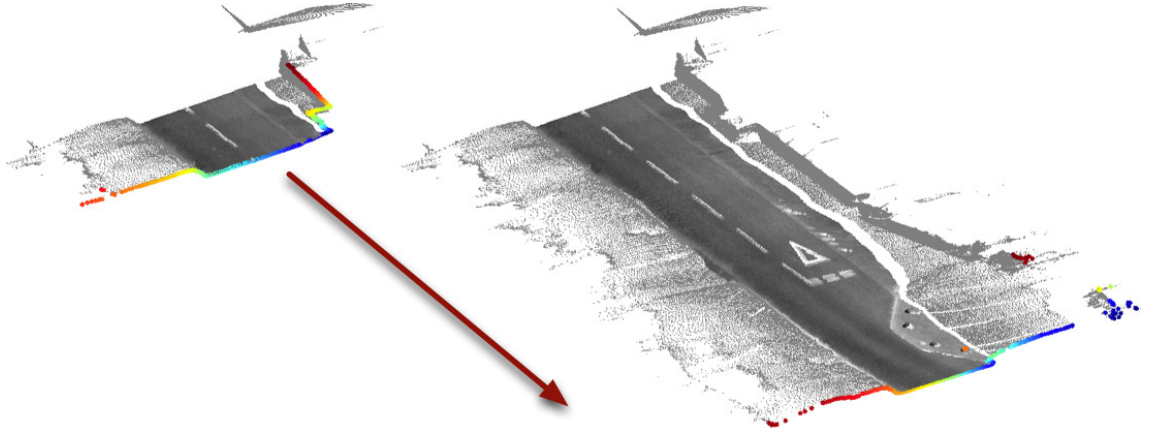
Figure 4.11: Example 3D data from a 2D pushbroom LIDAR. The process of generating 3D point clouds from the egomotion of the declined LIDAR through the scene, highlighted by the arrow. If we observe the rotational and linear velocities of the sensor, we can integrate these to produce this 3D cloud. Particularly visible are the retro-reflective road-markings and lane demarcations. The speed of the vehicle was approximately 6m/s, with the LIDAR scanning at 50 Hz.
