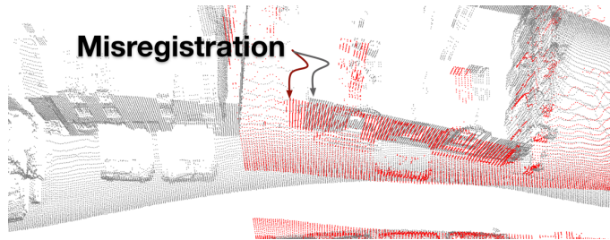
Figure 5.23: NDT: Matching failure. A matching failure for a similar point cloud, in the same location as in Figure 5.21.
