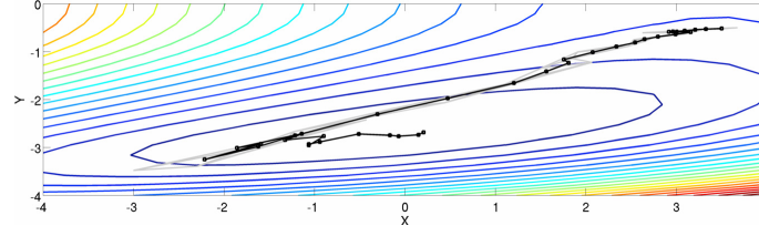
Figure 4.51: Optimisation illustration: Simplex algorithm. The Nelder-Mead simplex method over an example objective function (Himmelblau’s function). Simplex evaluations – and their associated centroid – are shown in grey and black, respectively.
