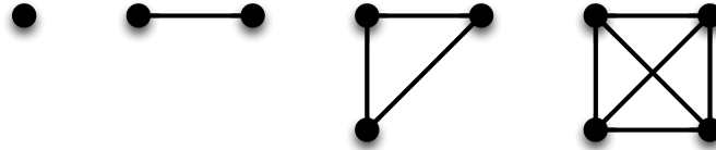
Figure 6.53: Fully connected sub-graphs, or “cliques” . Fully connected cliques for 1, 2, 3, and 4 variables. The pairwise cliques in the MRF model correspond to a fully-connected graph of size 2.
