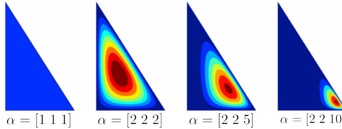
Figure 4.24: Dirichlet “shape” parameters. An illustration of the growth of a trivariate Dirichlet distribution with increasing variable counts. On the left, the \alpha parameters are equal and unary – each variable has equal probability. As we observe more “counts” of one variable, the posterior mass begins to shift – with a corresponding shrink in variance – to that variable (Red corresponds to high probability, blue to low probability).
