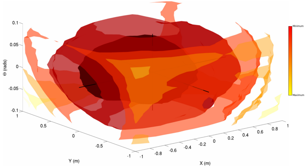
Figure 4.33: Relative Entropy objective “volume” . Representative iso-surfaces of the relative entropy, exhaustively evaluated over the input domain using the same data as shown in Figure 4.28.
