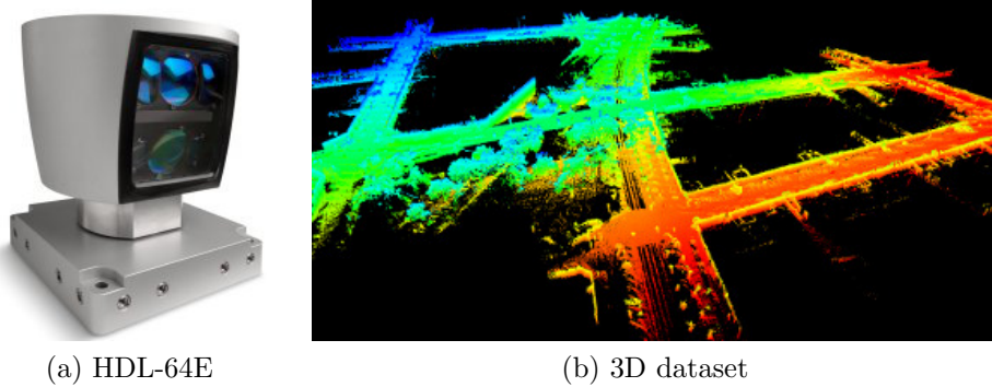
Figure 2.4: Velodyne HDL-64E 3D LIDAR . The Velodyne was a core component for mapping and localisation for many teams in the Urban challenge. (a) shows the sensor, and (b) a map acquired by [68].
