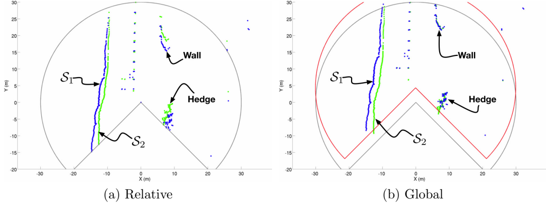
Figure 6.15: Consecutive LIDAR sweeps en-route to Woodstock. An overhead view of two scans from the horizontal LIDAR en-route to Woodstock. Points from one-second separated scans (green and blue, respectively) are overlaid into a global frame using the INS estimates. Visible are a wall and a roadside hedge. (b) The same fans, rendered into a global frame using the INS. The wall and hedge are now well aligned – however, the points on the left are not aligned, indicative of ground-strike.
