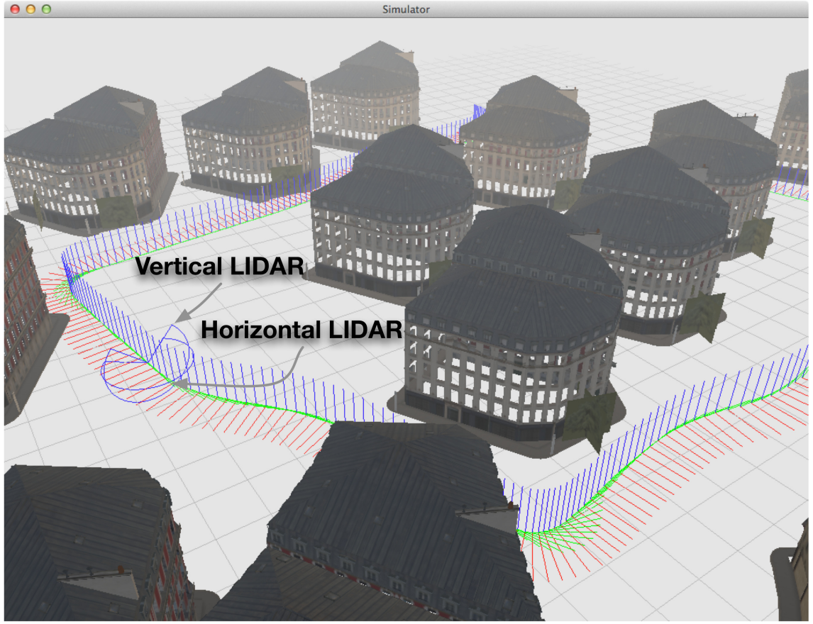
Figure 5.1: Synthetic validation. A virtual robot operating in a synthesized scene. The robot is augmented with two declined LIDARs, mimicking our actual sensor payload.
