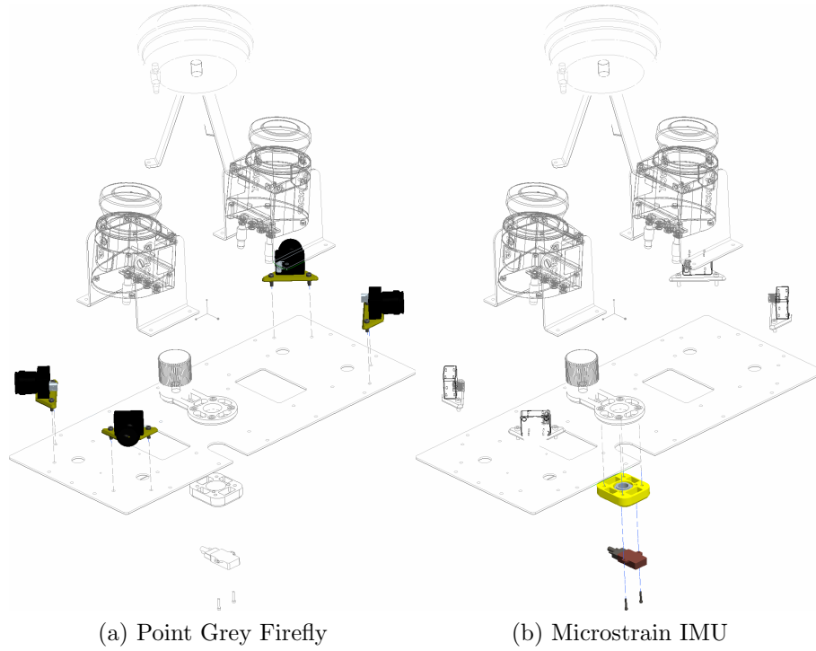
Figure 3.24: NABU sensors: Firefly cameras, and IMU. The remaining sensor packages on the top sub-assembly are the (a) four Point Grey Firefly monocular cameras, and (b) a MicroStrain Inertial Measurement Unit (IMU).
