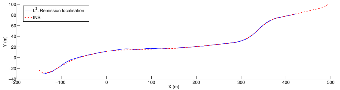
Figure 5.39: Featureless road section: Localisation results. Localisation results over the section shown in Figure 5.38 by matching remission using Mutual Information. The ground-truth (INS) estimates are shown in dashed red, the L3-MI estimates in solid blue.
