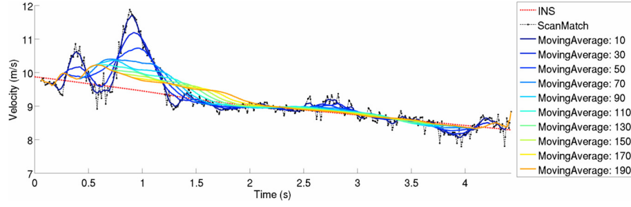
Figure 4.18: Velocity Filtering: Moving-average. Velocity filtering using a moving-average filter of varying window sizes over scan-match velocity estimates.
