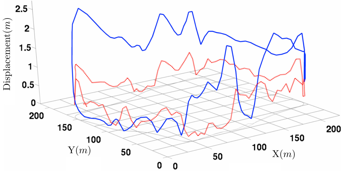
Figure 5.10: Relative displacement: L^3 vs. INS over 700m. An example relative displacement graph of both L^3 (shown in red, dotted) and the INS (blue, solid) as measured against a map of the Begbroke site. The INS exhibits a high displacement in areas of poor GPS signal quality, whereas L^3 is relatively constant.
