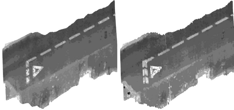
Figure 3.30: Timing illustration. Overhead view of a set of road markings around the Begbroke site. The point cloud generated with TICSynC-corrected timings is shown on the left, as compared against a similar point cloud with normally-distributed 50ms error. The corrected point cloud does not exhibit the ghosting (visible in the right image).
