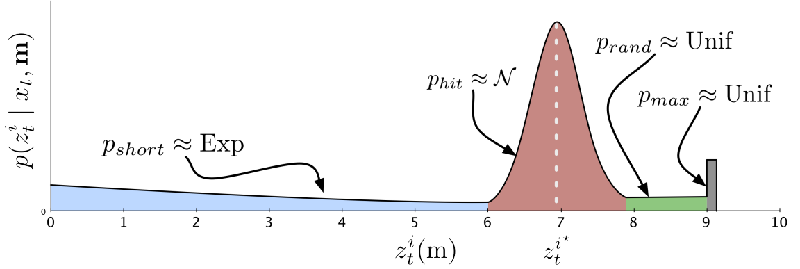
Figure 2.9: LIDAR beam model. A beam-model used in the measurement likelihood, inspired by a similar figure in [93]. The beam-model is comprised of a p_{short} component, modelled by an exponential distribution, a p_{hit} component (Gaussian), a “random” component (Uniform) and a max-range component (Uniform).
