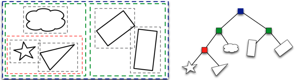
Figure 3.8: Example AABB tree. Shown are example primitives (left) along with their associated bounding boxes (grey, dashed), and the resulting AABB tree (right). The node colours in the tree correspond to the bounding-box colours in the spatial layout.
