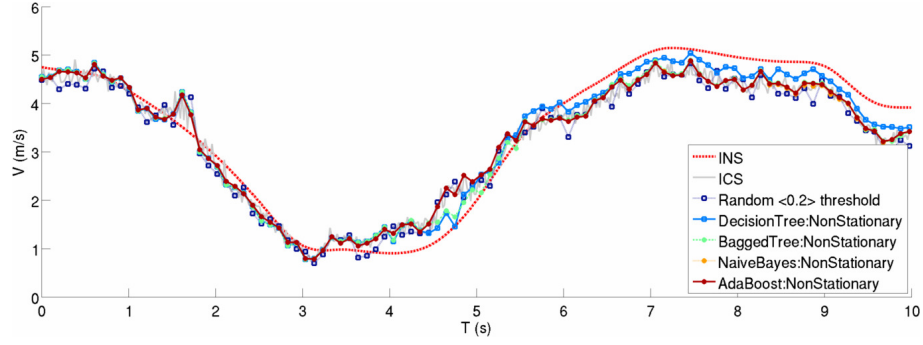
Figure 6.39: Filtered velocity estimates (Woodstock centre) . Filtered velocity estimates using the various classification techniques over the Woodstock town centre. Again apparent is the improved velocity estimate from the contextually-filtered estimator. RMSE comparisons are shown in Table 6.5.
