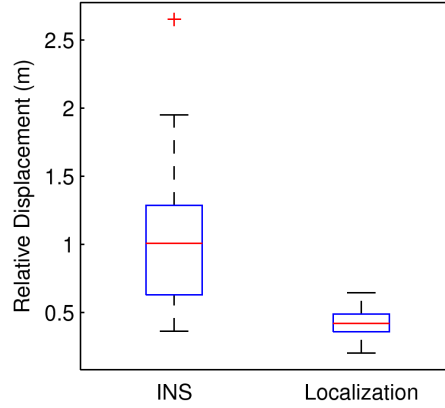
Figure 5.11: Cumulative relative displacement comparisons. A comparison of the mean displacement from the experience map for both the INS (left) and localisation using L^3 (right) over 26 km worth of trajectory data spanning three months. The box plot shows the median, 25 th and 75 th percentiles, with outliers plotted individually as points. As can be seen from the figure, the standard deviation of this displacement is substantially lower for L^3 .
