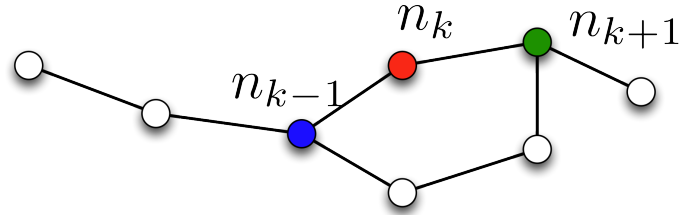
Figure 5.16: Graph-based map-management. Due to the sizes of the map for large-scale localisation tasks, map retrieval is done by traversing a graph of anchor nodes embedded in the map trajectory. This allows for sequential access, and alleviates the need to load the entire map into memory. Shown here is the current node n_k , and the next and previous nodes, n_{k+1} and n_{k-1} respectively.
