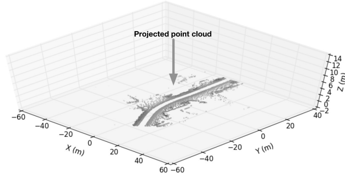
Figure 4.21: Projected point cloud. The projected point cloud, corresponding to Figure 4.20. This projected cloud is obtained from the raw point cloud by removing the height ( Z ) component.
