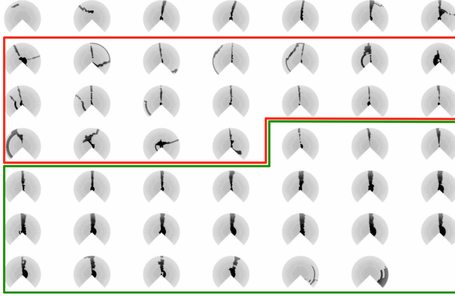
Figure 6.29: Learned models. The decision boundaries for the bagged decision-tree models for the locations depicted in Figure 6.17. Noticeable is the contrast between models learned in areas with a large dynamic component (highlighted in red are the models trained in the town centre, showing the variegated decision boundary shapes), and models learned where the traffic flow is more consistent (the green-highlighted models show models on the main road).
