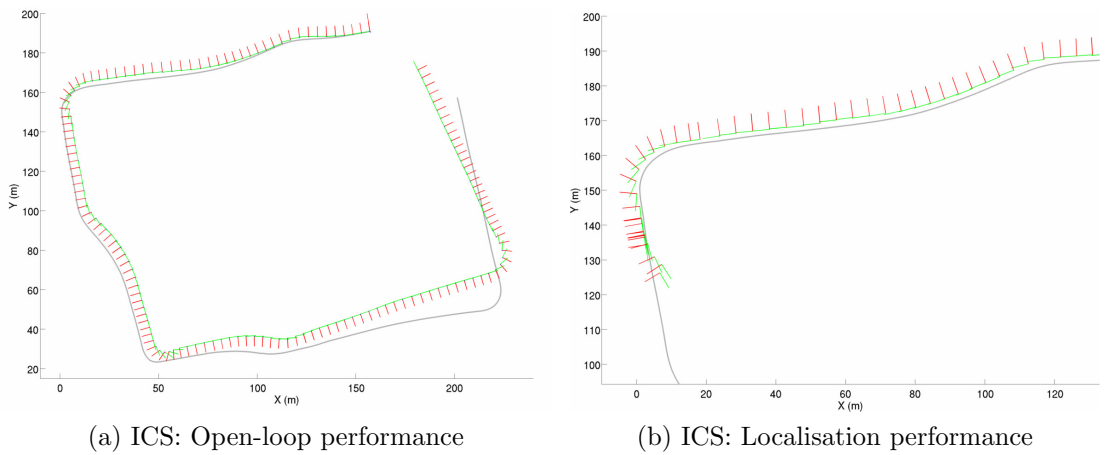
Figure 4.4: Scan-matching comparison: Open-loop vs. Localisation, 63 days later. Open-loop (a) and localisation (b) performance for an ICS scan-matcher, using a map from 63 days prior. Notice the localisation failure at (x = 10, y = 130) – this is due to distinct scene change in the intervening months.
