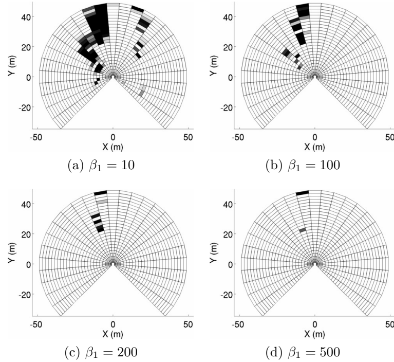
Figure 6.54: Cell transiency probabilities for varying \beta . (a) \beta_1 = 10 , (b) \beta_1 = 100 , (c) \beta_1 = 200 , (d) \beta_1 = 500 . Darker cells indicate higher probability.
