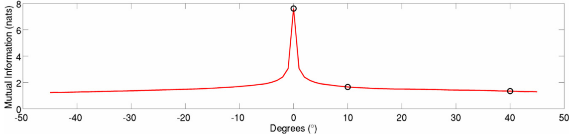
Figure 4.44: Mutual Information: Registration example. The MI for varying degrees of rotation ( \alpha ). Note the sharp peak at 0^\circ , which is to be expected – these images are maximally informative about each other at this angle. As the rotation is increased, the probability mass of the joint distribution becomes more diffuse, meaning the two distributions are progressively less informative. Highlighted are the rotation values for the images shown in Figure 4.42.
