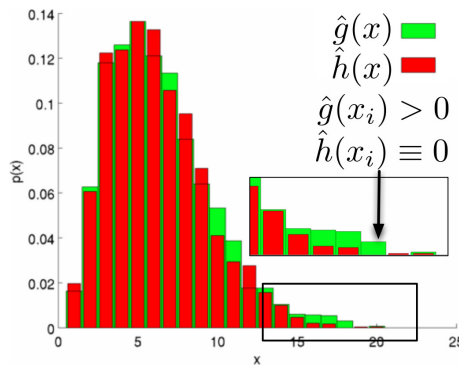
Figure 4.32: Estimating the KL-divergence from histograms. An issue arising from estimating the KL-divergence for probability distributions obtained from counts.
