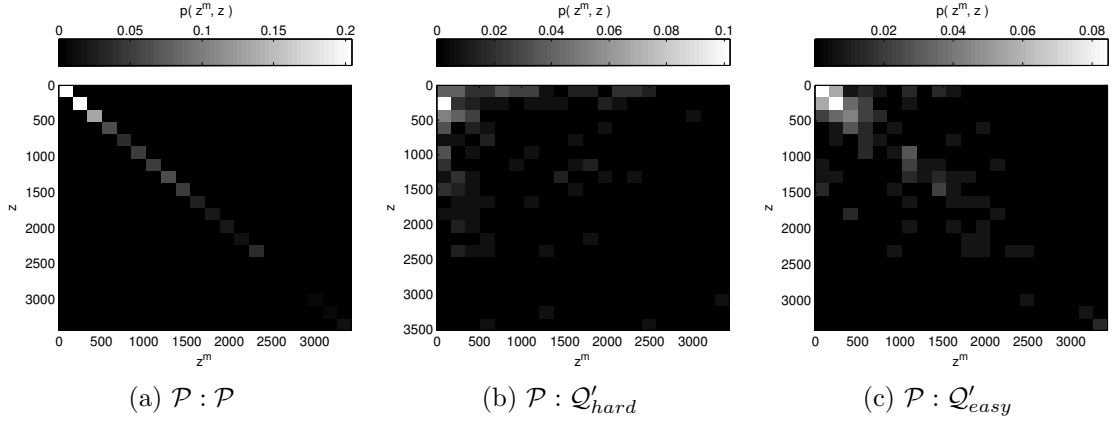
Figure 4.47: Joint distribution comparison.
