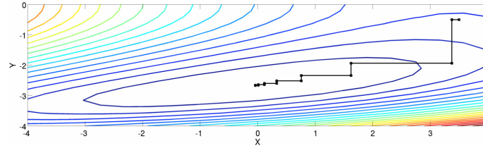
Figure 4.52: Optimisation illustration: Co-ordinate descent. Optimisation (function minimisation) using repeated application of coordinate descent, with minima found using Brent’s method.
