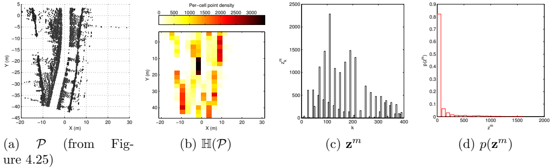
Figure 4.45: Mutual Information process: Prior. Steps illustrating the MI estimation process for the prior, \mathcal{P} . (a) Original point cloud, (b) Histogram approximation \mathbb{H}(\mathcal{P}) , (c) Pseudo-measurements \mathbf{z}^m , and (d) Density estimation, p(\mathbf{z}^m)
