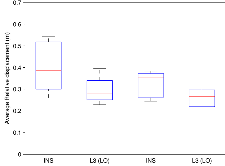
Figure 6.47: Woodstock/Kidlington INS/ L^3 displacement comparison. Averaged relative displacement for the data collected over Woodstock (INS and L^3 , left), and Kidlington (INS and L^3 ). Note that the left two images correspond to the Woodstock comparison, and the right two to the Kidlington comparison. The lower average relative displacement of L^3 is visible in both of these locations.
