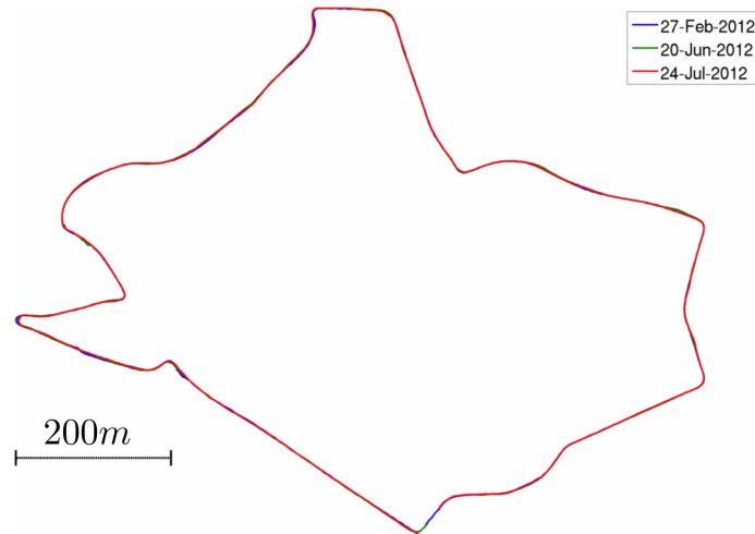
Figure 6.45: The resulting trajectories using contextual scan-filtering. After applying the contextual scan-filtering technique (in this case, bagged decision trees), the points of failure have been eliminated and the system stays localised for each of the datasets.
