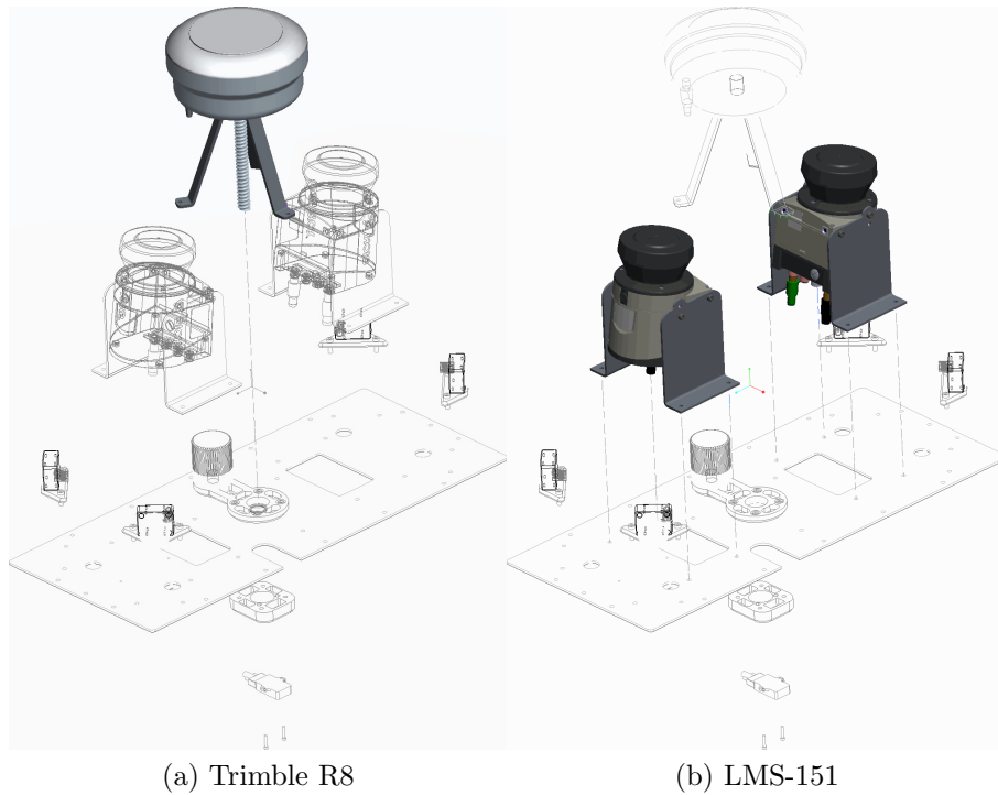
Figure 3.23: NABU sensors: GPS and LIDAR. Two of the sensor modalities of the NABU: (a) a Trimble R8 GPS, and (b) dual SICK LMS-151 scanning LIDARs.
