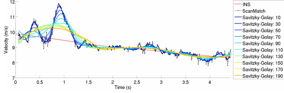
Figure 4.17: Velocity Filtering: Savitzky-Golay. Velocity filtering using the Savitzky-Golay algorithm for varying window sizes over scan-match velocity estimates.
