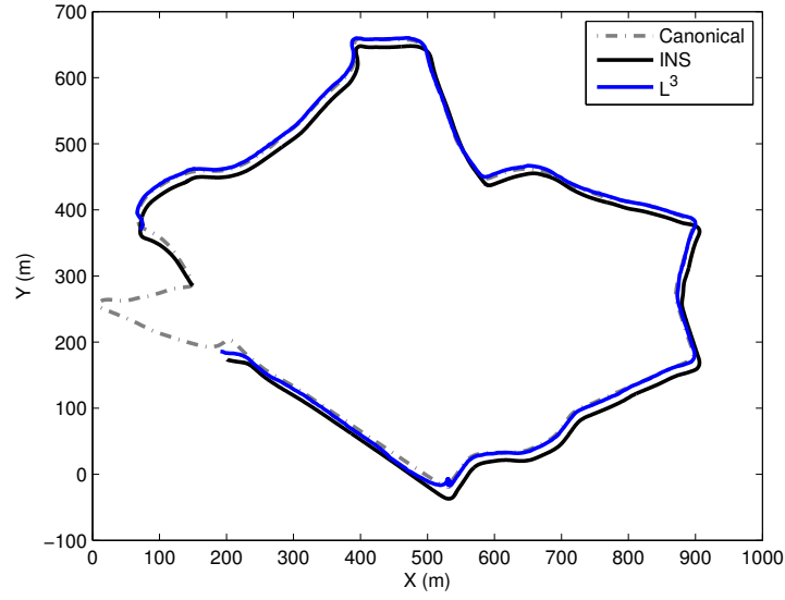
Figure 5.35: Trajectory comparison around Woodstock: INS vs L^3 . Comparisons of estimated trajectories around the canonical Woodstock route (grey, dashed) using L^3 (blue) and the INS (black). Note the Y axis shift present in the INS estimate.
