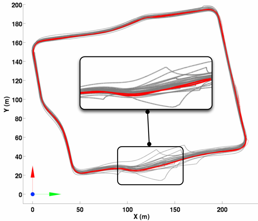
Figure 5.7: L^3 vs. INS over 26km (and 3 months). A comparison of the INS trajectories (grey, dotted) vs. the L^3 trajectories (red, solid). As is very apparent from the image, the INS data drifts substantially in areas of poor reception (predominantly the northern and southern sections), while L^3 does not exhibit the same degenerate performance.
