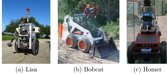
Figure 4.9: Generating 3D point clouds from 2D LIDARs. (a) The Lisa platform, based on a Segway RMP. (b) A Bobcat vehicle, with a rotating 2D LIDAR, as developed by [15] (c) The Homer research platform with a “nodding” LIDAR.
