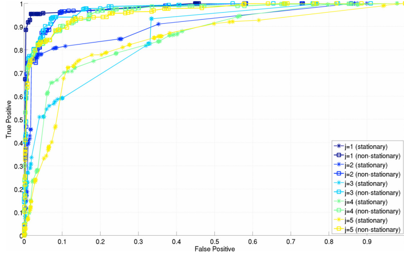
Figure 6.28: Boosted Decision Trees stationary vs. non-stationary ROC. Boosted decision trees (using the AdaBoostM1 algorithm) ROC curves, for the same training instances shown in Figure 6.26 and Figure 6.27. The boosted trees again outperform NaiveBayes, and are comparable to the bagged approach, but again show that the non-stationary model is superior to the stationary model.
