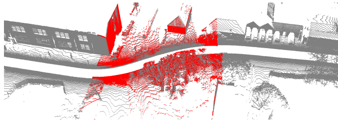
Figure 5.22: NDT: Good match. A successful match from a run-time point cloud (coloured red) against a previously captured survey (grey).
