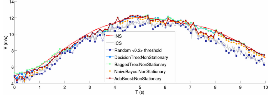
Figure 6.38: Filtered velocity estimates (Woodstock entry) . A comparison of each of the classification strategies (NaiveBayes, Boosting and Bagging) for the scene shown in Figure 6.30(a). The ICS velocity estimates, due to traffic, underestimate the true velocity. However, filtering out points that are likely to be traffic leads to better velocity estimates for each of the classification schemes.
