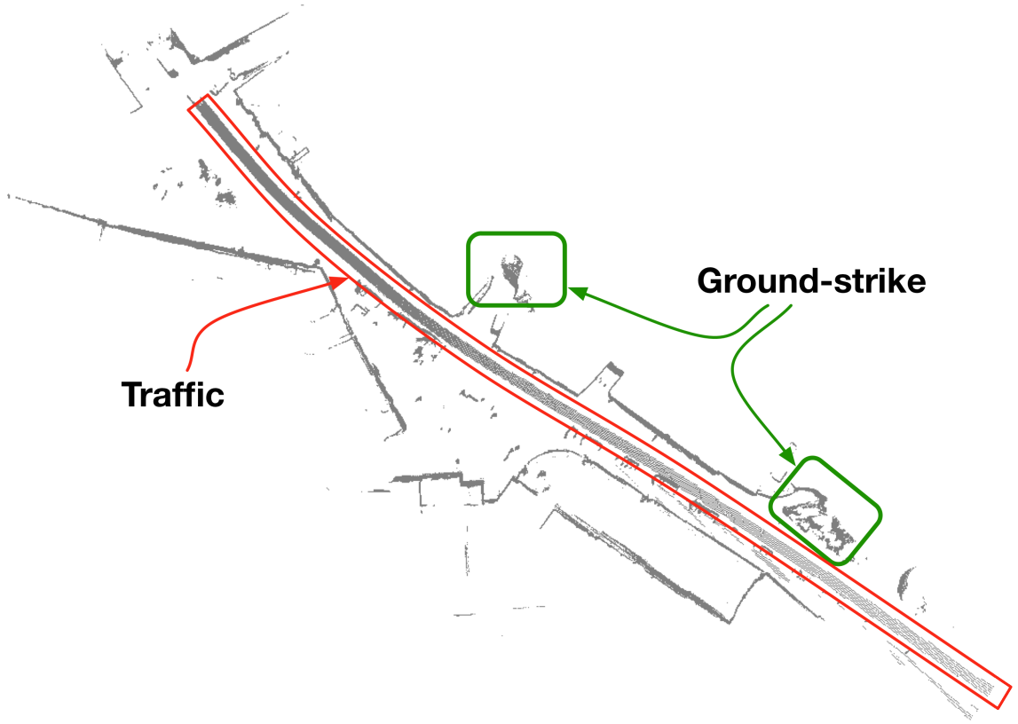
Figure 6.50: Woodstock LIDAR transiency illustration: Raw LIDAR points. The raw LIDAR points collected from the horizontally-mounted LIDAR, projected into a global frame using the INS. Apparent in this figure are the “tracks” left by vehicles in front of the Wildcat; also visible are ground-strike points arising from the pitching and rolling motion of the vehicle on the road.
