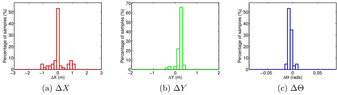
Figure 4.39: Relative Entropy optimisation: 2 iterations. Residual errors after 2 iterations of Algorithm 3 over: (a) X , (b) Y and (c) \Theta .
