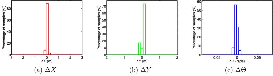
Figure 4.41: Relative Entropy optimisation: 4 iterations. The final residual errors, after 4 iterations of Algorithm 3 over: (a) X , (b) Y and (c) \Theta .
