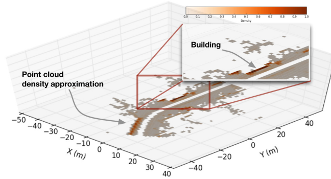
Figure 4.22: Histogrammed point cloud. The discrete approximation of the X, Y density of the projected point cloud shown in Figure 4.21. Highlighted by the inset image is the observed density of the building face – the higher densities of salient features (walls, buildings, etc.) is the aspect we exploit to enable large-scale, long-term localisation.
