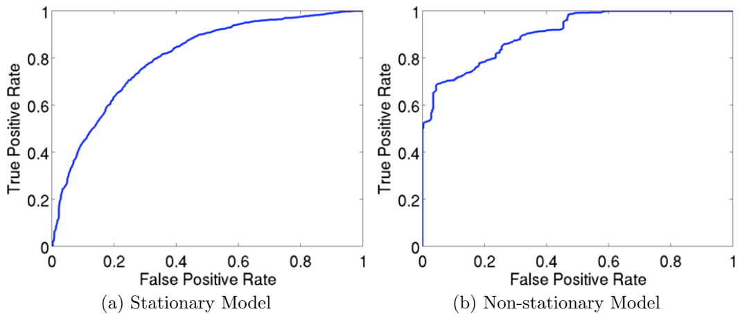
Figure 6.23: ROC curves. The Receiver Operating Characteristic (ROC) curves for (a) the stationary model, and (b) a single element of the non-stationary ensemble. A larger area under the ROC curve indicates a better classifier.
