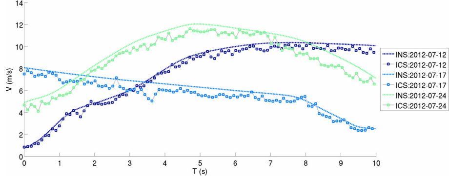
Figure 6.36: Velocity estimates: INS vs. ICS estimates (Woodstock main-road). Velocity estimates for the main road, leaving Woodstock. Again apparent in each of the datasets is the bias inherent in the ICS velocity feed due to traffic on the road. This effect is persistent enough to justify the effort to develop a scan filter that is able to correct this bias.
