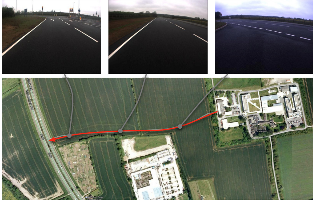
Figure 4.48: Featureless road section. A relatively featureless section near the Begbroke Science Park. The lack of informative structure in this region requires the use of the reflective properties of the LIDAR data.
