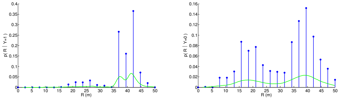
Figure 6.21: Non-stationary Model conditionals: range. Conditional distributions over range for the non-stationary sensor model at a particular \lambda value. Notice how the form of the distributions (particularly over range) has changed – this gives us an indication that conditioning on place will lead to better classification performance – compare this image to Figure 6.19. (Blue corresponds to the PMF from histogrammed counts, green to the kernel-density estimated PDF).
