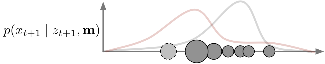
Figure 2.14: Particle Filter: Approximation. The new set of re-weighted particles now form the discrete approximation of the posterior distribution. The dashed circle represents a state-estimate added through external means, e.g. via GPS.
