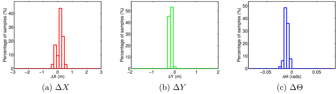
Figure 4.54: Mutual Information optimisation: Residual error. The residual error distribution at termination of the optimisation over (a) X , (b) Y , and (c) \Theta .
