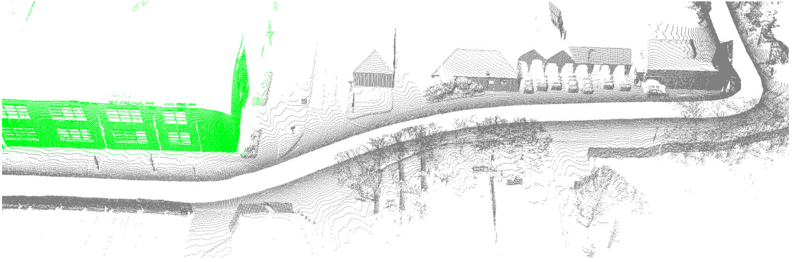
Figure 5.14: LIDAR data: Rain. The dataset corresponding to Figure 5.12(b). Note again that – although the road surface is different to both Figure 5.12(a) and Figure 5.12(b), the prismatic structure of the environment – buildings, walls – is unchanged.
