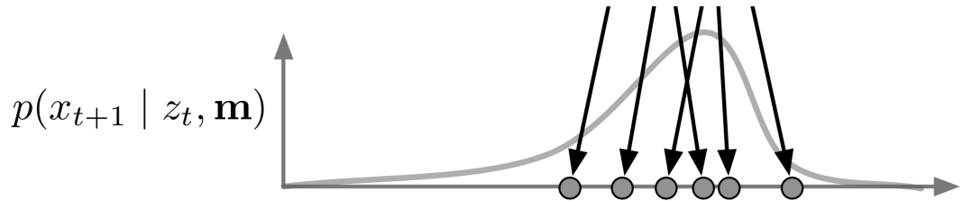
Figure 2.12: Particle Filter: Propagation. The set of propagated particles, using the motion model.
