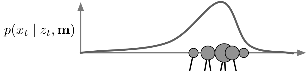
Figure 2.11: Particle Filter: Approximation. A weighted set of particles representing the underlying continuous probability distribution over pose.
