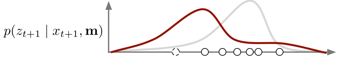
Figure 2.13: Particle Filter: Re-weighting through the measurement likelihood. Particle re-weighting through the observed data.
