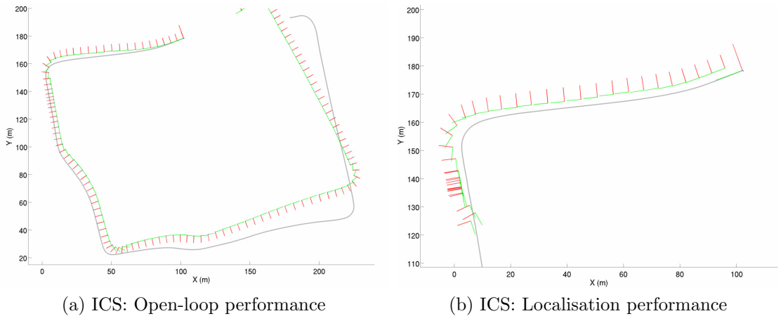
Figure 4.6: Scan-matching with a fixed-map over the long-term, 64 days later. Open-loop (a) and localisation (b) performance for the ICS matcher for a dataset taken 64 days after map acquisition. Notice the similar failure location to Figure 4.4(b).
