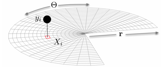
Figure 6.52: Discretized LIDAR model. A visualisation of the model used to estimate the transience of areas in the LIDAR scan plane (given a location in the world, indexed by \lambda ). The unobserved latent states, \mathbf{X} , constitute the underlying transience of a certain location in the beam plane of the LIDAR. The observed value \mathbf{y} are noisy estimates from training data, estimated by observing point misalignment in consecutive laser scans.
