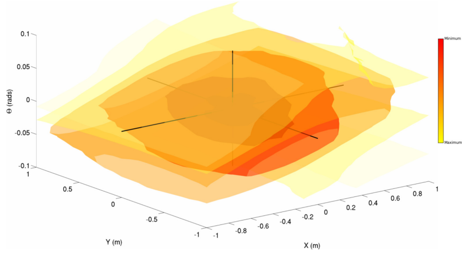
Figure 4.50: Localisation through reflectance matching. The objective function over SE2, using the mutual-information over the joint reflectances of the swathe and map.
