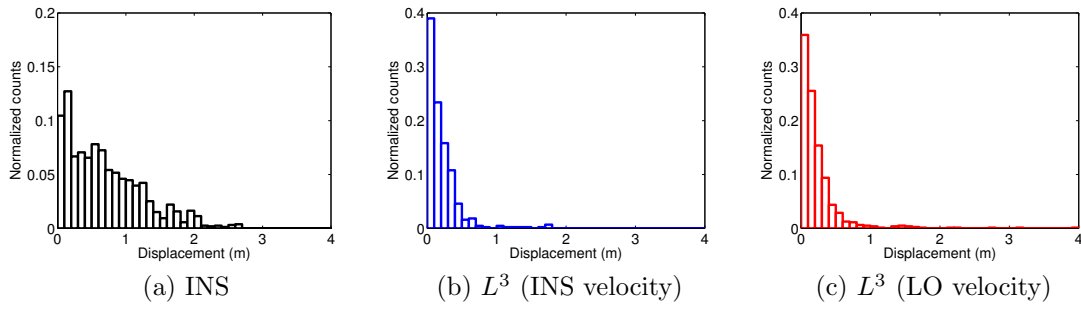
Figure 5.33: Relative displacement: L^3 (16/08/2012) . Histograms of the relative displacement for L^3 over the trajectories shown in Figure 5.32(a), showing (a) the INS performance, (b) L^3 with INS velocity, and (c) L^3 with LO velocity.
