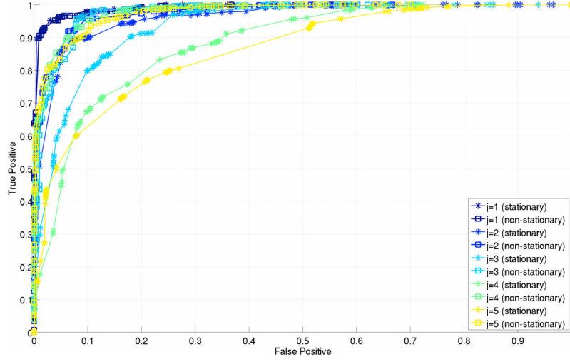
Figure 6.27: Bagged Decision Trees stationary vs. non-stationary ROC. Bagged decision tree ROC curves, for the same training instances shown in Figure 6.26. Decision-trees are a more discriminative classifier than Naive-Bayes, and this is reflected in the performance curves – although the non-stationary approach still dominates the stationary approach for all \mathcal{M} .
