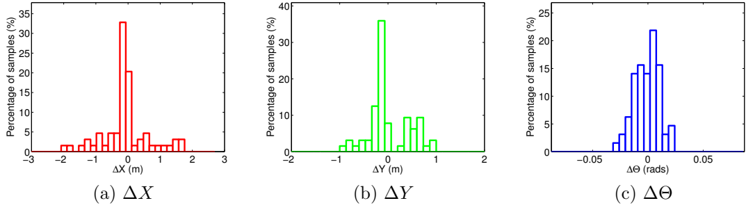
Figure 4.38: Relative Entropy optimisation: 1 iteration. Residual error after running Algorithm 3 for 1 iteration: (a) X , (b) Y , (c) \Theta .
