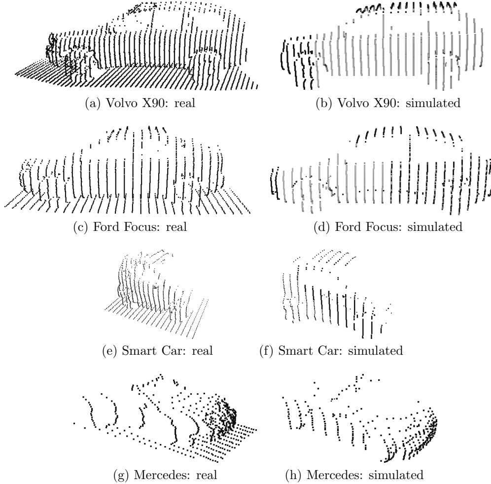
Figure 3.19: A comparison of LIDAR data. Real LIDAR data (left-column) compared against simulated LIDAR data (right-column) for the vehicles in Figure 3.18: (a) Volvo X90, (c) Ford Focus, (e) the Smart Car, and the (g) Mercedes.
