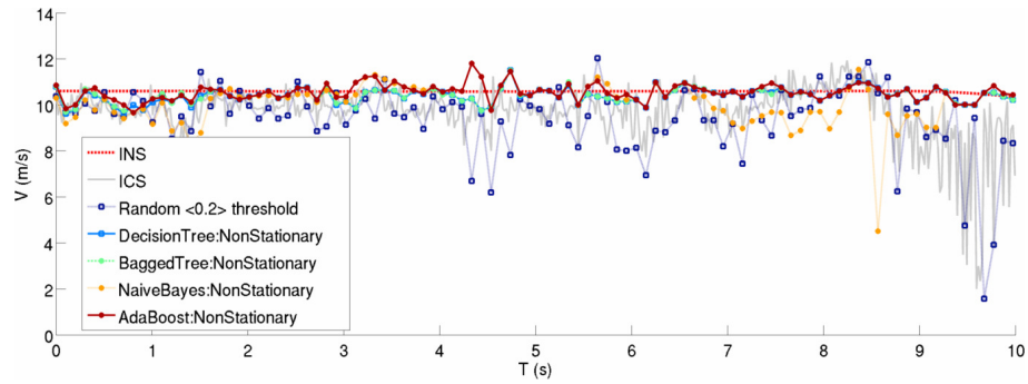
Figure 6.41: Filtered velocity estimates (Woodstock exit). Filtered velocity estimates using the various classification techniques over the Woodstock exit. In this example, the ICS velocity error due to traffic is highly visible. RMSE comparisons are shown in Table 6.7.
