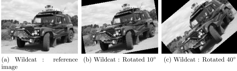
Figure 4.42: Using Mutual Information for alignment. Shown in (a) is a reference image, corrupted by varying degrees of rotation – (b) 10° and (c) 40°.
