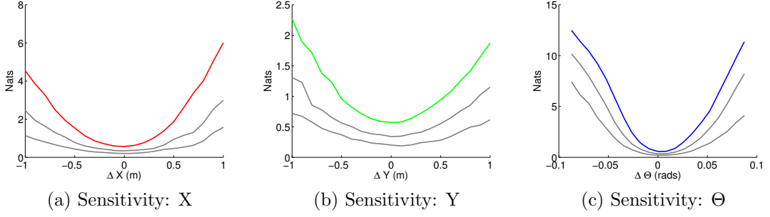
Figure 4.34: Relative Entropy sensitivity over SE2. An enumeration of the objective function along the cardinal axes of SE2 space: (a) X-axis, (b) Y-axis and \Theta -axis, (c).
