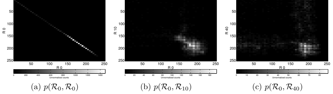
Figure 4.43: Estimating the joint distribution over intensity. The joint distribution over intensity, p(\mathcal{R}_0, \mathcal{R}_\alpha) , for the images shown in Figure 4.42. Note in (a) the strong diagonal, indicating exact alignment (this is expected, they are the same images). For increasing rotation, the distribution becomes more diffuse, with a correspondingly higher entropy, resulting in a lower mutual information. Note that the \alpha subscript corresponds to the rotations in Figure 4.42.
