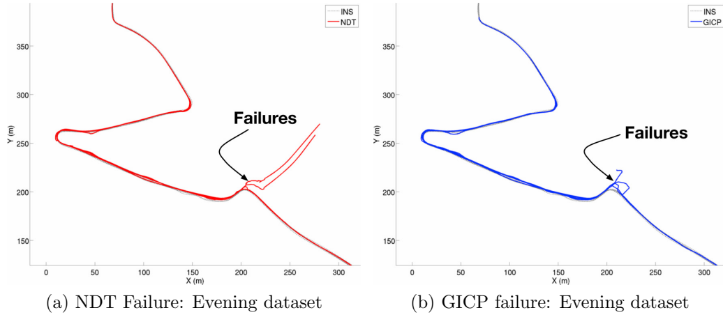
Figure 5.24: NDT/GICP failure cases. NDT (a) and GICP (b) have similar failure cases when using LO as a velocity source – slight velocity errors result in matching (and subsequently tracking) failure. This catastrophic failure is not suffered by L^3 . (These comparisons were made over the same data used by L^3 in Figure 5.19).
