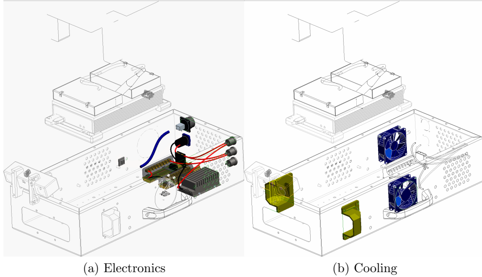
Figure 3.26: NABU: Power electronics and cooling units. The electronics shown in (a) provide the necessary voltage rails and power-regulation for the different sensor types. (b) shows the fans (blue) and air ducts (yellow) responsible for cooling the unit when stationary and moving, respectively.
