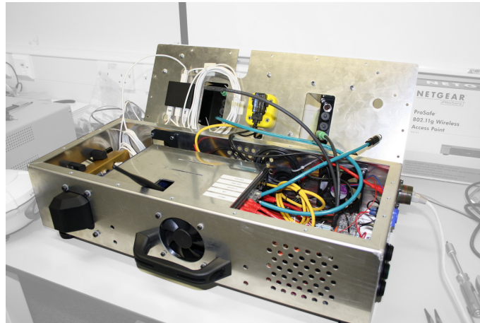
Figure 3.27: NABU: Construction. Visible in this image is the Bumblebee2 stereo camera from PointGrey (left side of the image), the MicroStrain IMU (top) and the air-scoops and fans for cooling.
