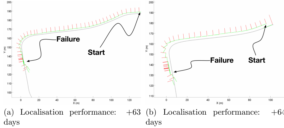
Figure 5.5: ICS localisation failures. The failures using a scan-matching approach with a static map from two months prior. These are the same figures as shown in Chapter 4, repeated here for continuity.
