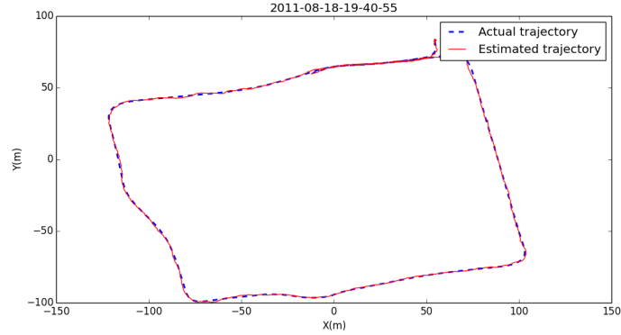
Figure 5.4: L3 results: Example 2. A similar experiment to Figure 5.3 using actual INS data around the Begbroke scene. Again, L3 provides a good estimate of the vehicle trajectory.
