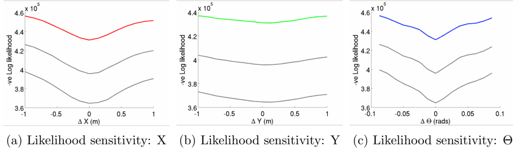
Figure 4.31: Likelihood sensitivity over SE2. An interrogation of the objective function (likelihood) along the cardinal axes of SE2 space: (a) X-axis, (b) Y-axis and (c) \Theta -axis, for various histogram granularities.
