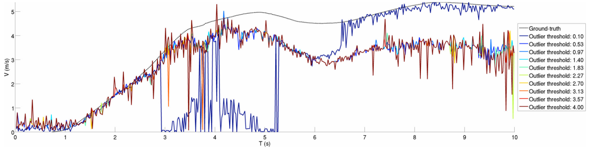
Figure 6.58: Comparison of ICP parameters in Woodstock centre. Velocity estimates arising from different outlier thresholds in an ICP scan-matching engine.
