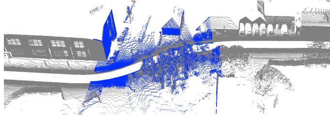
Figure 5.20: GICP: Good match. A successful match of a run-time point-cloud (blue) against a previously captured survey (grey). These point-clouds were generated using a 2D LIDAR and accurate pose estimates from a commercial INS. This location in Begbroke (along the western section) is used as a control point as there exists substantial planar-structure visible from the LIDAR, which is highly beneficial for point and plane-based registration algorithms.
