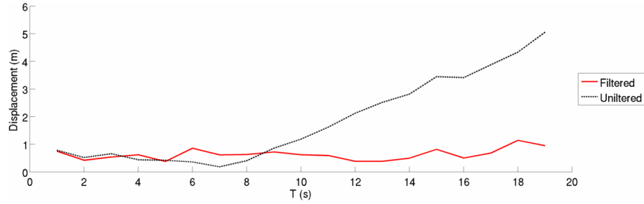
Figure 6.43: The effect of filtering on localisation. The difference in sequential pose estimates measured as a function of distance to the current INS pose estimate, using the non-stationary filter (red) and the unfiltered approach (black). Using the unfiltered velocity estimates, the estimate using L^3 begins to diverge until failure. However, by filtering the LIDAR points, the velocity estimate exhibits less error, maintaining localisation.
