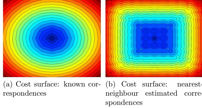
Figure 2.17: Cost surface: known vs. unknown correspondences. The difference in the cost-surface, comparing the squared-error of E(\mathcal{T}) with known (true) correspondences (a), and correspondences estimated with a nearest-neighbour approximation. (Dark-blue corresponds to the lowest cost, red to the highest)
