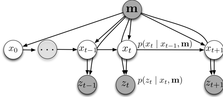
Figure 2.10: Bayesian Network. The posterior probability (represented as a graph) of the pose (and observation) chain of the robot as it moves through the environment. Observed quantities are shaded, unobserved – or latent quantities are not. Localisation consists of estimating the latent states x_{0:n} from the observed data z_{1:n} and the map, \mathbf{m} .
