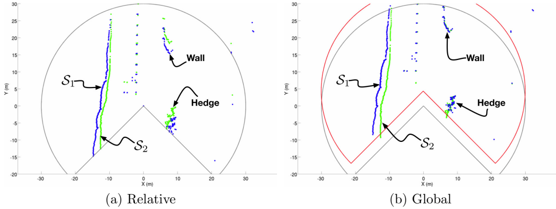
Figure 6.49: LIDAR point-overlay comparison. (a) A comparison of two 1-second separated LIDAR fans from the horizontally-mounted LIDAR, showing the point-comparison when projected into the same frame. Visible on the right-hand side are a wall and a roadside hedge. (b) The same fans, rendered into a global frame using the INS. The wall and hedge are now well aligned – however, the points on the left are not aligned, indicative of ground-strike.
