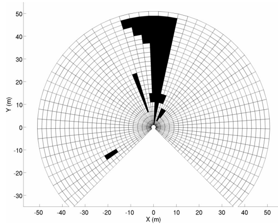
Figure 6.55: Iterated Conditional Modes (ICM) . The resulting locally maximal \mathbf{X} given by applying ICM to the observed data for the location \lambda'' shown in Figure 6.51 over the model depicted in Figure 6.52. Note how the road has been learned to be an unreliable place for scan-matching, given the presence of vehicles. Also, the entryway between two buildings has also been classified as transient – this is due to repeated induced roll experienced by the vehicle at that particular point.
