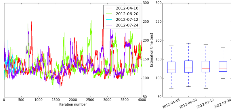
Figure 5.40: Particle Filter performance. The performance of a Sequential Importance Sampling (SIS) over portions of several L3 datasets. As can be seen, the performance of the estimator is consistent, if slow.
