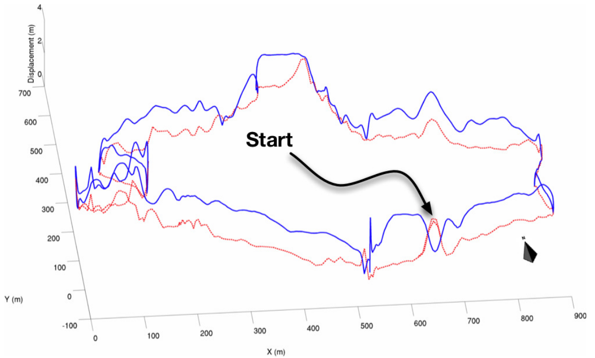
Figure 6.46: Average relative displacement. The relative displacement comparison of estimated trajectories from the INS (blue, solid) and the L^3 system (red, dashed) against a reference trajectory over 2.7km. As can be seen, the L^3 approach exhibits a lower displacement as compared to the INS over the course.
