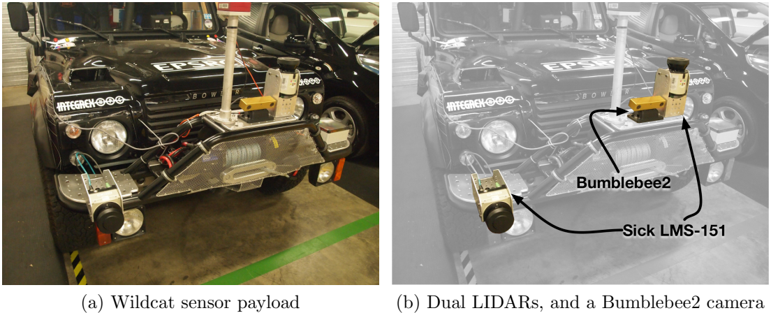
Figure 6.1: Wildcat sensor configuration. The dual-LIDAR setup on the Wildcat. Note the horizontally-oriented LIDAR adjacent to the Bumblebee camera, and the vertically-oriented LIDAR on the front bumper. The velocity estimates from the horizontal LIDAR and the range-data from the declined LIDAR allow us to build the run-time swathe, as discussed in Chapter 4.
