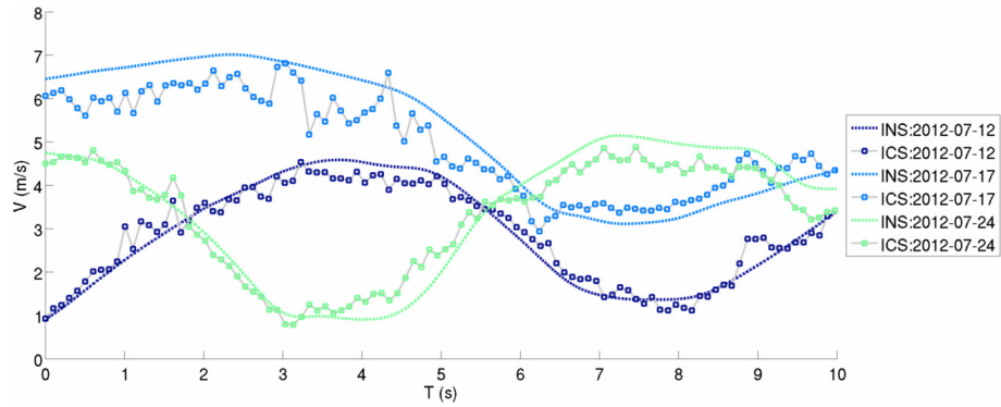
Figure 6.35: Velocity estimates: INS vs. ICS estimates (Woodstock centre). Velocity estimates for the same datasets as in Figure 6.34 in the centre of Woodstock, exhibiting similar behaviour. In some cases, on the 12 th of July for example, the ICS estimates are not unduly biased, due to the lack of traffic at this particular time.
