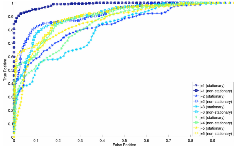
Figure 6.26: Naive-Bayes stationary vs. non-stationary ROC. Naive-Bayes ROC curves for different numbers of training instances – j corresponds to the index of one of the 48 model positions shown in Figure 6.17. As we increase the amount of data taken from different places in Figure 6.17, the performance of the stationary model begins to degrade – although this is also true for the non-stationary approach, the degradation is much less rapid.
