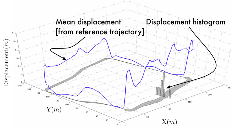
Figure 5.9: INS cumulative relative displacement over 26km. 26 kilometres of accumulated relative displacement data – using the INS – around the Begbroke site. By measuring the distance from any pose in a given trajectory to the closest pose (in an Euclidean sense) in a reference trajectory, we obtain this graph. Indicated are the mean ( z -axis) and standard deviation (shaded, grey) for the entire set, as well as an example histogram for a given point. This histogram is of displacements over multiple repeats over the same route. The degraded INS performance is highly visible in the northern and southern sections.
