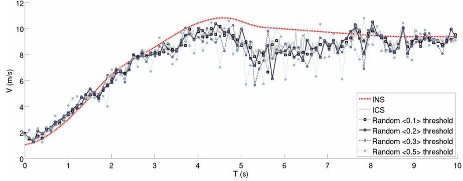
Figure 6.42: Filter comparisons : Randomized sub-sampling. Filtered ICS estimates using a random decimation of the incoming points. This naive approach merely increases the signal-to-noise ratio, and does little to compensate for the accrued velocity bias.
