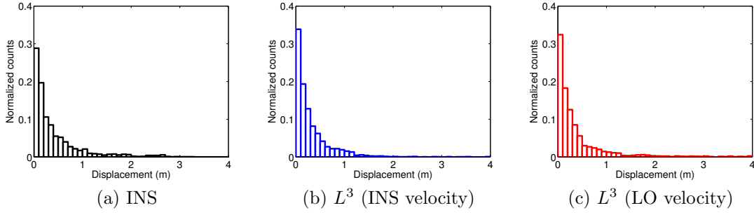
Figure 5.29: Relative displacement: L^3 (23/08/2012) . Histograms of the relative displacement using a DGPS base station, showing (a) the INS performance, (b) L^3 with INS velocity, and (c) L^3 with LO velocity. Notice the substantially improved INS estimate.
