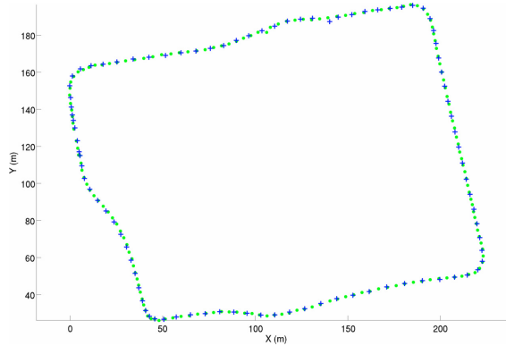
Figure 5.6: L^3 vs. ICS over 1.5km (and 2 months). The same run-time data – as used in Figure 5.5 – with the same map, captured two months prior. This figure shows that the localisation performance of L^3 – which is explicitly leveraging the persistent 3D structure of the environment – is superior to that of scan-matching. (Note: Trajectory estimates have been down-sampled and plotted as points for easier visible differentiation.)
