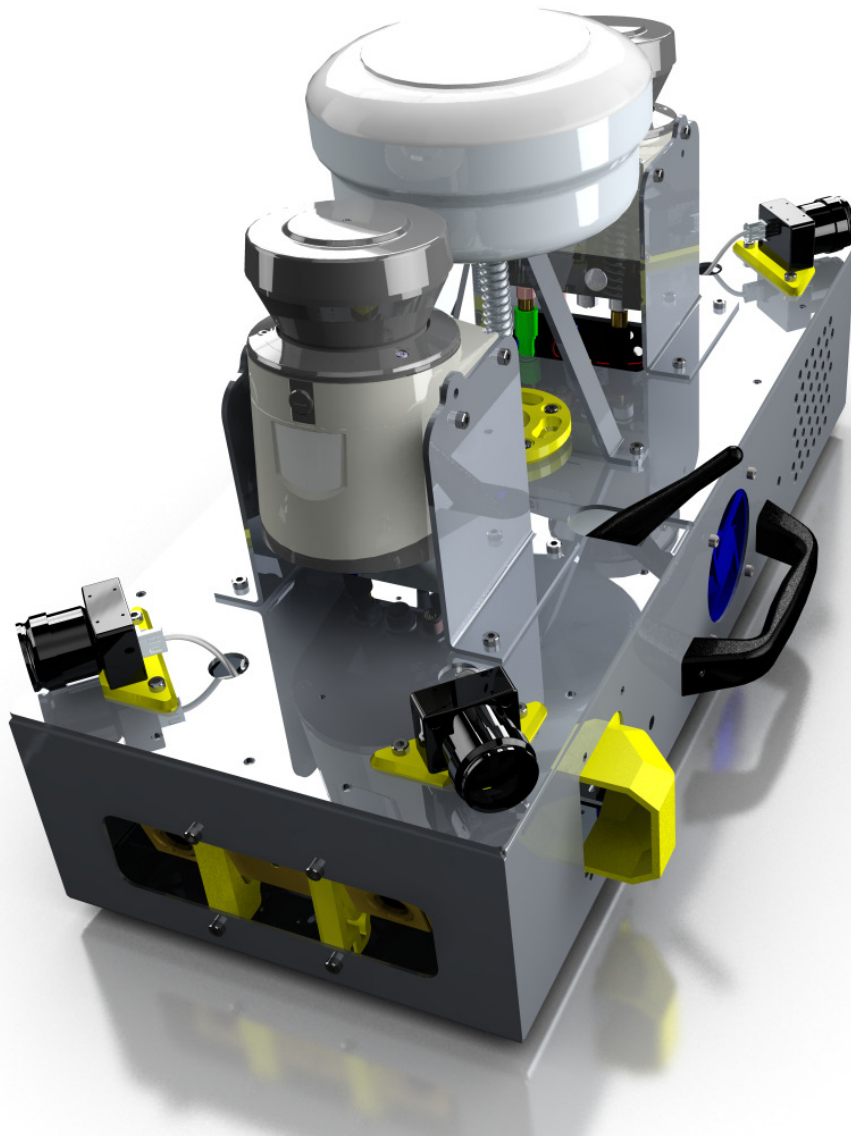
Figure 3.20: NABU: CAD rendering. A CAD of the NABU. The NABU is a vehicle-agnostic stand-alone sensor suite that is designed to be used for mapping and/or localisation tasks.
