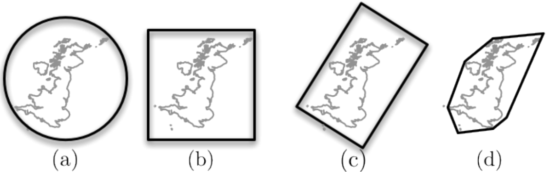
Figure 3.7: Bounding volume construction. Different ways of generating bounding volumes for arbitrary geometry: (a) spherical, (b) axis-aligned bounding box, (c) oriented bounding box, and (d) convex-hull. The more complex the bounding volume (i.e. the more representative of the underlying geometry), the fewer high-level queries have to be performed, at a cost of significant increases in memory requirements.
