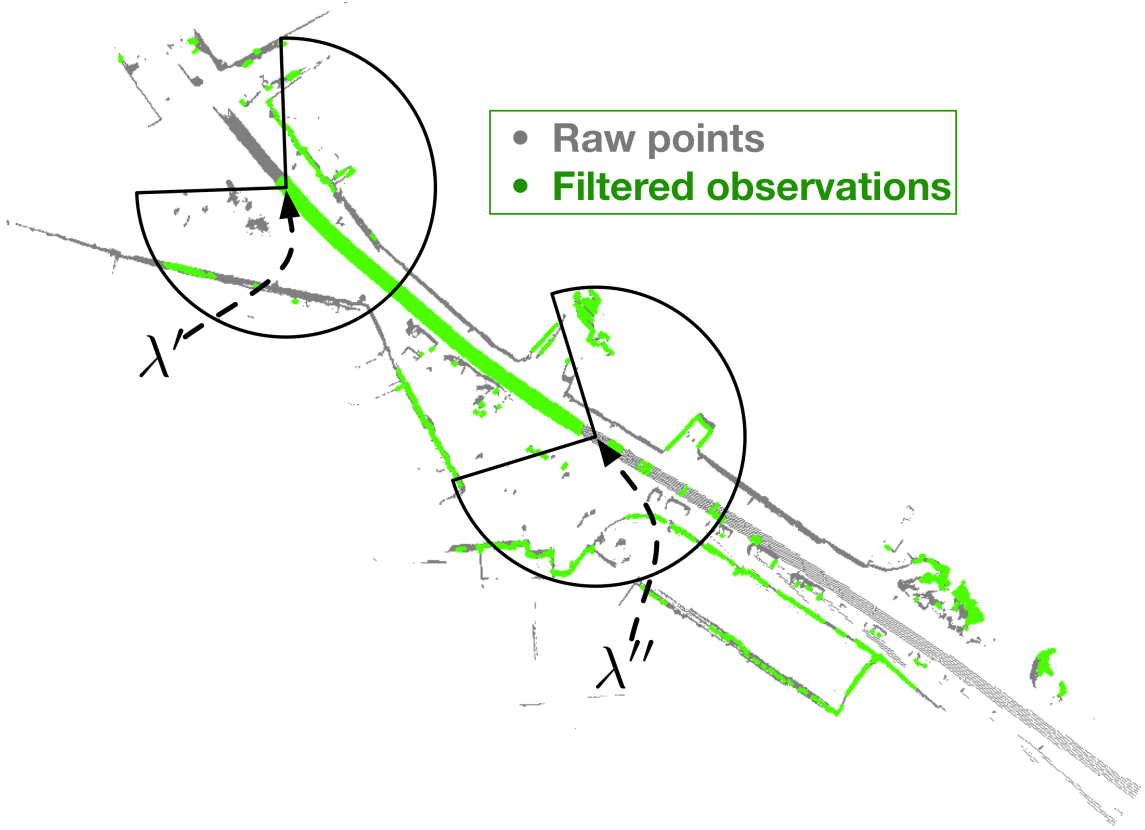
Figure 6.51: Woodstock LIDAR transiency illustration: Transient observations. The filtered LIDAR points from Figure 6.50, filtered as per Algorithm 8. By fusing INS and LIDAR data during the initial run and applying simple clustering methods, we can isolate areas in the environment that exhibit a high degree of transience. In addition to vehicles, ground strike (top-right) is also detected – this is to be expected, as ground-strike can be characterized as a fast-moving wavefront. Some static structures are incorrectly observed as transients – however, the number of these observations is small. Also shown are two example LIDAR fans rendered at two successive \lambda positions.
