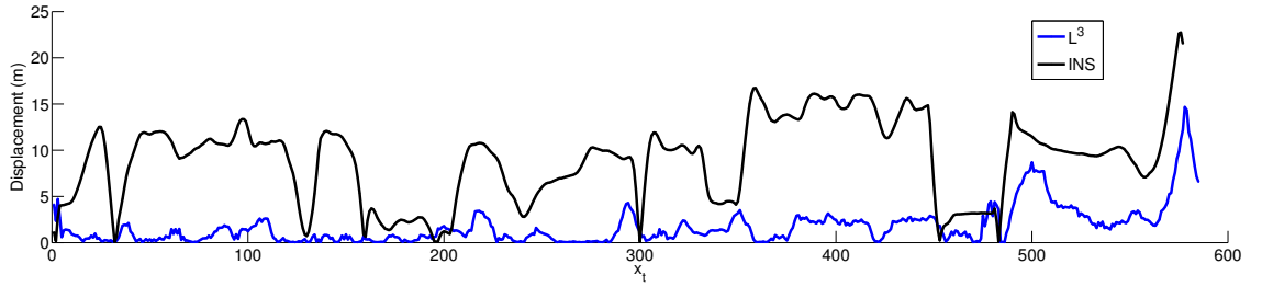
Figure 5.36: Displacement comparison around Woodstock: INS vs L^3 . The displacement comparison for the trajectories shown in Figure 5.35, showing the larger averaged displacement of the INS to the reference trajectory.
