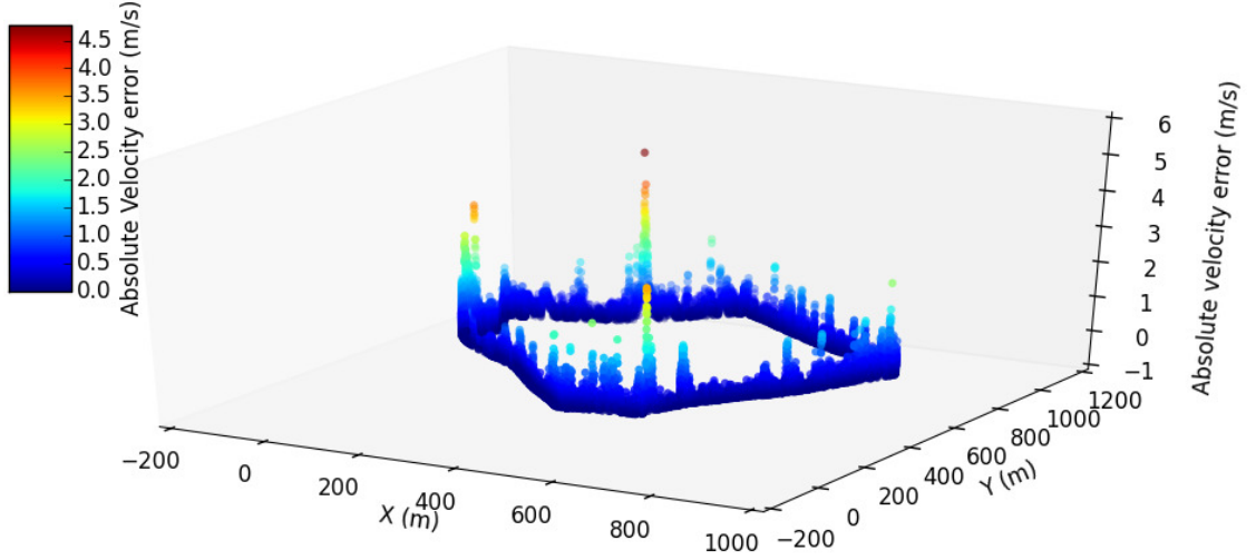
Figure 6.6: Velocity error: Kidlington. A similar plot to Figure 6.5 around Kidlington, Oxfordshire. Again we see the presence of ground strike and traffic inducing error in the velocity estimates (highlighted in the north-east and west, respectively).
