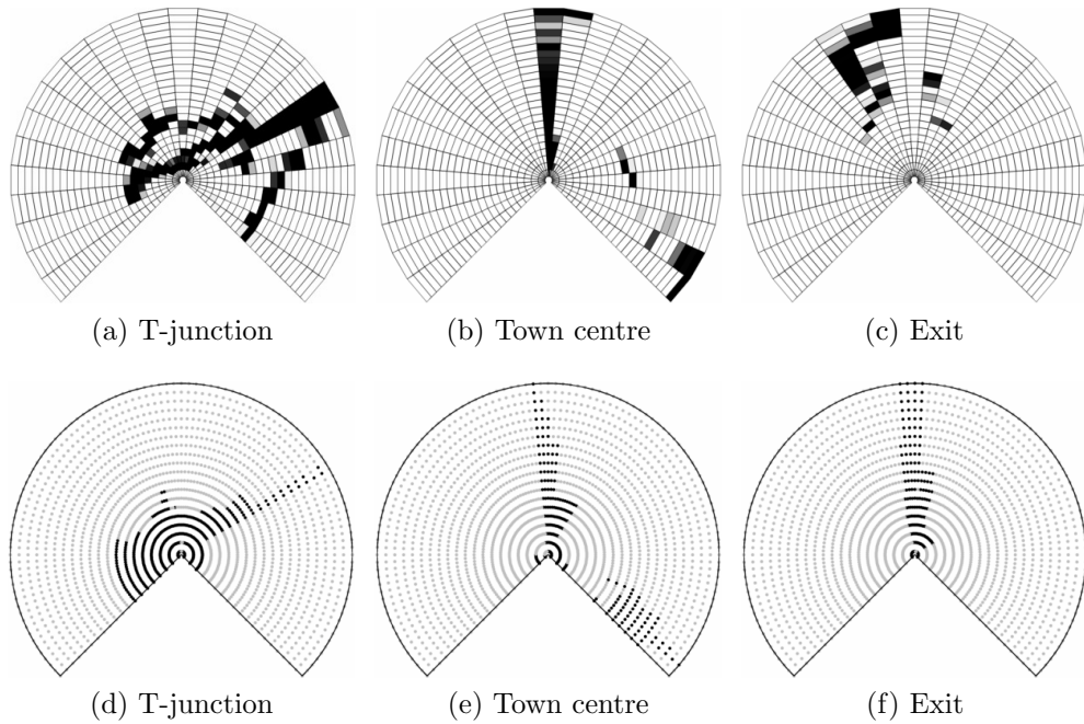
Figure 6.56: Comparison of supervised/unsupervised filters. Top row is the transiency-based estimation over the LIDAR model, bottom-row is the fully-enumerated decision boundary for the equivalent non-stationary supervised classifier at the same location (Decision Trees, in this example). (a)(d) are the Woodstock T-junction, (b)(e) the town centre, and (c)(f) the Woodstock exit.
