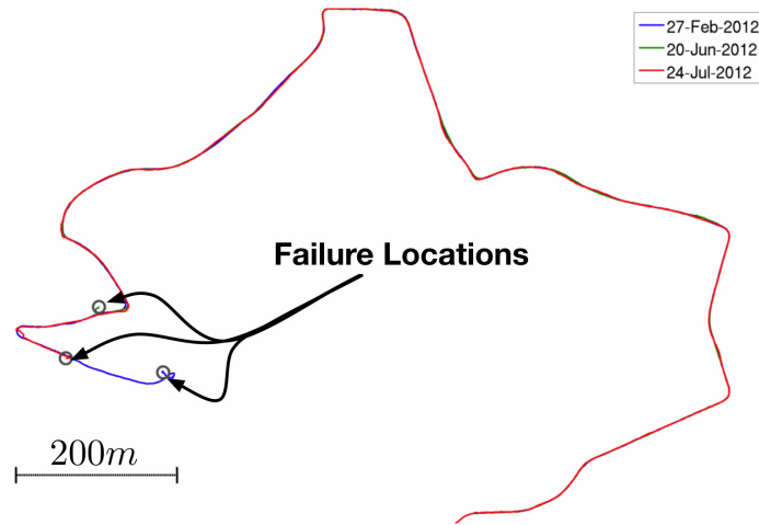
Figure 6.44: Woodstock failure locations. Localisation points-of-failure over the Woodstock route over three datasets spanning several months. Note how the failure locations cluster in the town centre – typically due to the presence of traffic.
