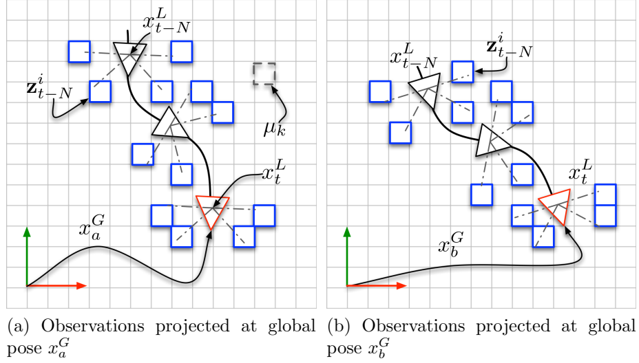
Figure 4.23: Observations as a function of pose. Figure (a) shows the distribution of pseudo-observations \mathbf{z} at global pose x_a^G , with rigid relative pose-chain \mathbf{x}_{t-N:t}^L obtained from the linear and rotational velocity estimates, while figure (b) shows the distribution of the same observations and pose-chain, at a different global-pose x_b^G (Blue-squares represent observations, triangles represent poses). LIDAR readings \mathcal{Z}_t are projected, using calibration parameters and the estimated transform, into world-coordinates and then subsequently projected onto the XY plane to give the pseudo-observations, \mathbf{z} . The divergence between the histogrammed approximation of these measurements and the histogrammed approximation of the prior point-cloud is then minimized as a function of x , y , and \theta to give an estimate of the current pose.
