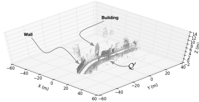
Figure 4.20: Raw point cloud. This figure shows a point cloud as obtained from the declined 2D LIDAR. Visible are various aspects of a scene, including a low wall and the front of a building.
