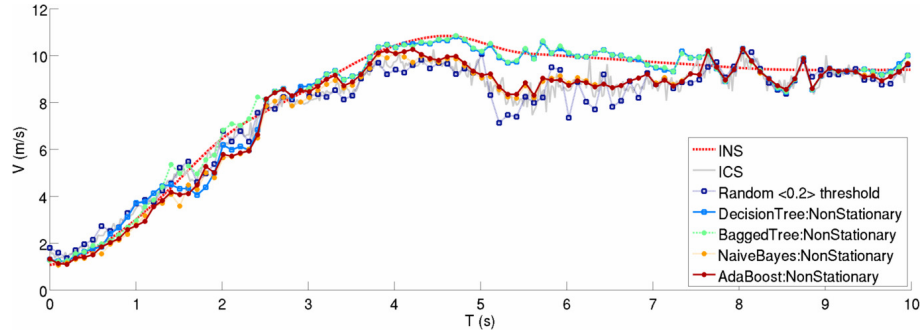
Figure 6.40: Filtered velocity estimates (Woodstock T-junction) . Filtered velocity estimates using the various classification techniques over the Woodstock T-junction. RMSE comparisons are shown in Table 6.6.
