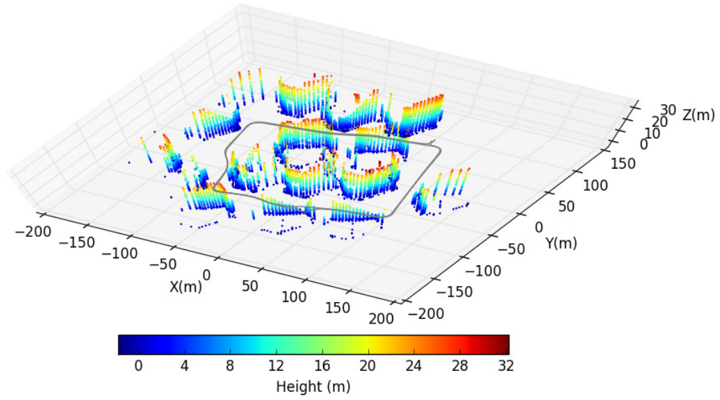
Figure 5.2: Synthetic Begbroke experience. The point cloud used as the experience cloud, for the scene shown in Figure 5.1. Visible are the LIDAR points (false-coloured by height) as well as the trajectory used to generate these points.
