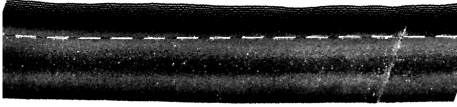
Figure 4.49: Road reflectance from the declined 2D LIDAR. Road reflectance from the 2D LIDAR over the area shown in Figure 4.48. Clearly visible are the lane dividers.
