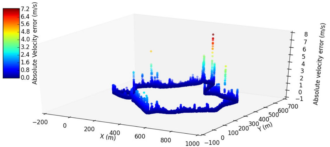
Figure 6.5: Velocity error: Woodstock. A plot of the absolute error in linear velocity from the scan-matching algorithm over the course of the Woodstock run, as compared to the INS on the vehicle. In some locations, the error is in excess of 7m/s . Typical causes of these errors are illustrated in Figure 6.7 through Figure 6.9.
