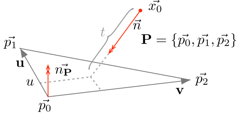
Figure 3.5: Ray/triangle intersection using barycentric co-ordinates. The barycentric co-ordinates (u, v) are a weighted sum of the polygon vertices \mathbf{P} , and have natural constraints when considering the putative intersection of ray x(t) .
