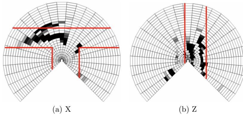
Figure 6.57: Kidlington: Unsupervised filters. Unsupervised filters learned for a (a) T-Junction, and (b) straight road section.
