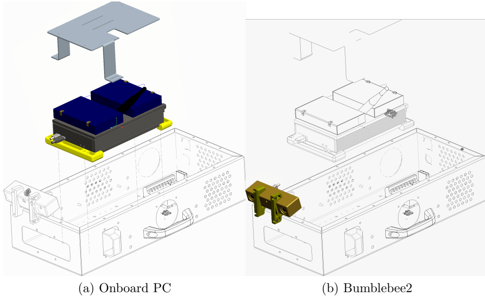
Figure 3.25: NABU: On-board PC and Bumblebee2 camera. Shown in (a) is the combined PC/Networking stack, consisting of a fan-less low-power PC, a router, and a wireless access point (WAP). (b) is a Point Grey Bumblebee2 stereo camera.
