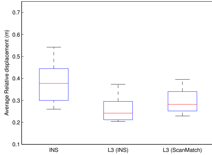
Figure 5.34: Average relative displacement over 50 kilometres. A plot showing the average relative displacement – the average displacement to a reference trajectory, averaged over more than 50km of trajectory data. This is shown for the INS (left), the L^3 approach with INS velocity estimates (centre), and (right) L^3 with LO velocity estimates.
