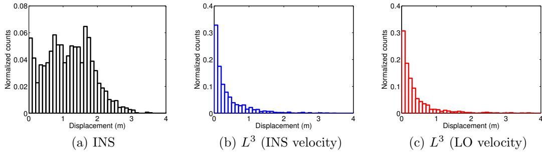
Figure 5.26: Relative displacement: L^3 (16/04/2012). Histograms of the relative displacement of the INS (a) against: (b) L^3 with INS velocity, and (c) L^3 with LO velocity.
