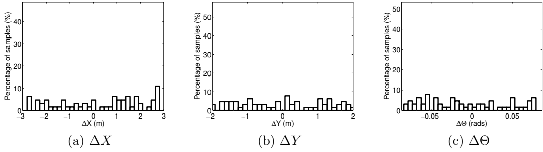
Figure 4.53: Mutual Information optimisation: Initial pose distribution. The initial distribution over starting pose for the purposes of interrogating the MI cost function. Figure (a) is the distribution over X , (b) over Y , and (c) over \Theta .
