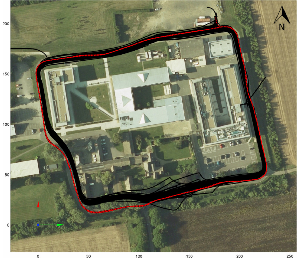
Figure 4.2: 26 kilometres of trajectory data around the Begbroke Science Park. A substantial dataset comprising of 3 months of INS data (26km total distance) around the Begbroke site in Oxford, contrasting areas of good GPS reception with poorer areas (the latter are predominantly in the northern and southern sections). As can be seen in the lower section of the image, the trajectories exhibit a large variation, caused mainly by GPS signal degeneracy due to foliage. The majority of the trajectories (black, solid) are counter-clockwise, with a single clockwise loop (red, dotted).
