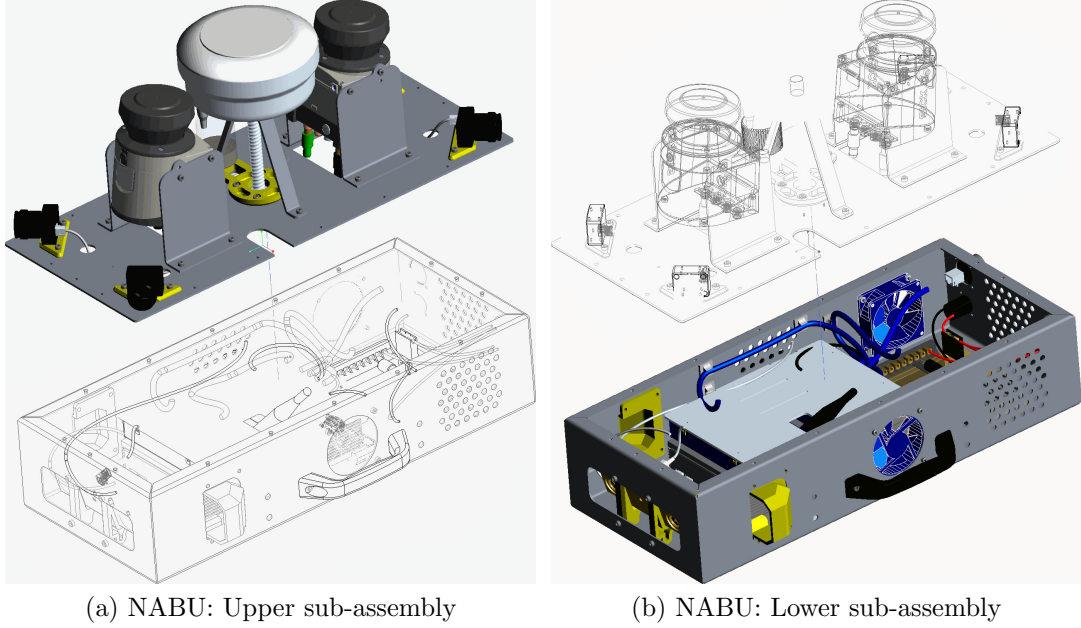
Figure 3.22: NABU: Sub-assemblies. The two major sub-assemblies of the NABU. (a) Shows the upper sub-assembly (shaded) which contains the majority of the sensors, while (b) is the lower sub-assembly (shaded), which contains the computing and power-management components.
