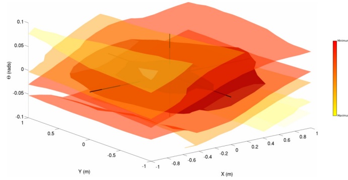
Figure 4.30: Histogram granularity: high. An objective function evaluation around a ground-truth registration, similar to Figure 4.28 with a high granularity.
