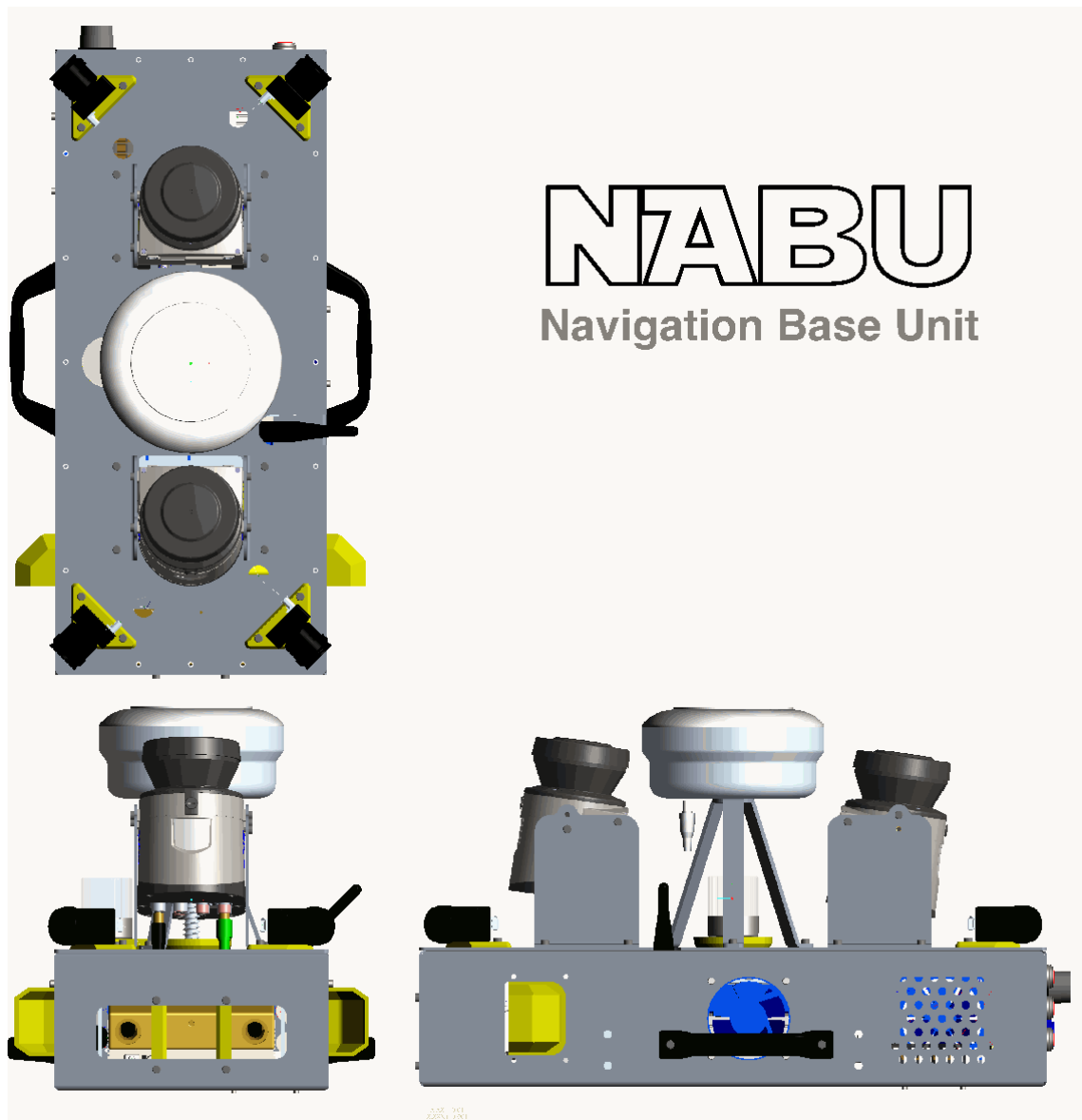
Figure 3.21: NABU: Top, front and right-side views. The top, front, and right views of the NABU. The unit was designed to be easily handled and mounted, and to allow for simple sensor re-configuration.
