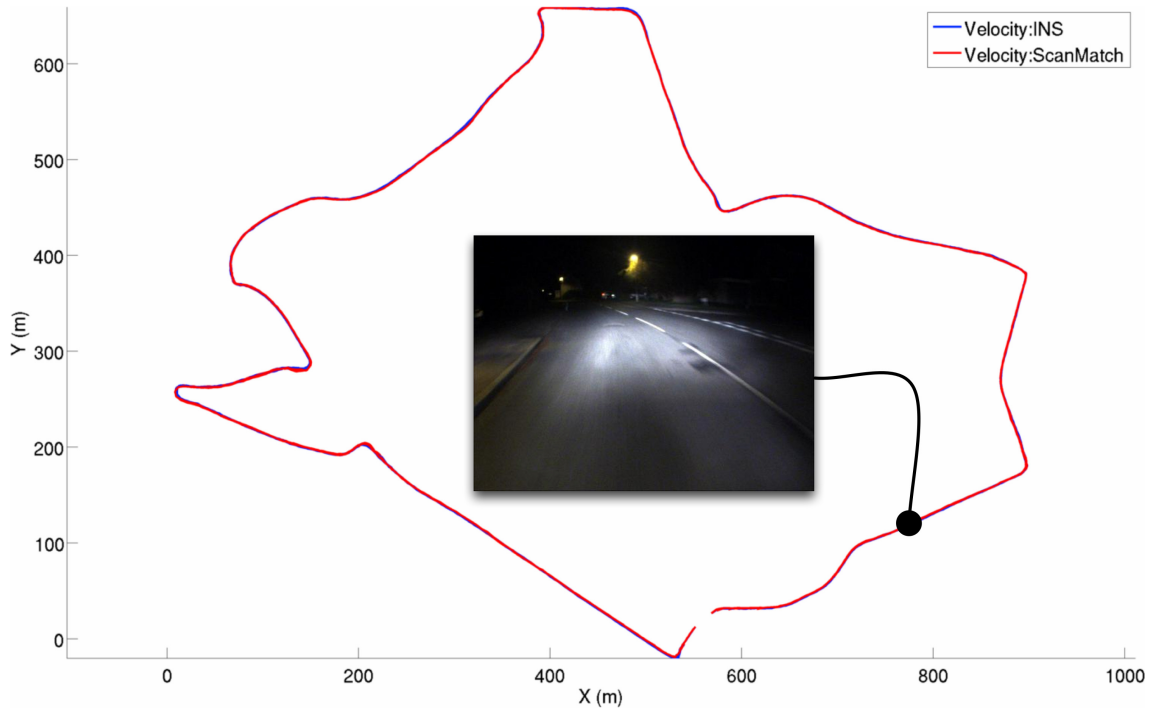
Figure 5.19: Woodstock evening results. An overview of the Woodstock evening dataset trajectory estimates. Two velocity sources are used: (1) INS velocity estimates as a control (blue), LO estimates (red). As can be seen from the figure, they are indistinguishable. Also shown is an example image from the forward-facing stereo camera – this is a testing situation for VO.
