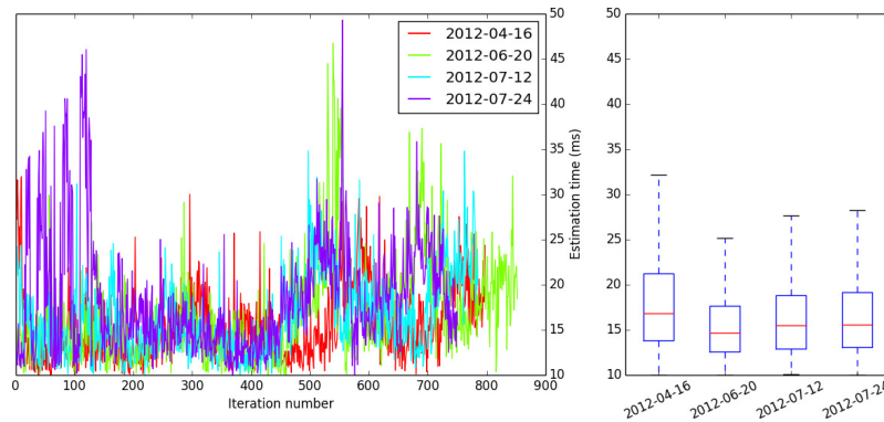
Figure 5.41: UKF Performance. Performance of the UKF over the same data in Figure 5.40. The average response time is approximately 15ms, corresponding to approximately 66Hz.
