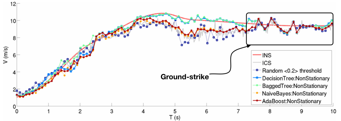
Figure 6.48: Velocity errors induced from ground-strike. The velocity error arising from ground-strike in the LIDAR fan. Although the decision tree and bagged decision tree models have reduced the signal-to-noise ratio by filtering out the traffic, both incorporate points corresponding to ground-strike, leading to velocity error.
