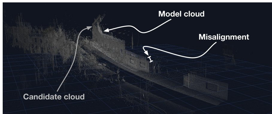
Figure 4.35: Unaligned registration scenario. A scenario, using real-world data, used to test the convergence properties of the registration algorithm. This figure shows two unregistered point clouds, as can be seen from the visible ghosting.
