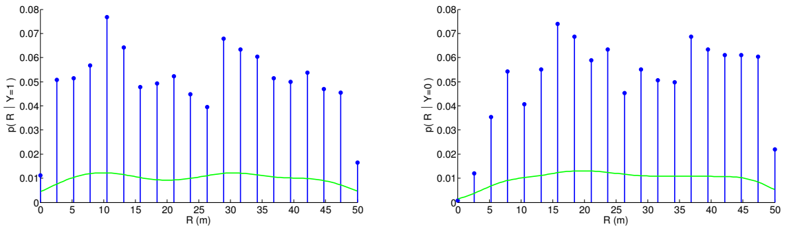
Figure 6.19: Stationary model conditionals: range. Conditional distributions for the stationary sensor model over range for both classes. Note how the range measurements are very uniformly distributed for both classes – this makes classification difficult. (Blue corresponds to the PMF from histogrammed counts, green to the kernel-density estimated PDF).
