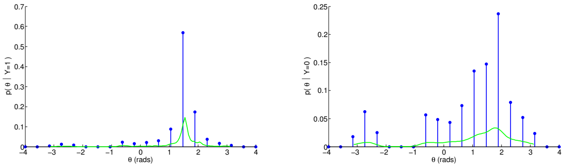
Figure 6.20: Stationary model conditionals: angle. A similar graph to Figure 6.19 over angle. For the data collected, vehicles tend to occur at \theta \in (0, 2) rads, which corresponds to the front and right-hand side of the vehicle. (Blue corresponds to the PMF from histogrammed counts, green to the kernel-density estimated PDF).
