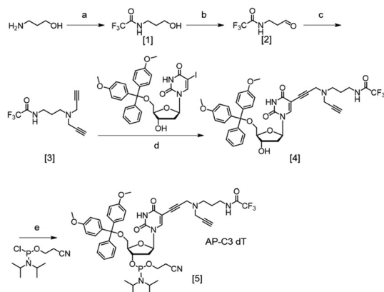
Fig. 2 Synthesis of AP-C3 dT phosphoramidite (5). Reagents and conditions: (a) neat ethyl trifluoroacetate, 3 h, 0 °C to RT, 97%; (b) CH 2 Cl 2 , Dess–Martin periodinane, 2 h, 0 °C to RT, 51%; (c) CH 2 Cl 2 , dipropargylamine, NaBH(OAc) 3 , 2 h, RT, 95%; (d) N,N -dimethylformamide, compound 3, PdCl 2 (PPh 3 ) 2 , CuI, triethylamine, 12 h, RT, 59%; (e) CH 2 Cl 2 , 2-cyanoethyl N,N -diisopropylchlorophosphoramidite, N,N -diisopropylethylamine, 1.5 h, RT, 72%.
