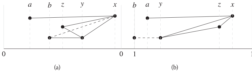
Figure 7: We show in (a) how to create a bull when the edge bx is removed and we show in (b) how to create a bull when by is added.
