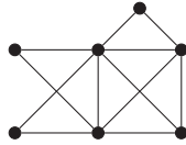
Figure 11: The final graph F_{\mathcal{Q} \sim w} .
