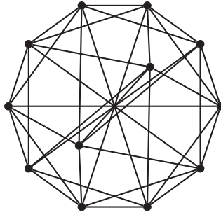
Figure 1: The complement of the icosahedral graph is induced-saturated for P_5 .
