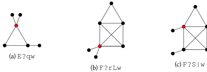
Figure 9: The three problematic graphs which we handle using the rational geometric graph. The vertices highlighted in red have neighborhoods which cannot be split into two cliques.
