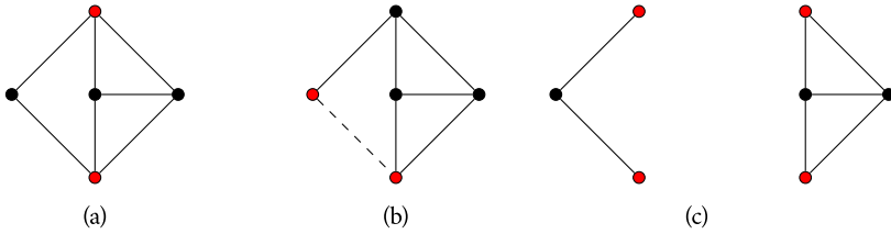
Figure 8: (a) The graph \text{Dr}[\ ] with its only 2-cut highlighted in red. There are no 2-cuts which are edges, so every non-edge is a gatekeeper. (b) The graph with the edge xy removed, with x and y highlighted in red. (c) The two fragments of the graph created by taking the components of the only 2-cut and adding back in the 2-cut. Observe that there is no copy of either of the fragments in (b) with matching vertex colors, which means that xy is a gatekeeper.
