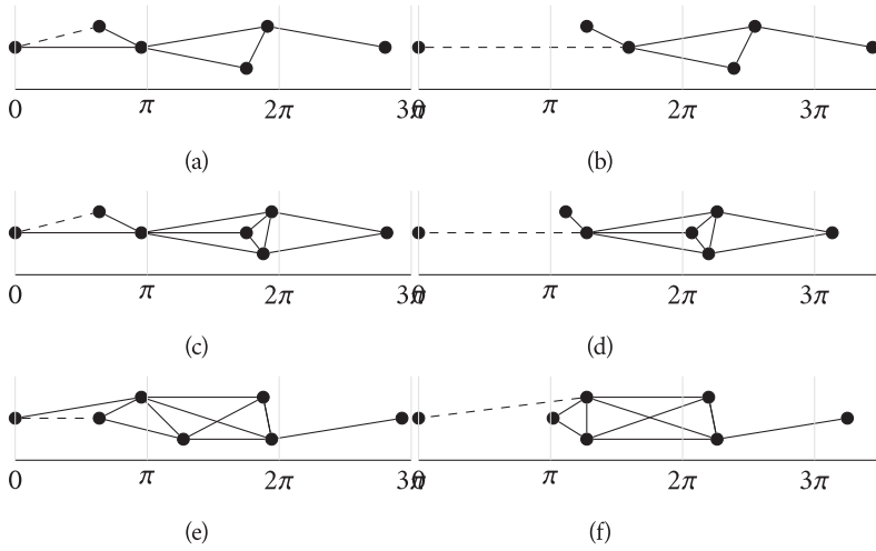
Figure 10: The left-hand side shows the constructions when removing an edge on the dotted line and the right-hand side shows the constructions when adding the edge indicated by the dotted line.
