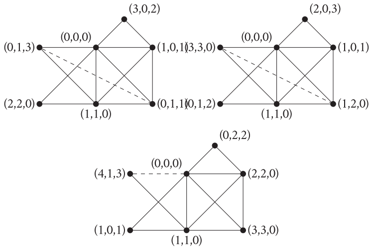
Figure 12: Examples of how to embed H into a copy of G when an edge of G has been perturbed. The dotted lines represent the location of the edge which was removed (top) or added (bottom).
