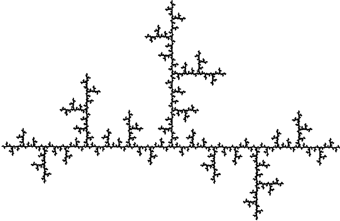
Figure 1.1: P.c.f.s.s. dendrite with |V^0| = 2 .
