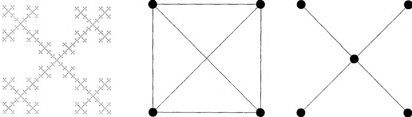
Figure 1.3: Vicsek set, (V^0, E^0) and (\tilde{V}^0, \tilde{E}^0) .
