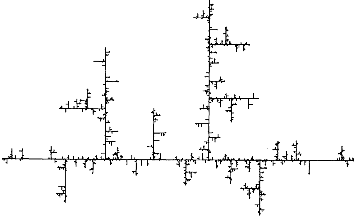
Figure 1.2: Random p.c.f.s.s. dendrite.
