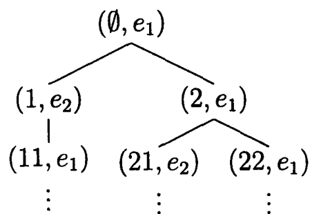
Figure 1.6: Hata family tree.
