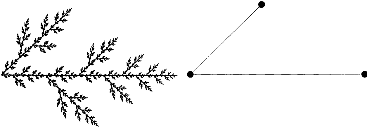
Figure 1.5: Hata's tree-like set and (\tilde{V}^0, \tilde{E}^0) .
