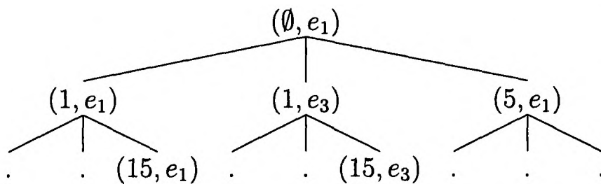
Figure 1.4: Vicsek set family tree.
