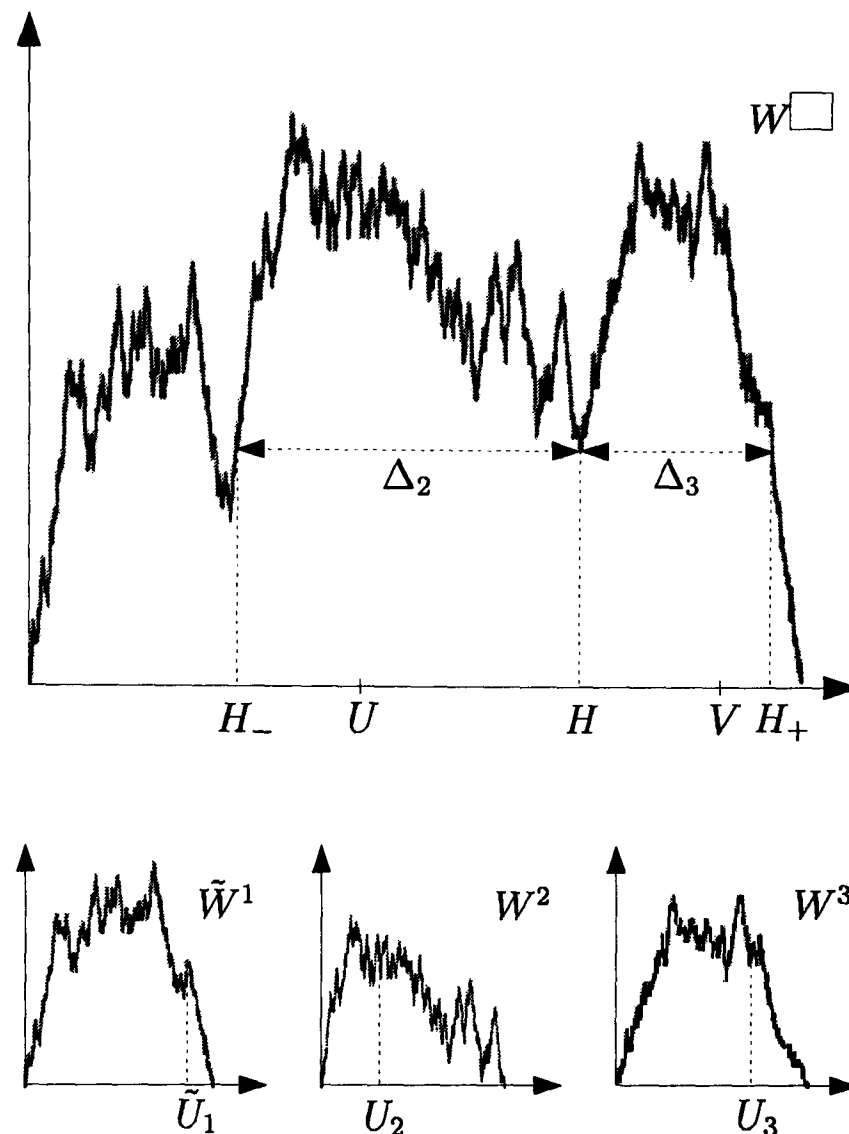
Figure A.1: Brownian excursion decomposition.
