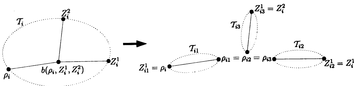
Figure A.2: Continuum random tree decomposition.
