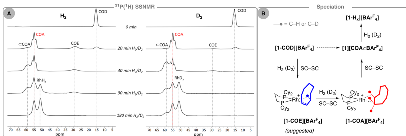
Figure 1. (A) Evolution of the products from the addition of H 2 or D 2 to crystalline [1-COD][BAR F 4 ] (1.5 bar, 293 K), measured by 31 P{ 1 H} SSNMR spectroscopy (10 kHz spin rate, 273 K). Dotted lines to guide the eye. (B) Solid-state speciation.
