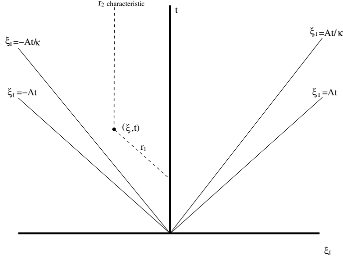
FIGURE 4.1. Sketch of the r_1 and r_2 characteristics emanating from the point (\xi, t) , shown in the t vs. \xi_I plane (where \xi = \xi_R + i\xi_I and \xi_R is fixed). The wide-angle wedge depicts the domain of analyticity of s(\xi, t) , w^s(\xi, t) , while the narrower wedge shows the domain of analyticity of r(\xi, t) , w^r(\xi, t) .
