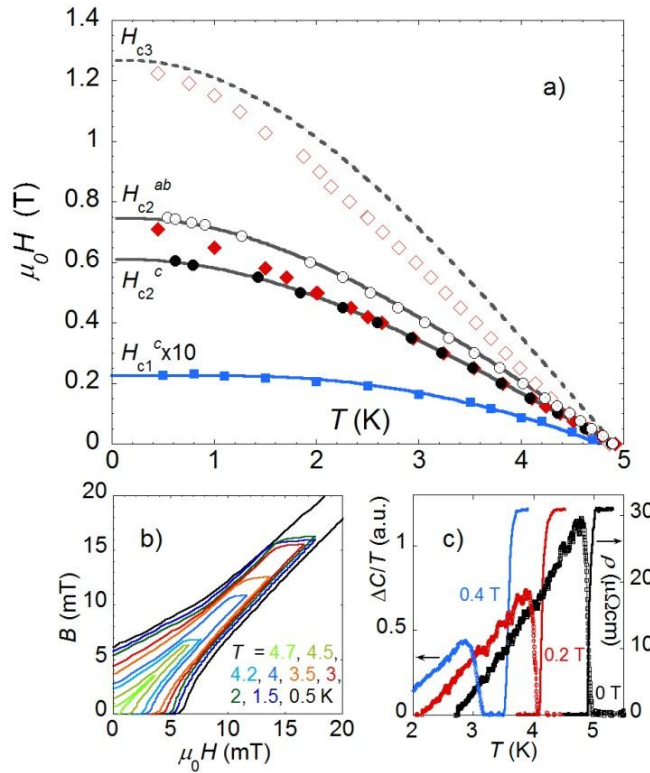
Fig.4 a) The phase diagram of \beta -Bi 2 Pd showing H_{c1}^c (blue squares, the data are multiplied by factor 10 to be in scale) with the best fit (blue line) to Eq. 2 corresponding to 2\Delta/k_B T_c = 4.1 ; H_{c2} from heat capacity (circles) and resistivity (lozenges) for both H||c (filled symbols) and H||ab (open symbols) together with the WHH theoretical curves (grey full lines) as well as a H_{c3} line (grey dashed line). b) Local magnetic induction B as a function of applied field H measured by a Hall-probe at selected temperatures, with the field first increasing and then decreasing back to zero. c) Superconducting transitions for H||ab revealed by the heat capacity (left axis) and resistivity measurements (right axis) at magnetic fields 0, 0.2 and 0.4 T, respectively.
