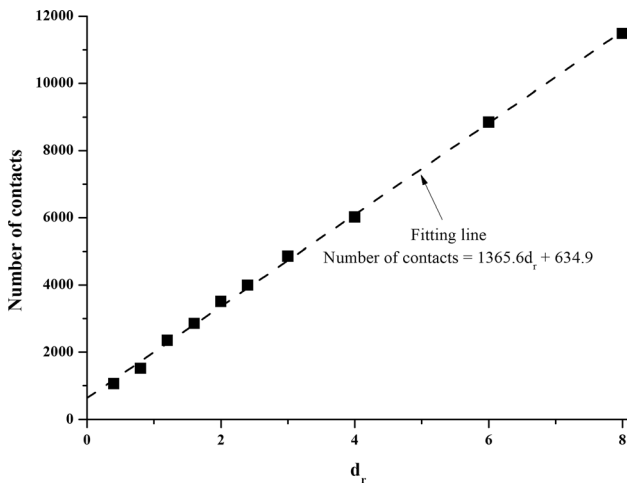
Fig. 16 Number of contacts on the sinker root at 0.4 mm (model scale) upward displacement (~ peak uplift force)
