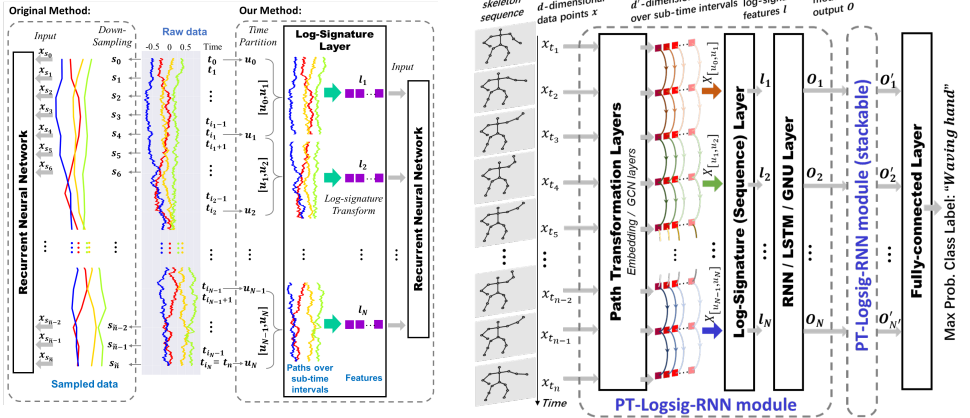
Figure 1: (Left) Comparison of Logsig-RNN and RNN; (Right) Pipeline of the PT-Logsig-RNN module for skeleton-based human action recognition. This stackable module consists of Path Transformation Layers, followed by the Log-Signature Layer and an RNN-type layer.
