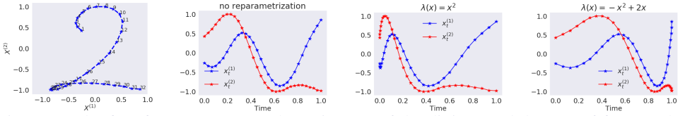
Figure 2: The first figure represents the trajectory of the digit 2, and the rest of figures plot the coordinates of the pen locations against time via different speed respectively, which share the same signature and log signature given in the first subplot.
